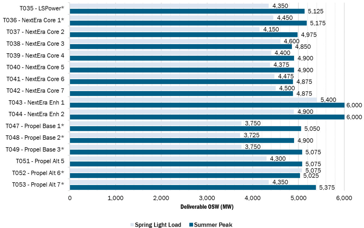
Figure 8: Electrical Expandability
