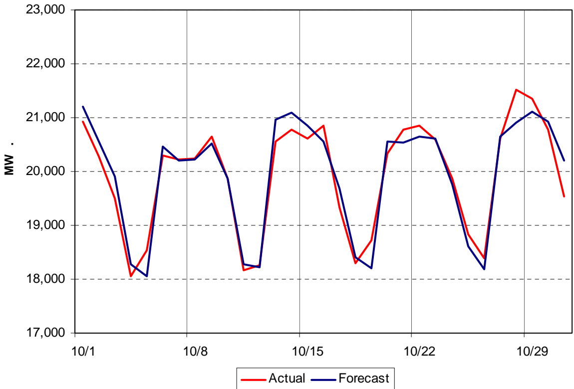
NYISO Daily Peak Load - October 2008 Actual vs Forecast
