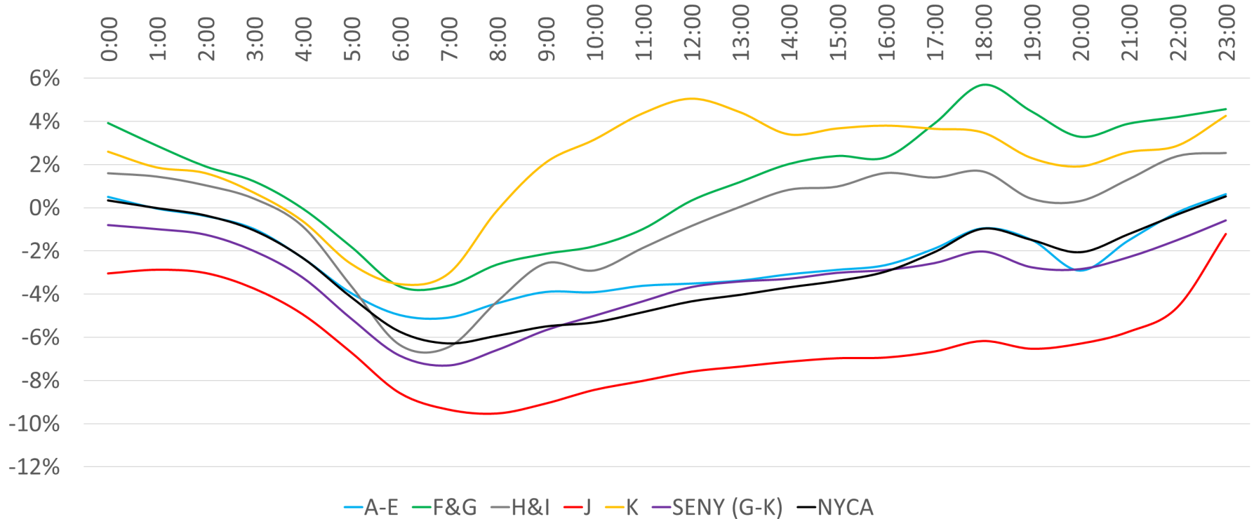
Average Hourly Deficit by Area - Week of 8/17- 8/21 (Weekdays)
