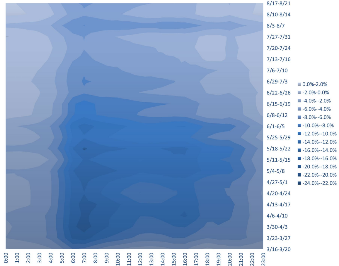
NYCA Load Profile - Weekday Diurnal Load Changes
