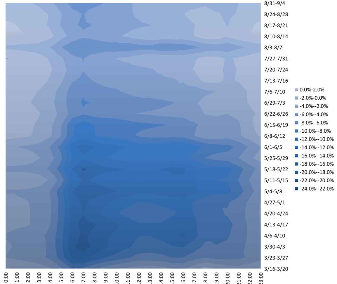
NYCA Load Profile - Weekday Diurnal Load Changes
