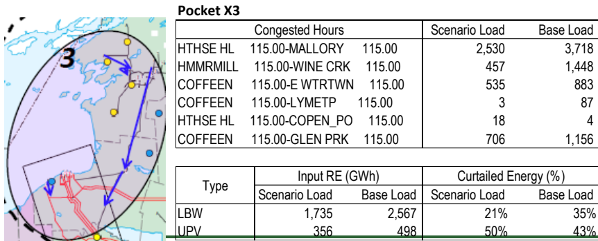
Figure 86: Pocket X3 Congestion and Curtailment Summary
