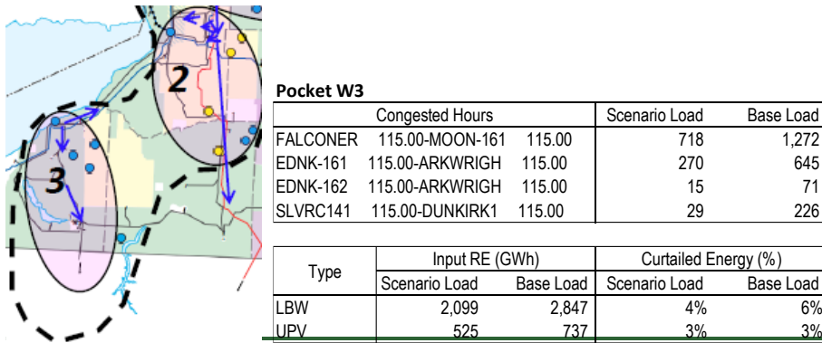
Figure 83: Pocket W3 Congestion and Curtailment Summary
