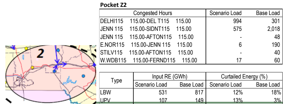
Figure 90: Pocket Z2 Congestion and Curtailment Summary
