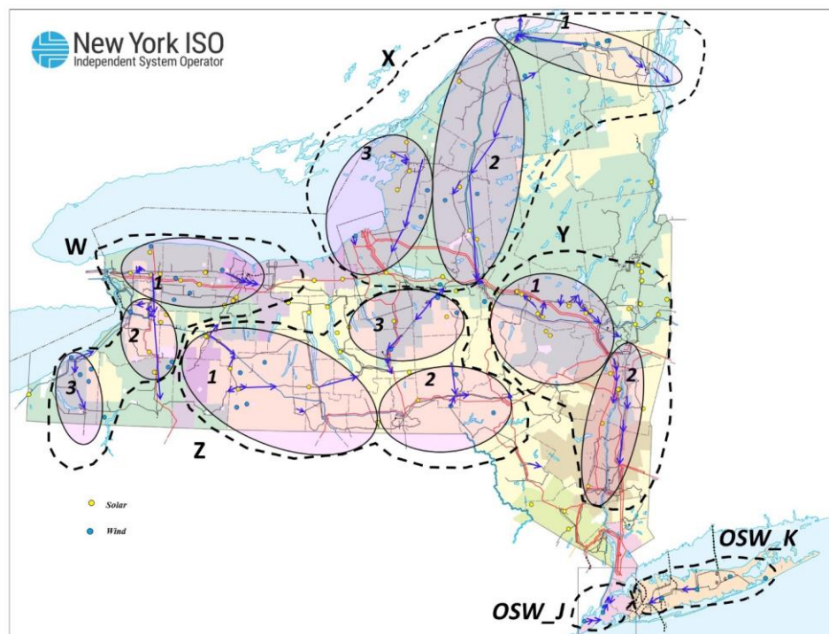
Figure 75: Map of Renewable Generation Pockets and Constraints
