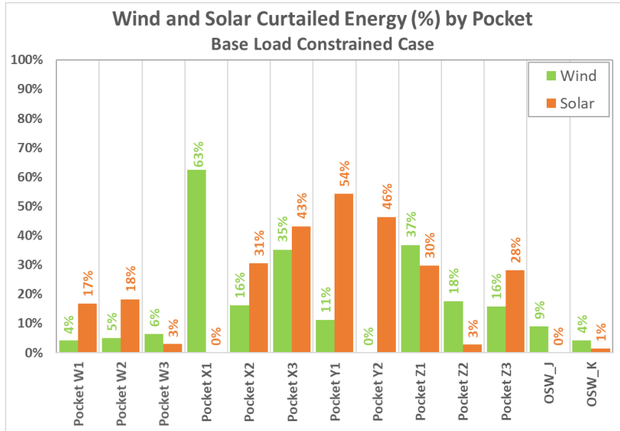
Figure 79: Curtailed Energy Percentage by Pocket Summary in (Base Load Constrained Case)
