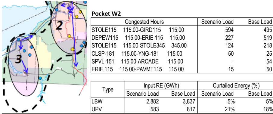
Figure 82: Pocket W2 Congestion and Curtailment Summary
