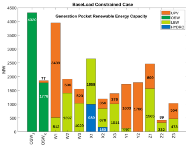
Figure 77: Generation-Pocket Renewable Energy Capacity in-by Pocket (Base Load CasesCase)
