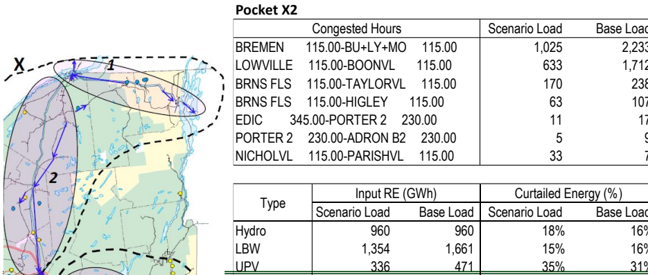
Figure 85: Pocket X2 Congestion and Curtailment Summary
