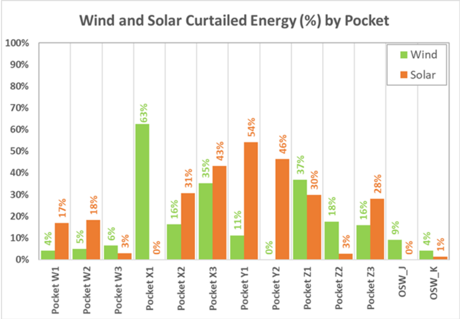
Figure 767: Wind and Solar Curtailment by Pocket
