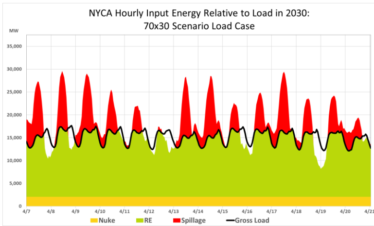
Figure 653165: Hourly Input Approach Illustration
