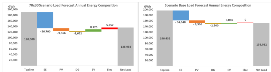
Figure 632963: 70x30 Scenario and Scenario Base Load Forecasts Energy Component Breakdown
