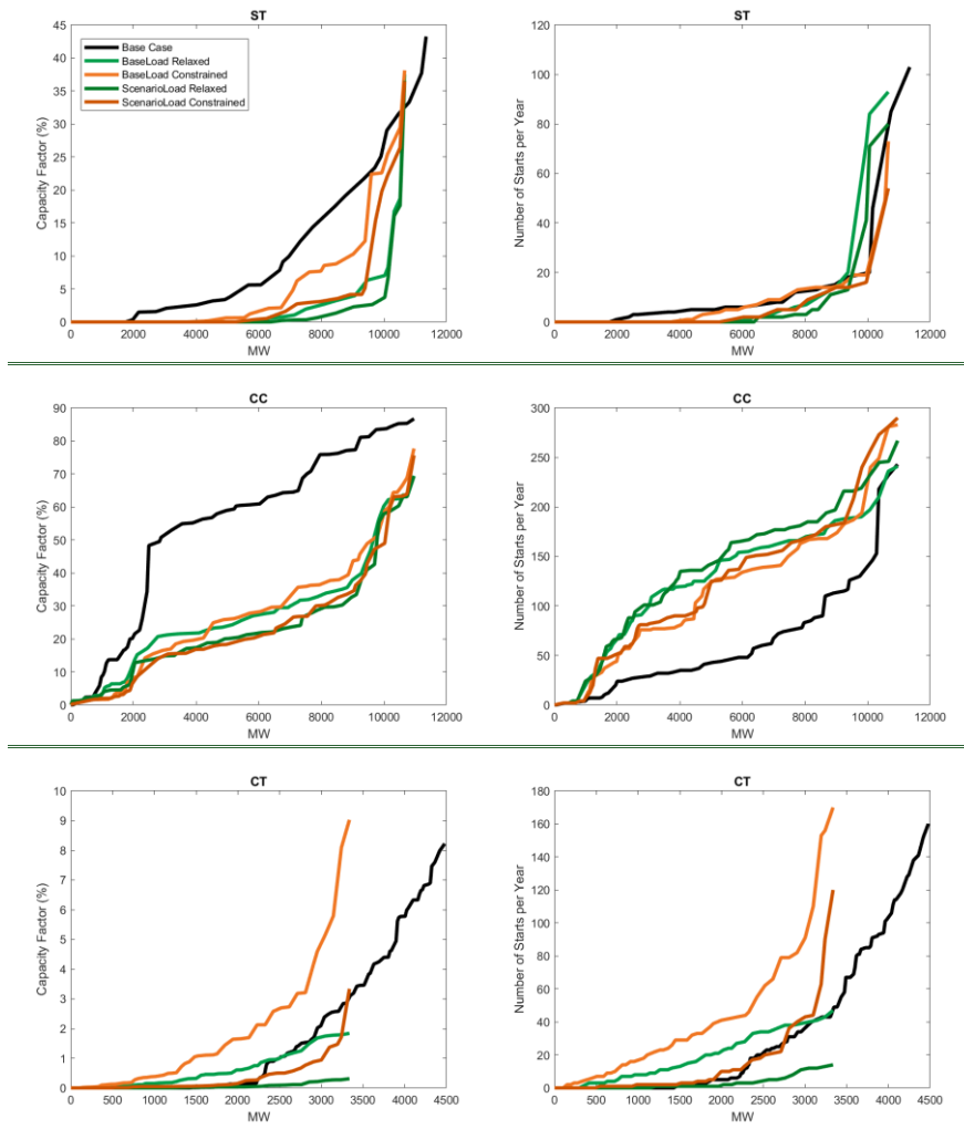
Figure 72: Base Load Relaxed and Constrained Cases Fossil Fleet Cumulative Capacity Curves
