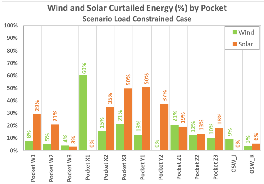
Figure 78: Curtailed Energy Percentage by Pocket Summary in (Scenario Load Constrained Case)
