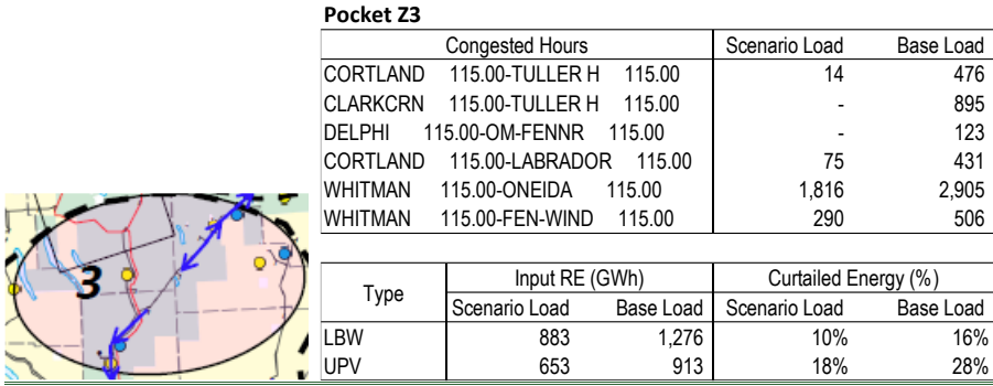
Figure 91: Pocket Z3 Congestion and Curtailment Summary
