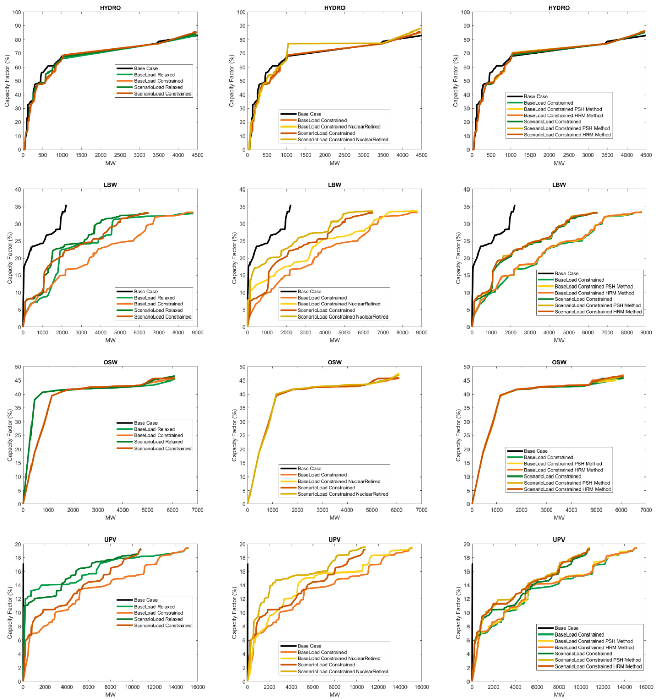
Figure 87: Renewable Fleet Cumulative Capacity Factor Curves
