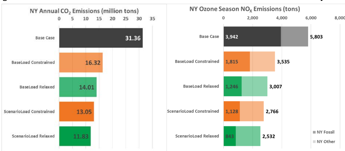
Figure 73: Base Load Relaxed and Constrained Cases CO 2 and Ozone Season NO x Emissions Projections
