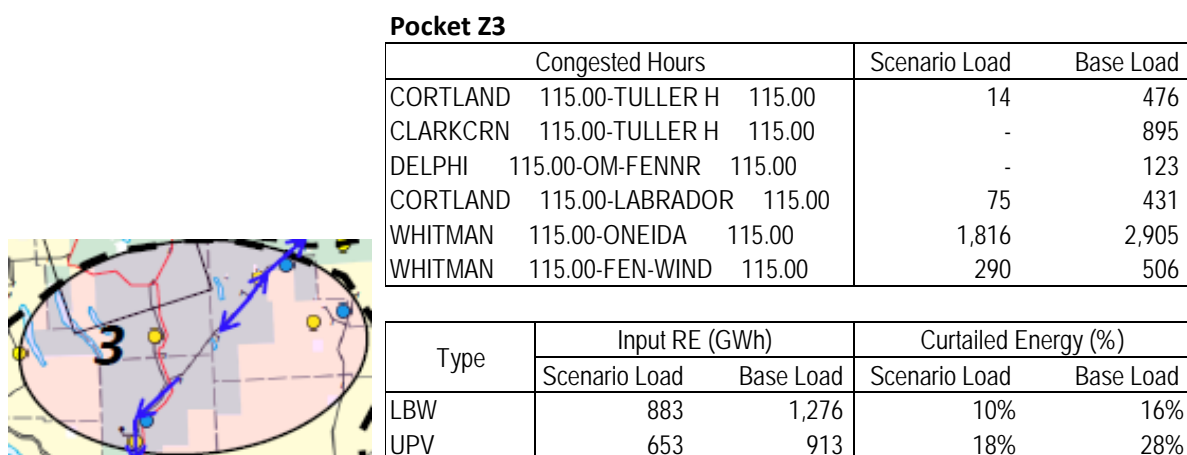
Figure 91: Pocket Z3 Congestion and Curtailment Summary
