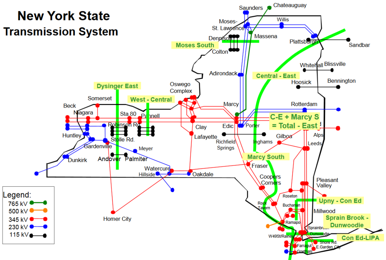
Figure 7: NYISO 230 kV and Above Transmission Map
