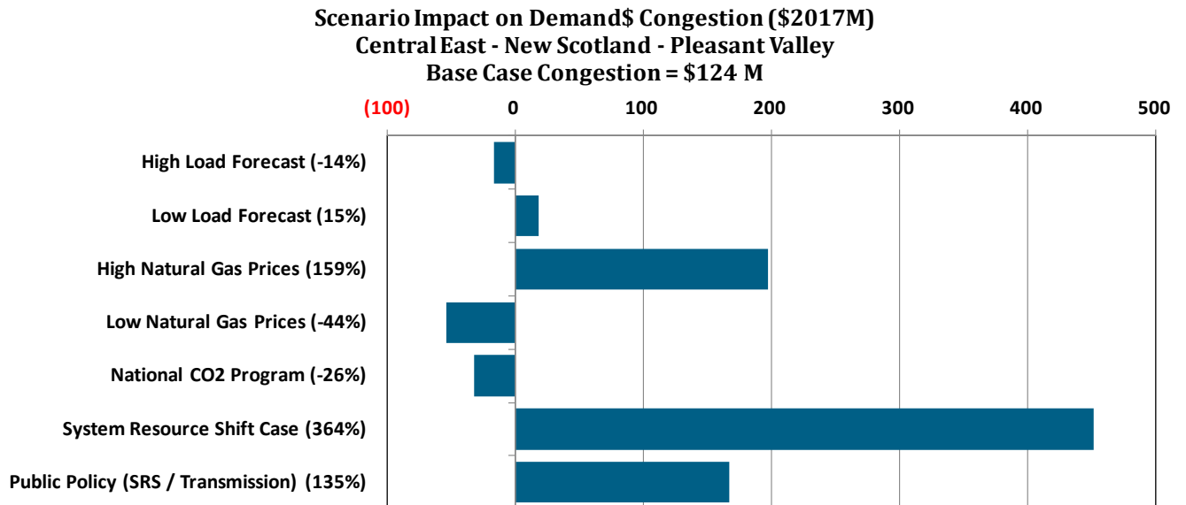
Figure 70: Scenario Impact on Central East - New Scotland - Pleasant Valley Congestion
