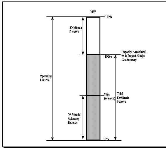
Figure 6-1 Operating Reserve Requirements
