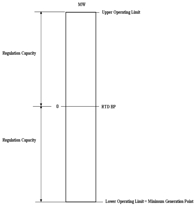
Figure 4-3 LESR with Full Regulation Service Deployment
