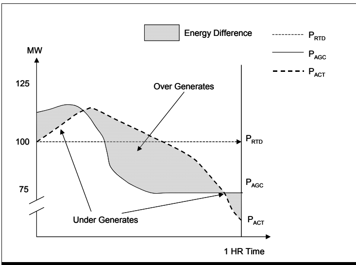
Figure 4-7 Error in Performance (30-Second Bandwidth not Included)
