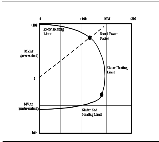
Figure 3-1 Generator MVAR versus MW Capability
