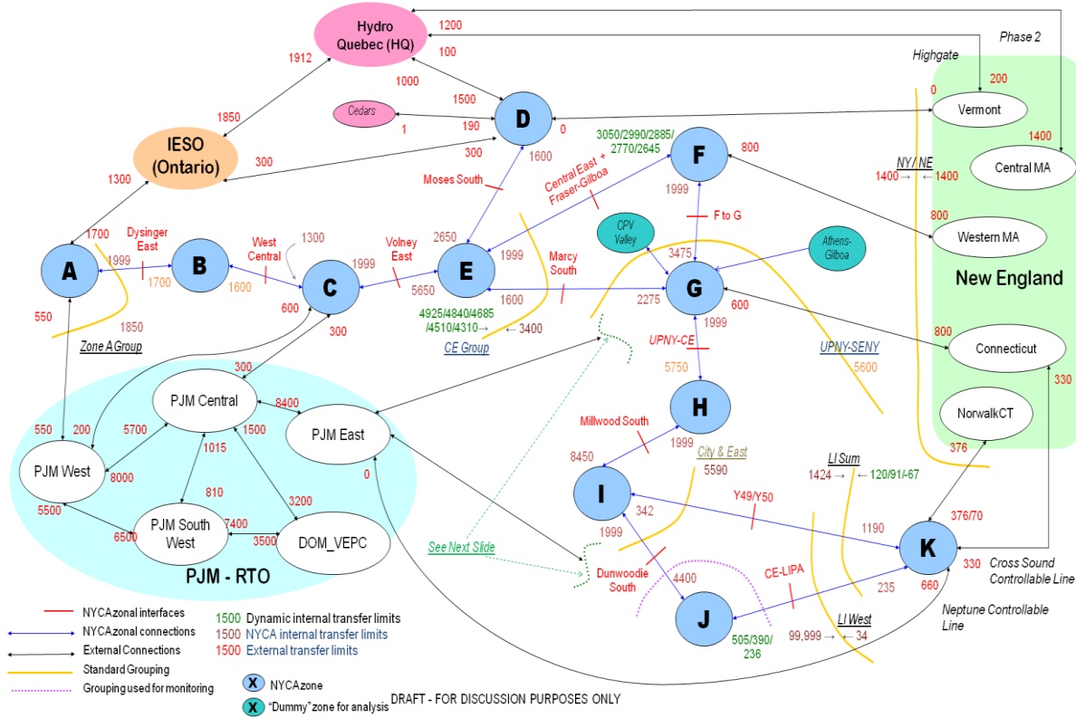
Figure 5-3: 2016 RNA Final Topology Year 2 to 10 (2018-2026)
