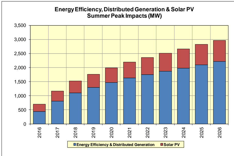
Figure 4-4: 2016 Energy Efficiency & Behind-the-Meter Solar PV – Summer Peak
