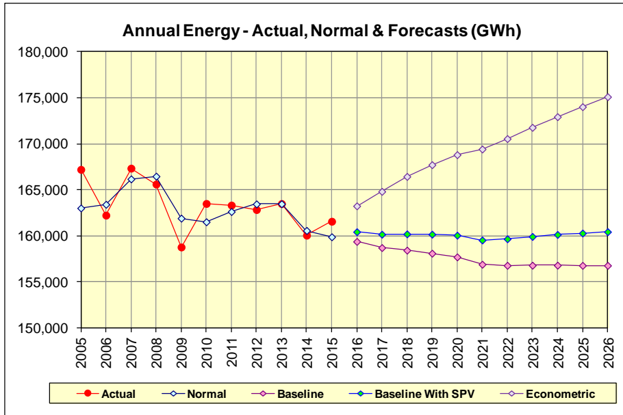
Figure 4-1: 2016 Econometric, Baseline and Baseline W with SPV Energy Forecasts
