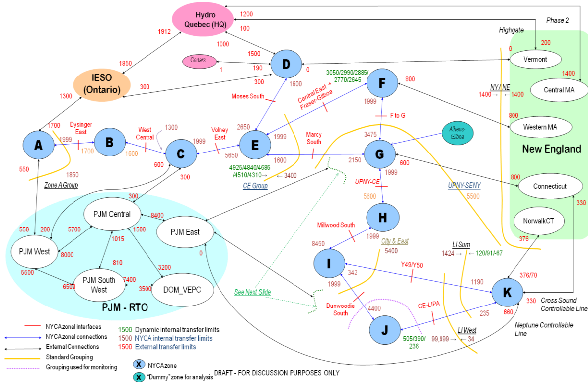
Figure 5-2: 2016 RNA Final Topology Year 1 (2017)
