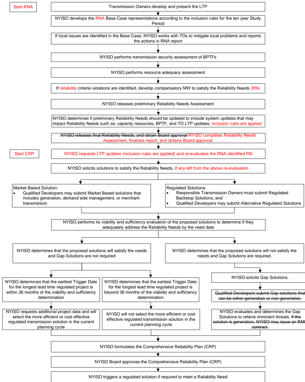
Figure 2-1: NYISO Comprehensive Reliability Planning Process (RPP)
