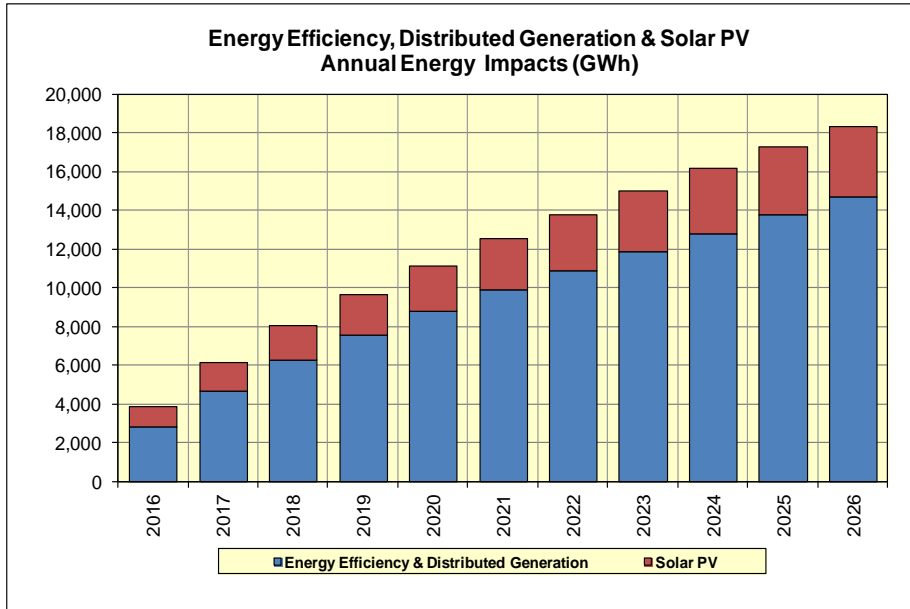
Figure 4-3: 2016 Energy Efficiency & Behind-the-Meter Solar PV – Annual Energy
