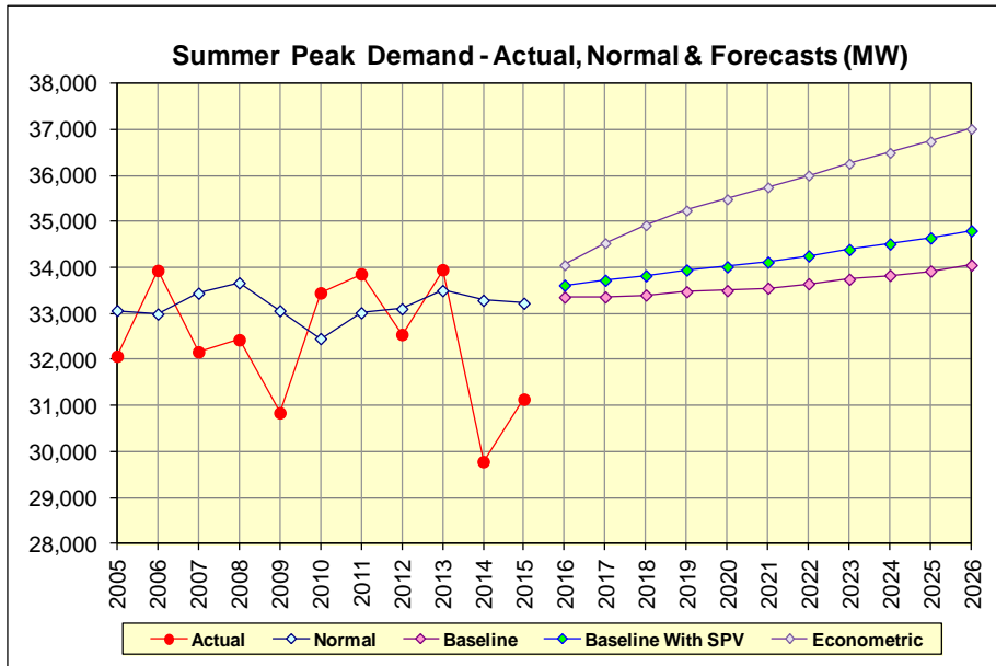
Figure 4-2: Econometric, Baseline and Baseline W with SPV Summer Peak Demand Forecast
