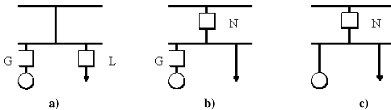
Figure 5-1 Metering Configuration
