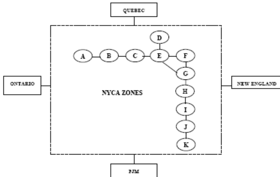
Figure 5.5-2: A simplified version of different zones and the external systems
