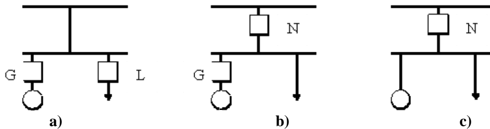
Figure 5-1 Metering Configuration
