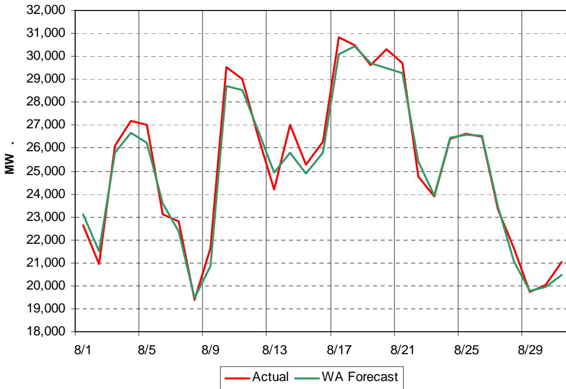
NYISO Daily Peak Load - August 2009 Actual vs Weather-Adjusted Forecast
