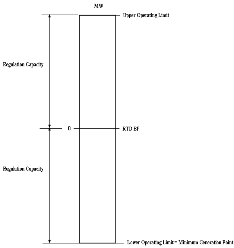
Figure 4-3 LESR with Full Regulation Service Deployment
