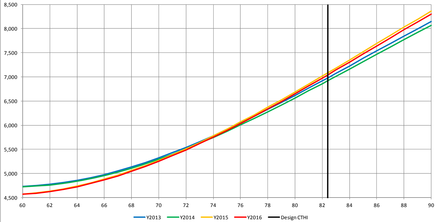
Weather Normalized Load vs CTHI, 2013 - 2016
