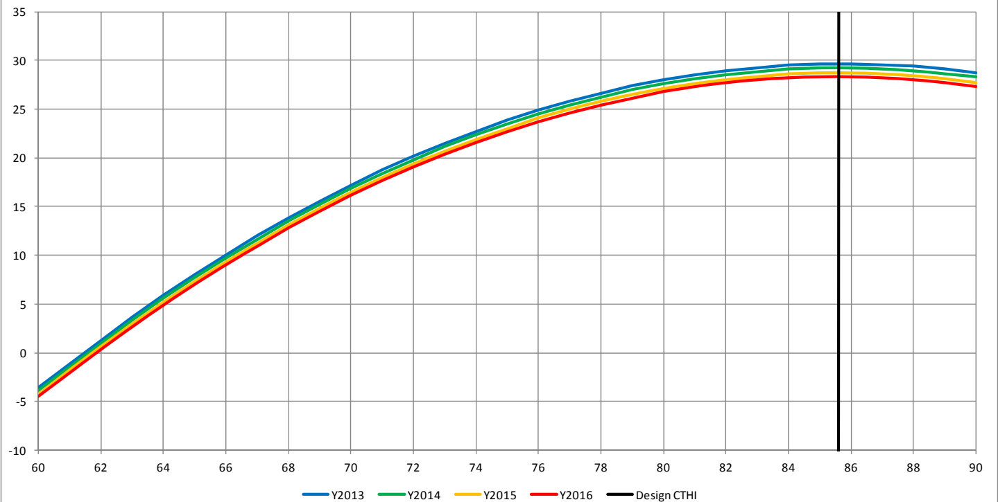
Central Hudson Weather Response vs CTHI, 2013 - 2016
