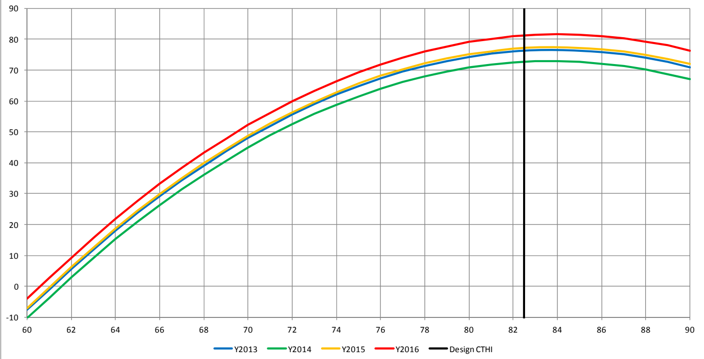
Weather Response vs CTHI, 2013 - 2016
