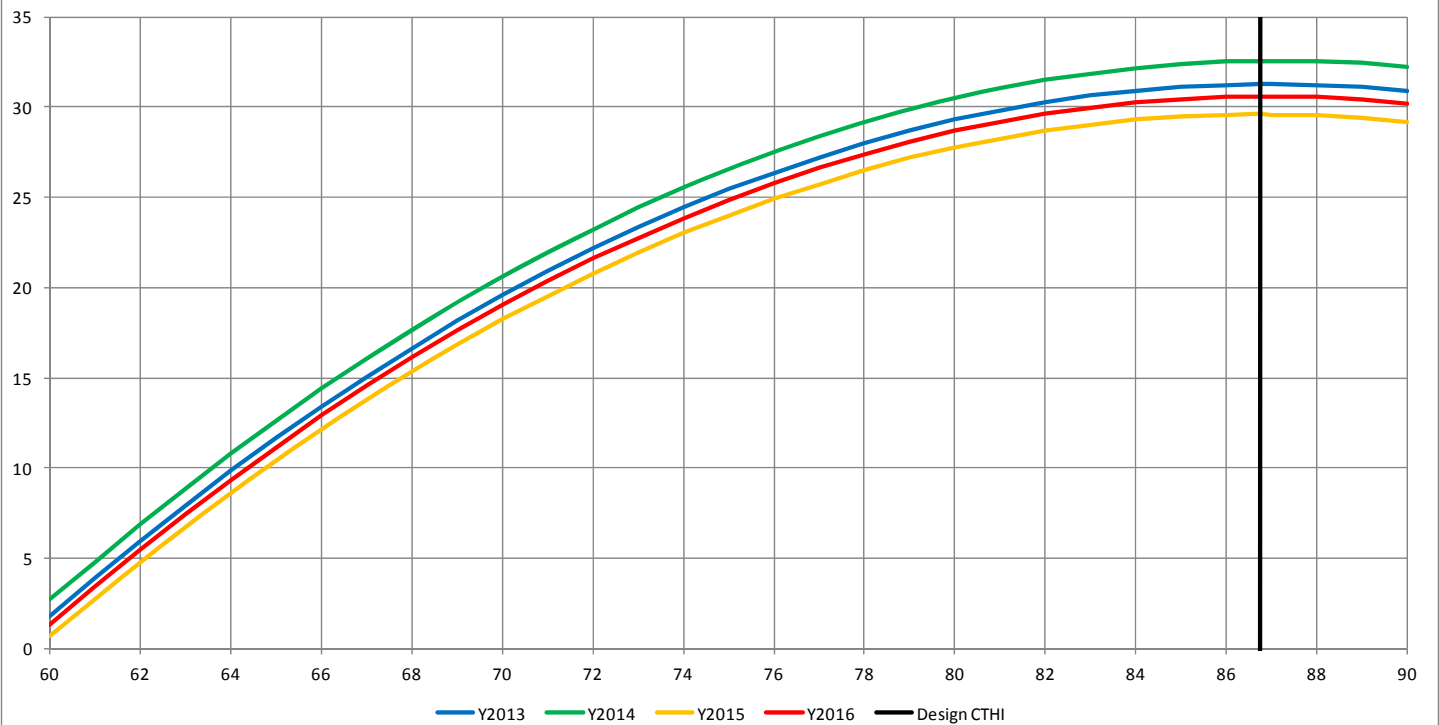
O&R Weather Response vs CTHI, 2013 - 2016
