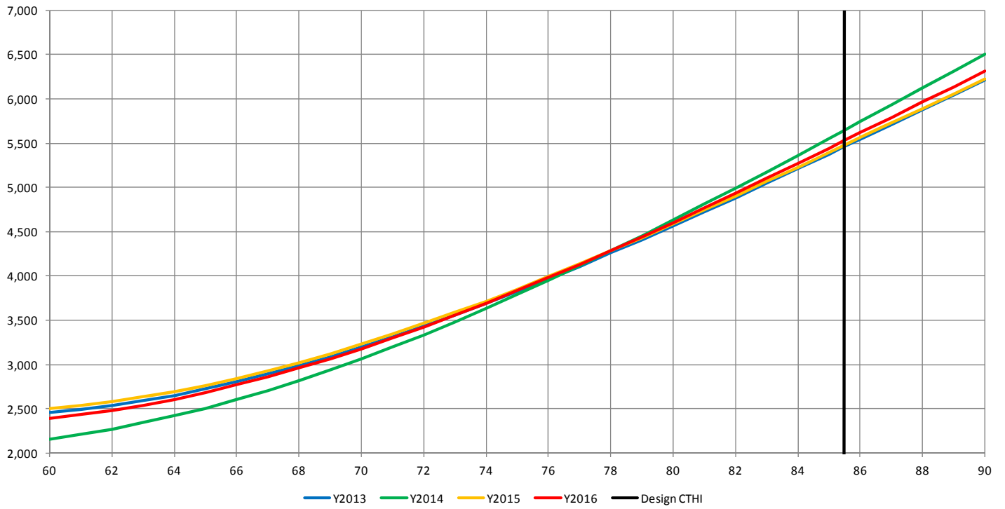
LIPA Weather Normalized Load vs CTHI, 2013 - 2016
