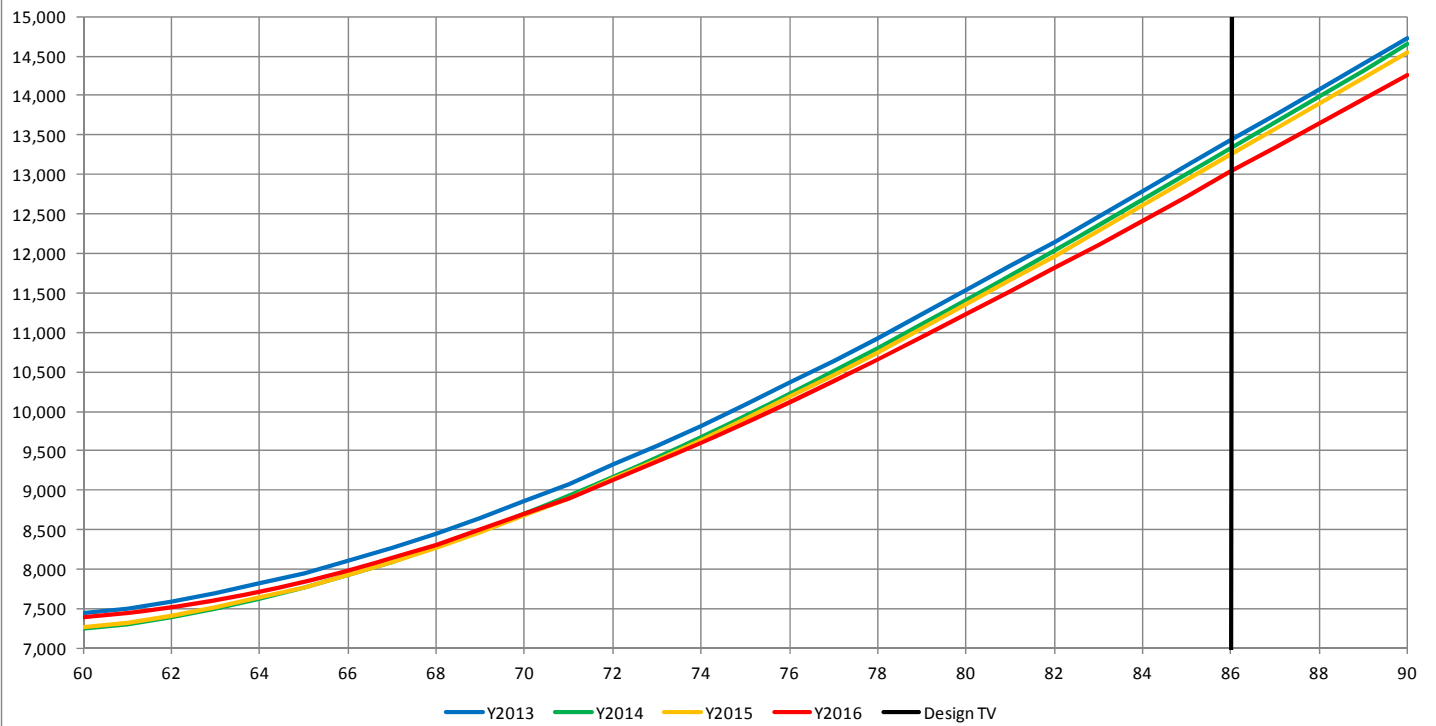
Con Ed Weather Normalized Load vs TV, 2013 - 2016
