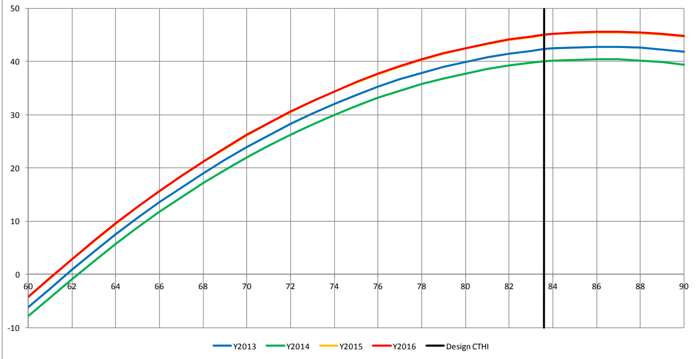
RG&E Weather Response vs CTHI, 2013 - 2016
