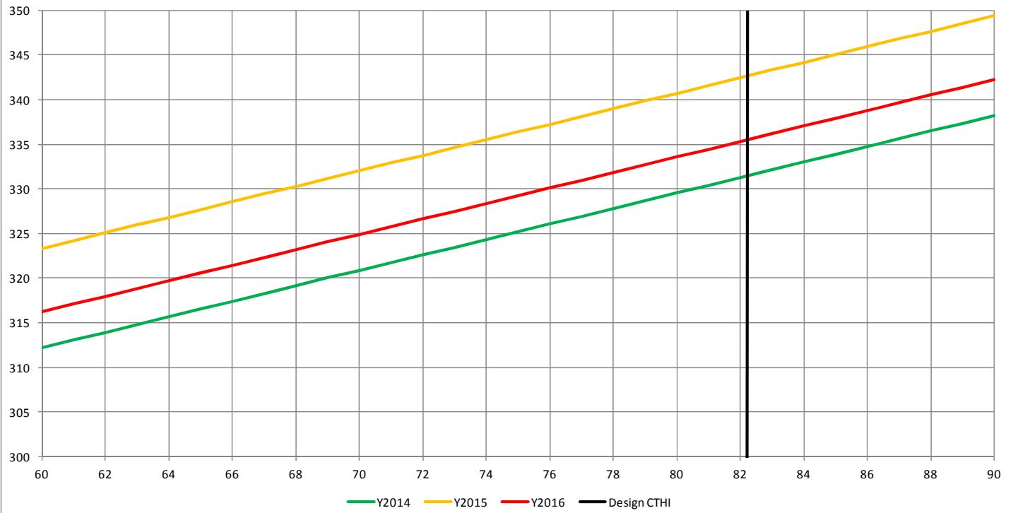
NYPA Weather Normalized Load vs CTHI, 2014 - 2016
