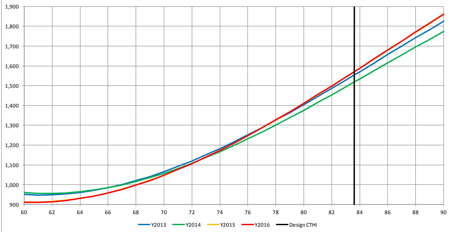
RG&E Weather Normalized Load vs CTHI, 2013 - 2016
