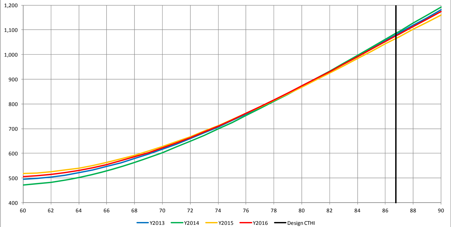
O&R Weather Normalized Load vs CTHI, 2013 - 2016
