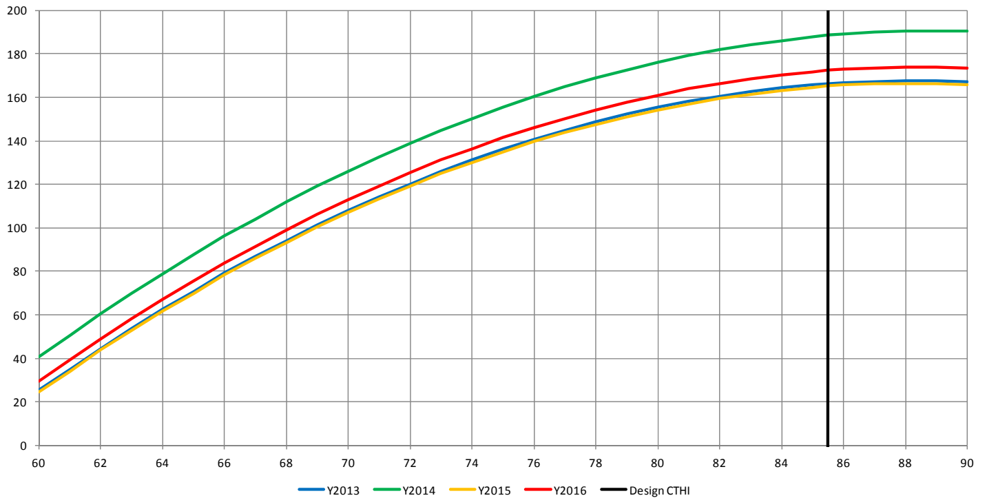
LIPA Weather Response vs CTHI, 2013 - 2016
