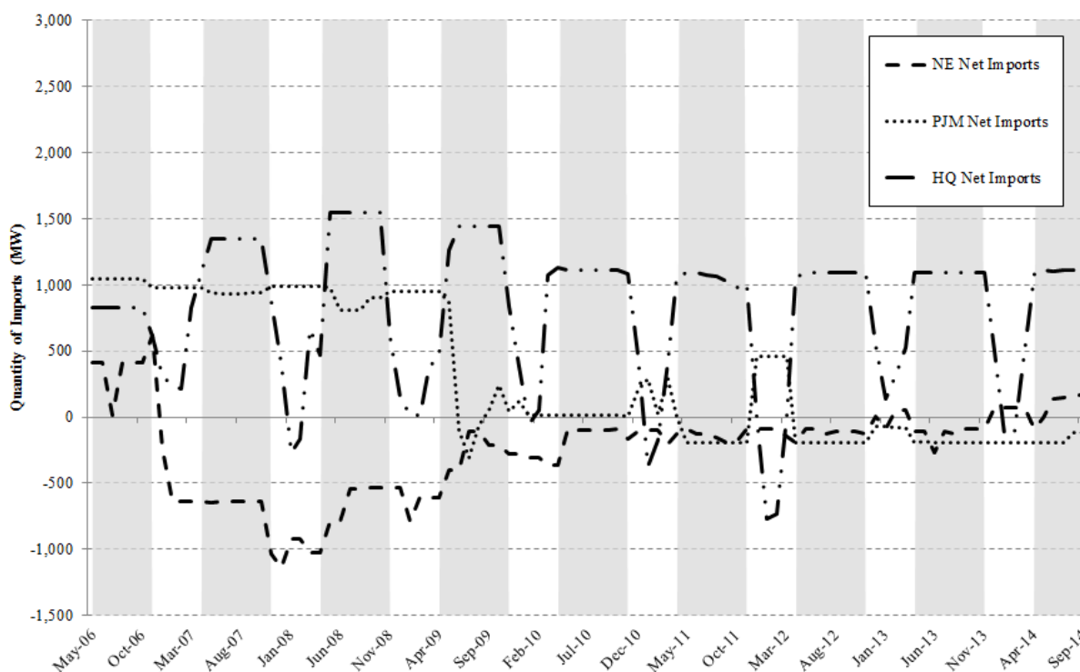
Figure 27: NYISO Net Imports (UCAP MW) by Region
