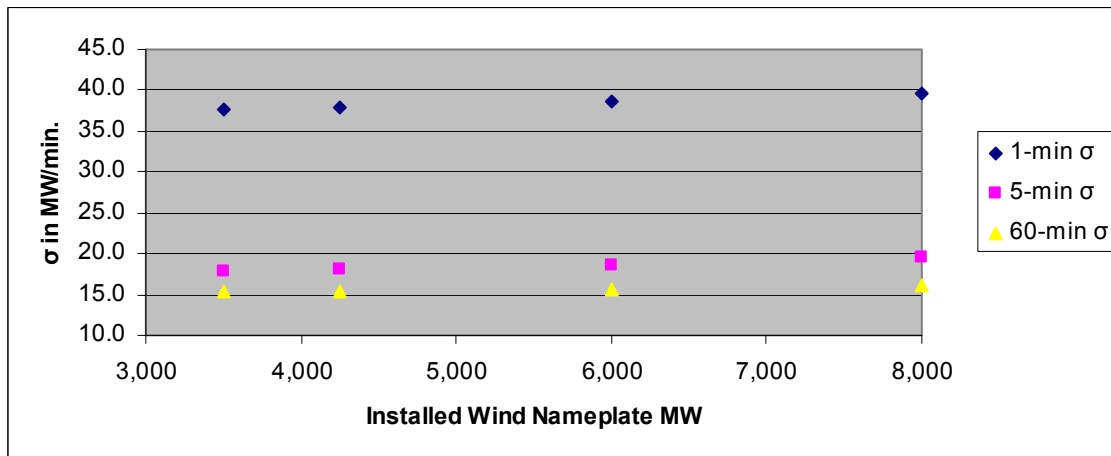
Figure 5.11: Normalized \sigma VS Installed Wind MWs
