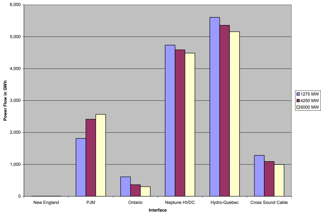
Figure 5.62: Changes in Imports for 2013 as Wind Plant Penetration Increases
