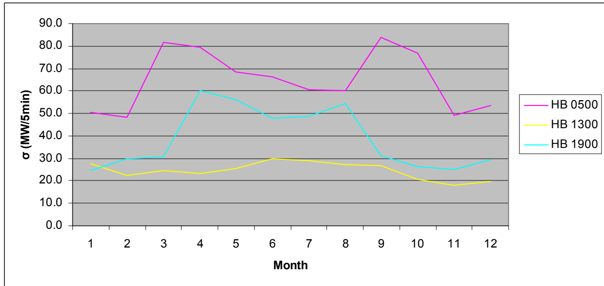
Figure 5.13: Sigma by the Hour of the Day for 5-min. Net-Load \Delta for 2008
