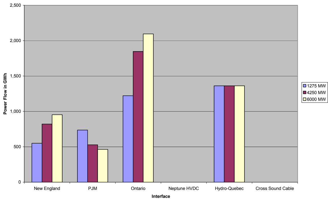
Figure 5.63: Changes in Exports for 2013 as Wind Plant Penetration Increases
