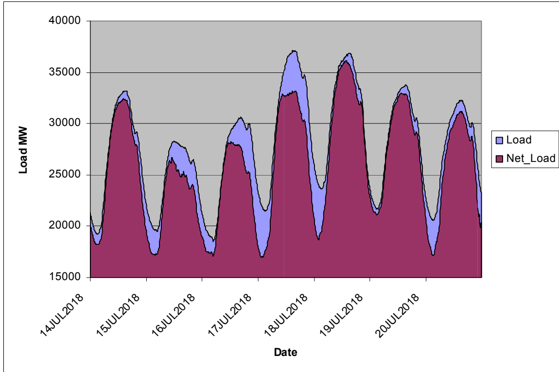
Figure 5.7: Load and Net Load for the Simulated 2018 Summer Peak Week
