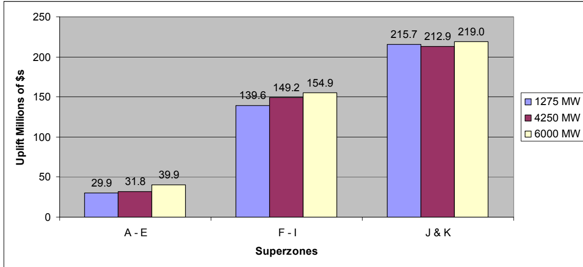
Figure 5.72: Uplift Costs for 2013 as the Level of Installed Wind Increases
