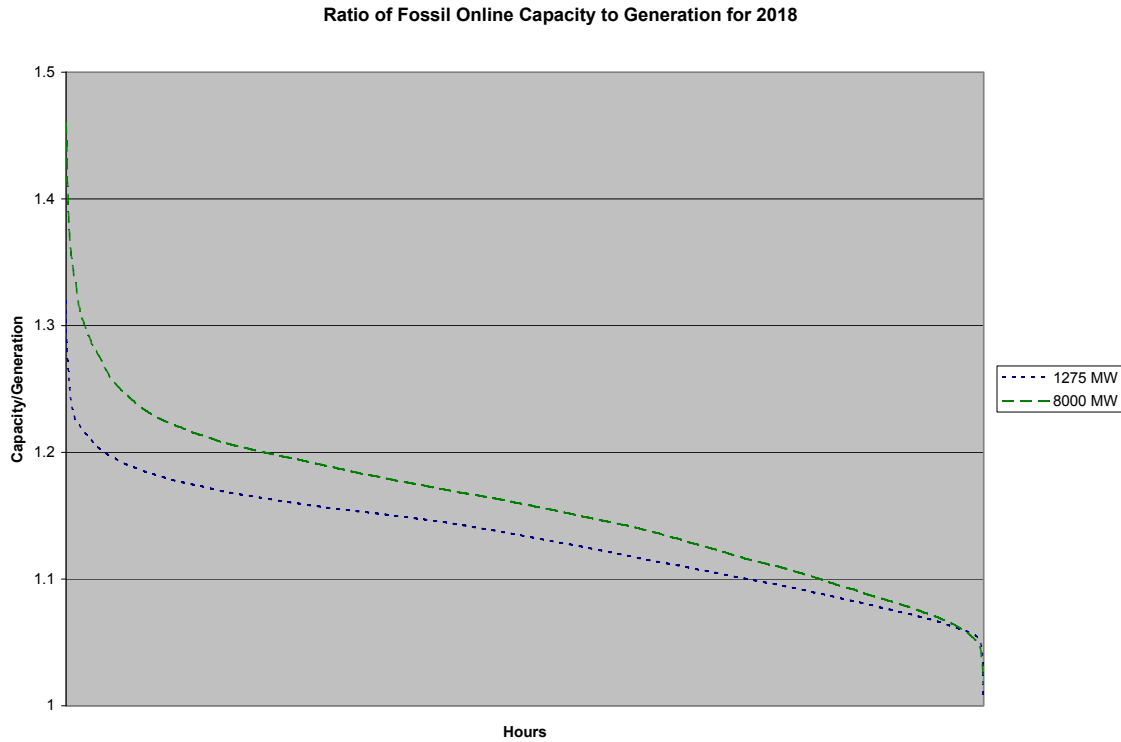
Figure 5.32: Ratio of the Committed Fossil Fired Generation MW to the Energy Produced
