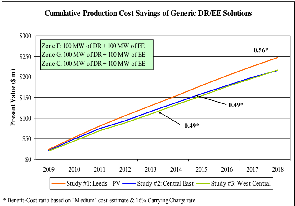
Figure 21: Cumulative Benefits of Generic Demand Response/Energy Efficiency Solutions of Each Study (Present Value in 2009 $ in Millions)
