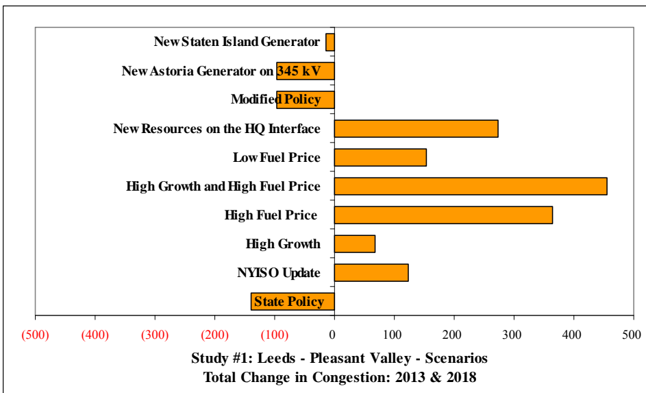
Figure 6: Scenarios Impact on Congestion in Leeds-Pleasant Valley Study
