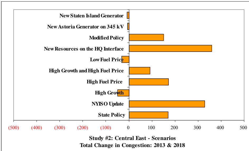
Figure 7: Scenarios Impact on Congestion in Central East Study
