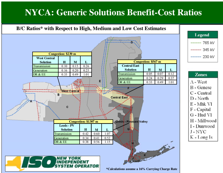
Figure 18: B/C Ratio (High, Medium, and Low Cost Estimate Ranges)
