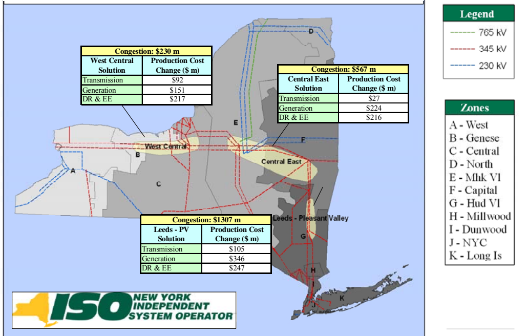
Figure 2: NYCA Generic Solutions Production Cost Savings
