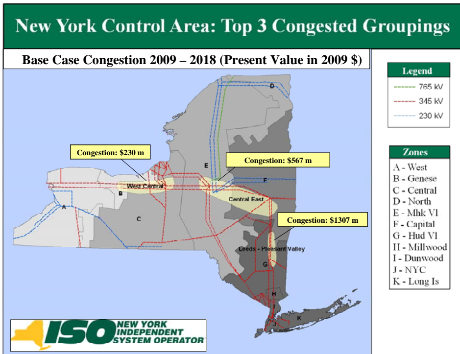
Figure 1: Projected Congestion on the Top Three CARIS Elements (present value in 2009 $ in Millions)
