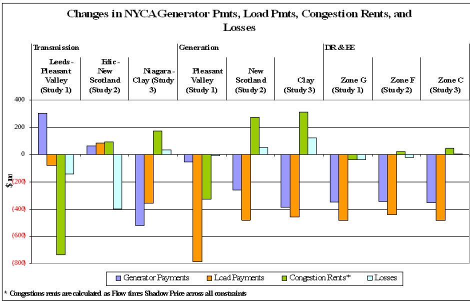
Figure 4: Change in Generator Payments, Load Payments, Congestion Rents, and Losses
