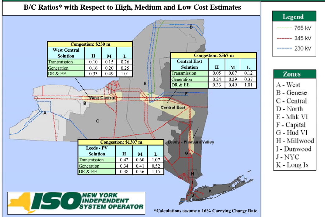
Figure 3: NYCA Generic Solutions Benefit/Cost Ratios
