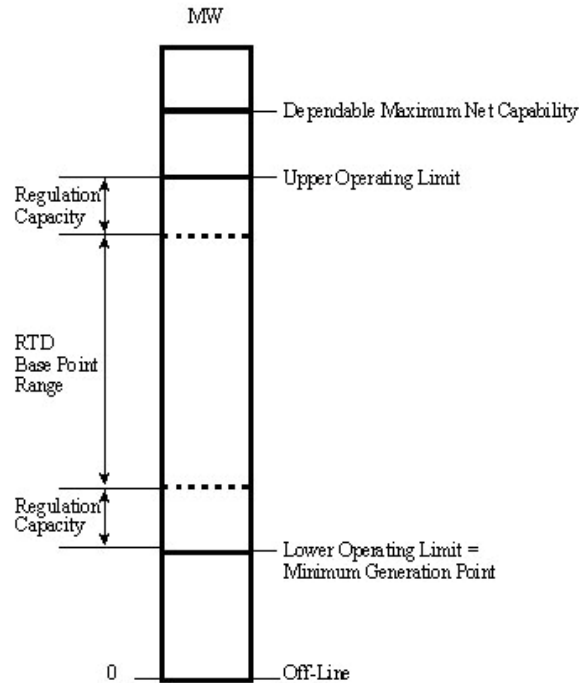
Figure 4.2b: Generating Unit Operating Characteristics
