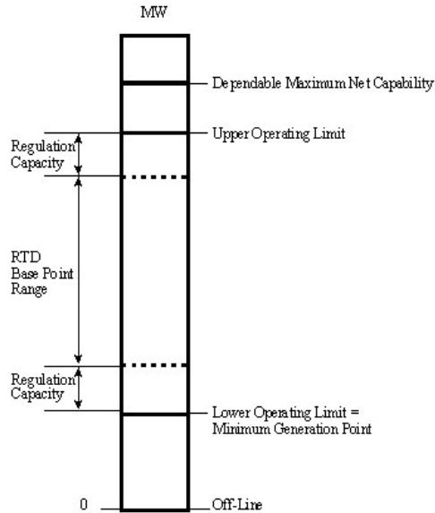
Figure 4.2b: Generating Unit Operating Characteristics
