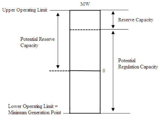
Figure 4.2a: Demand Side Resources Operating Characteristics
