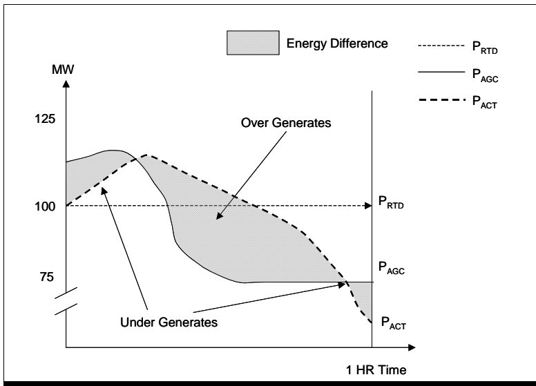
Figure 4.4: Error in Performance (30 Second bandwidth not included)
