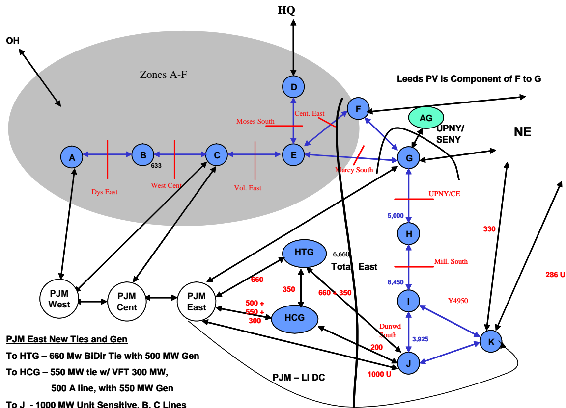
New York Control Area Transmission System Representation 2008 CRP Evaluation of Market Solutions
