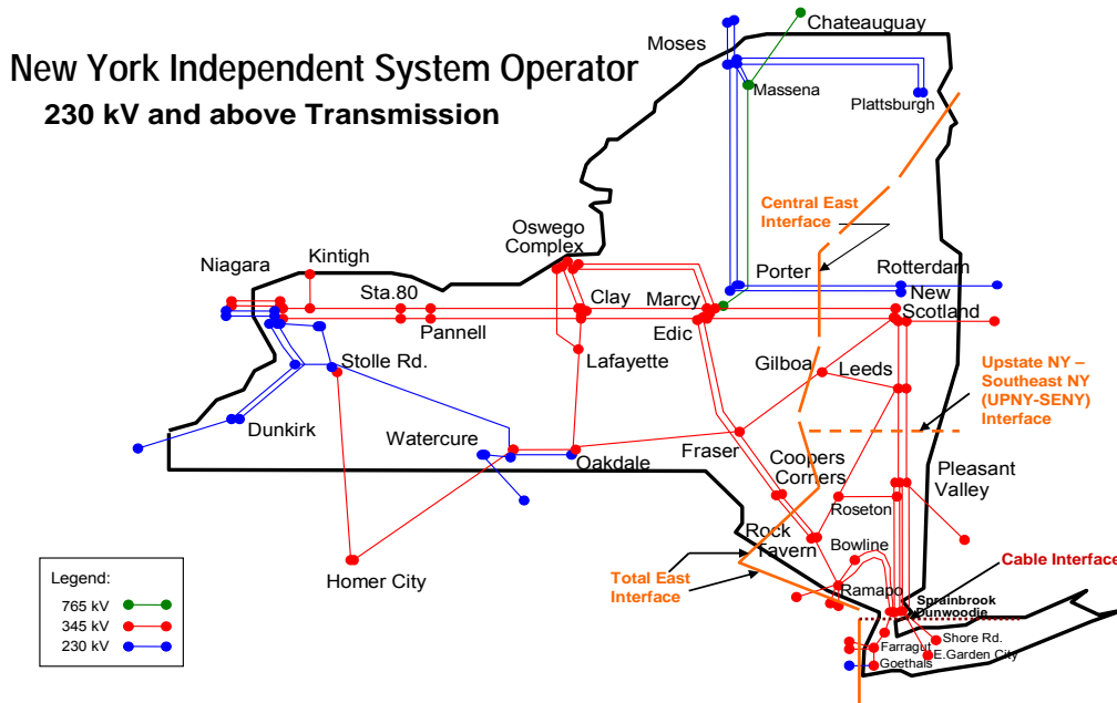
Figure 5.1.1: NYISO 230 kV and above Transmission Map
