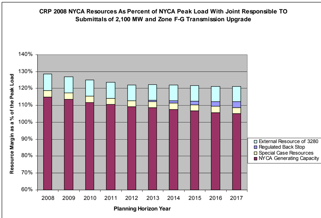
Figure 5.2.1: TO Regulated Backstop Solutions – 2,100 MW
