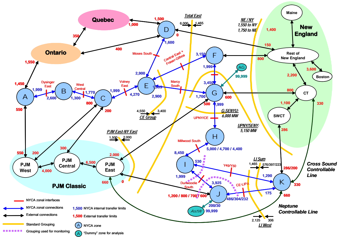
New York Control Area Transmission System Representation For 2008 Summer Ratings
