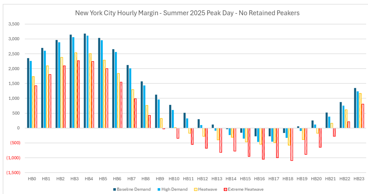
Figure 14: New York City Hourly Transmission Security Margin – Summer Peak
