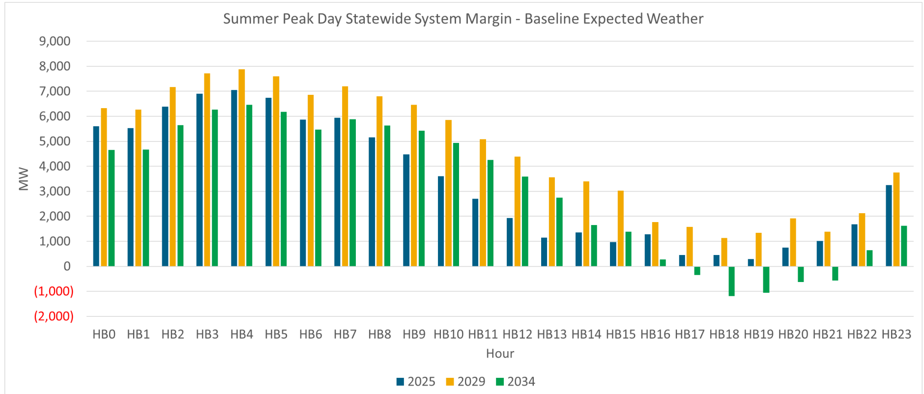
Figure 34: Summer Peak Statewide System Hourly Margin Chart
