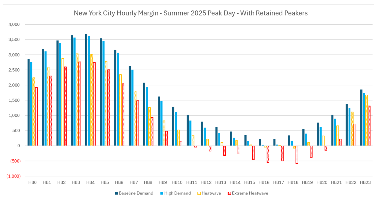
Figure 19: New York City Hourly Margin with Designated Peakers
