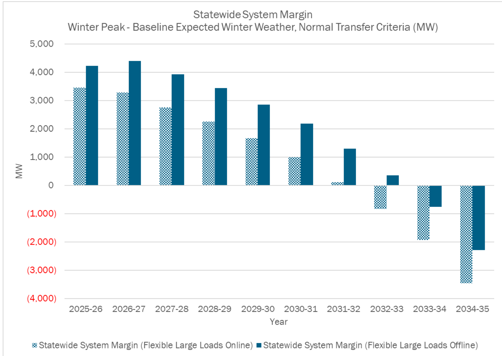
Figure 37: Winter Peak Statewide System Margin – Flexible Large Loads Comparison
