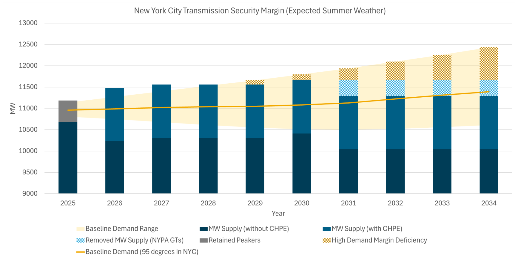
Figure 46: New York City Transmission Security Margin Summary – Summer Peak
