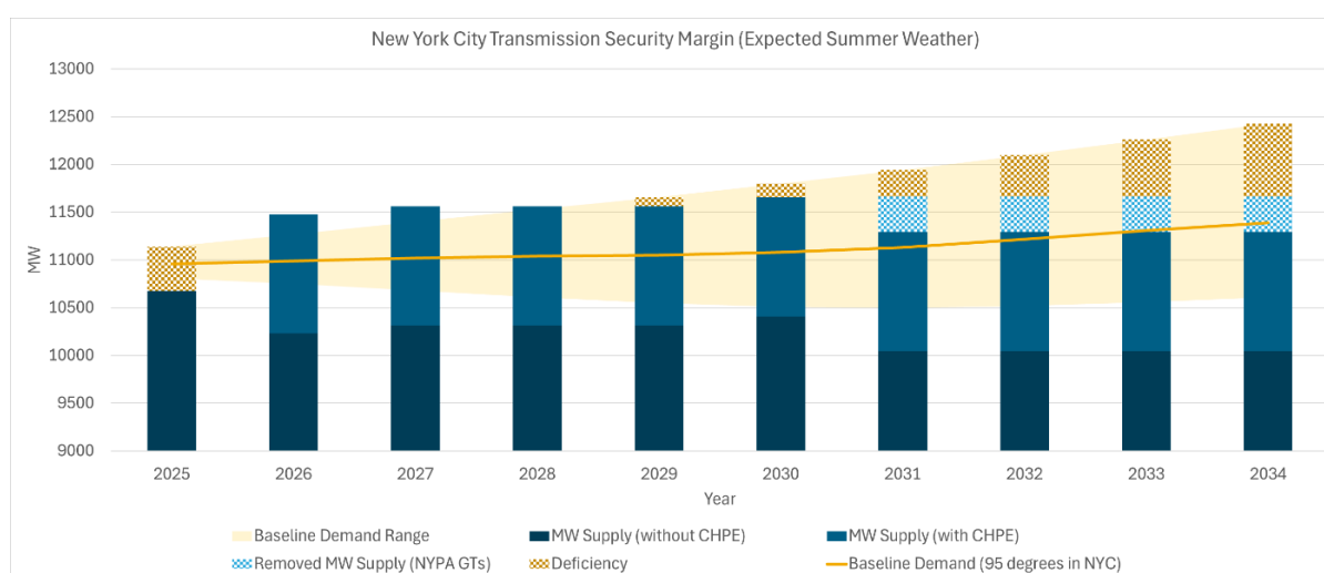
Figure 14: New York City Hourly Transmission Security Margin – Summer Peak
