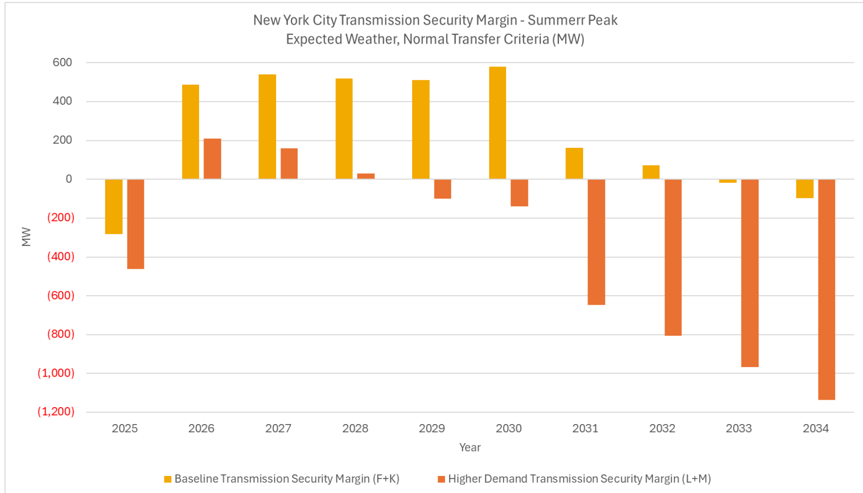
Figure 45: New York City Transmission Security Margin Results – Summer Peak
