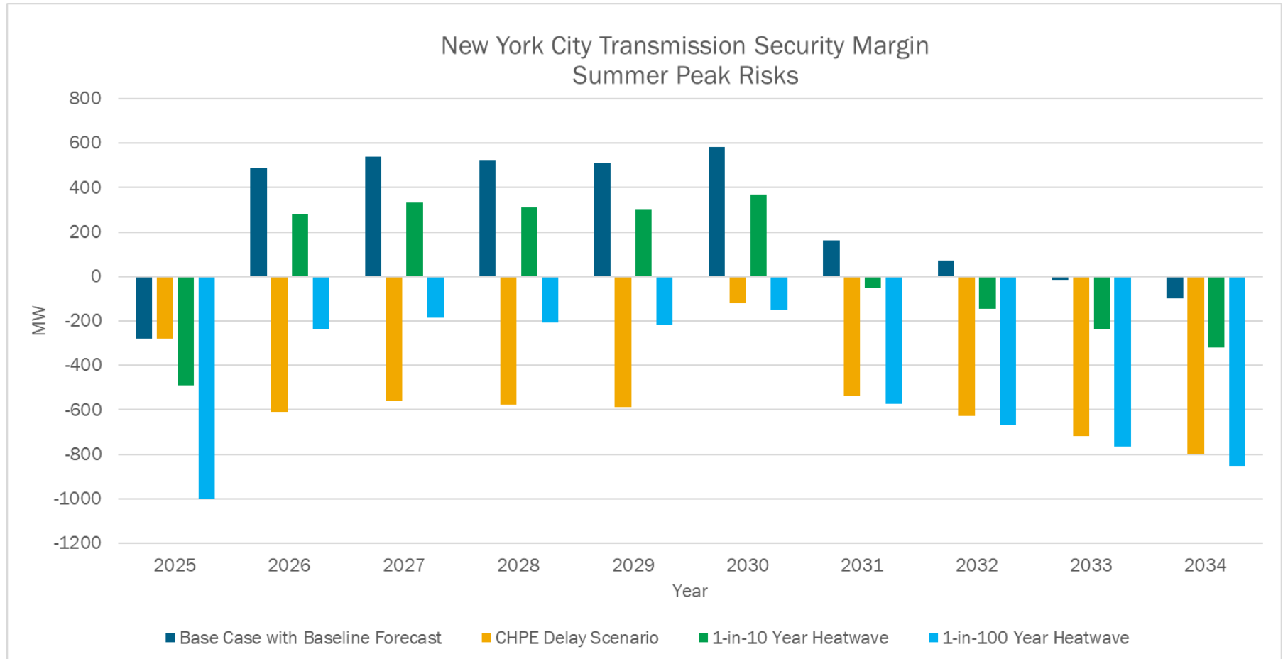
Figure 53: New York City Transmission Security Margin Risks
