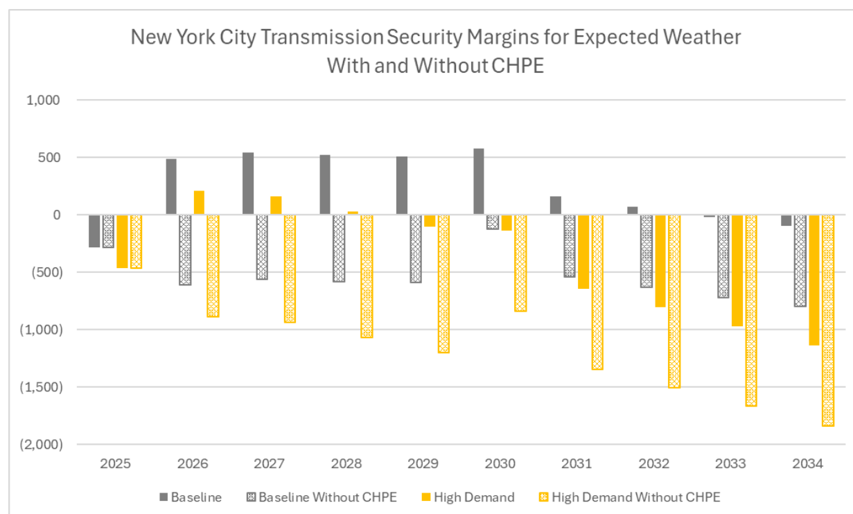
Figure 15: New York City Transmission Security Margin – Summer Peak - With and Without CHPE
