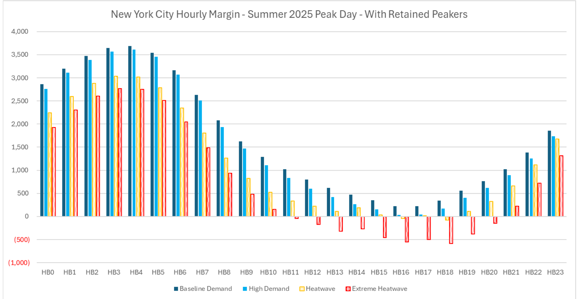
Figure 48: New York City Hourly Transmission Security Margin – 2025 Summer Peak Day – With Retained Peakers
