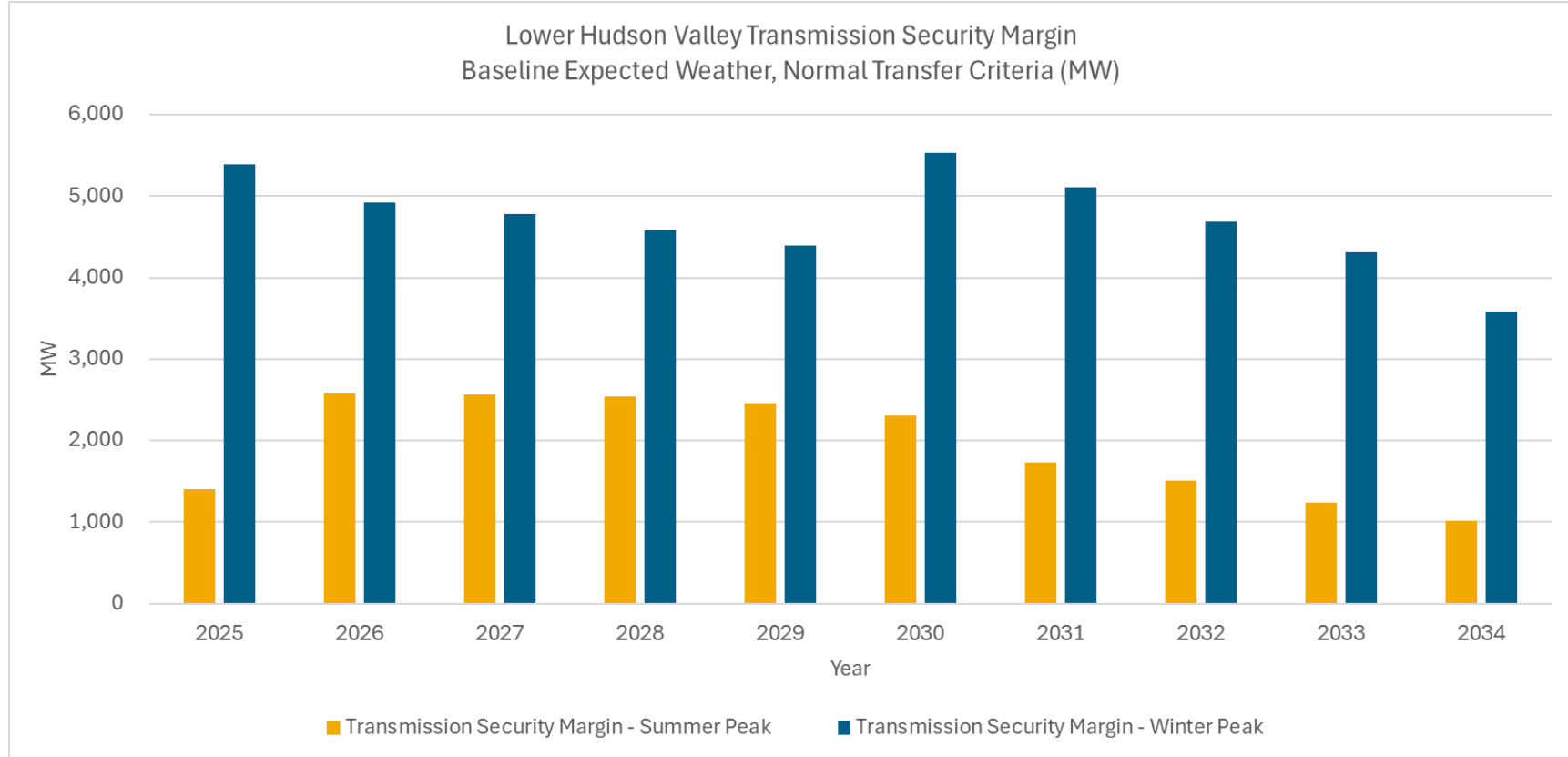
Figure 42: Lower Hudson Valley Margin Chart – Summer and Winter
