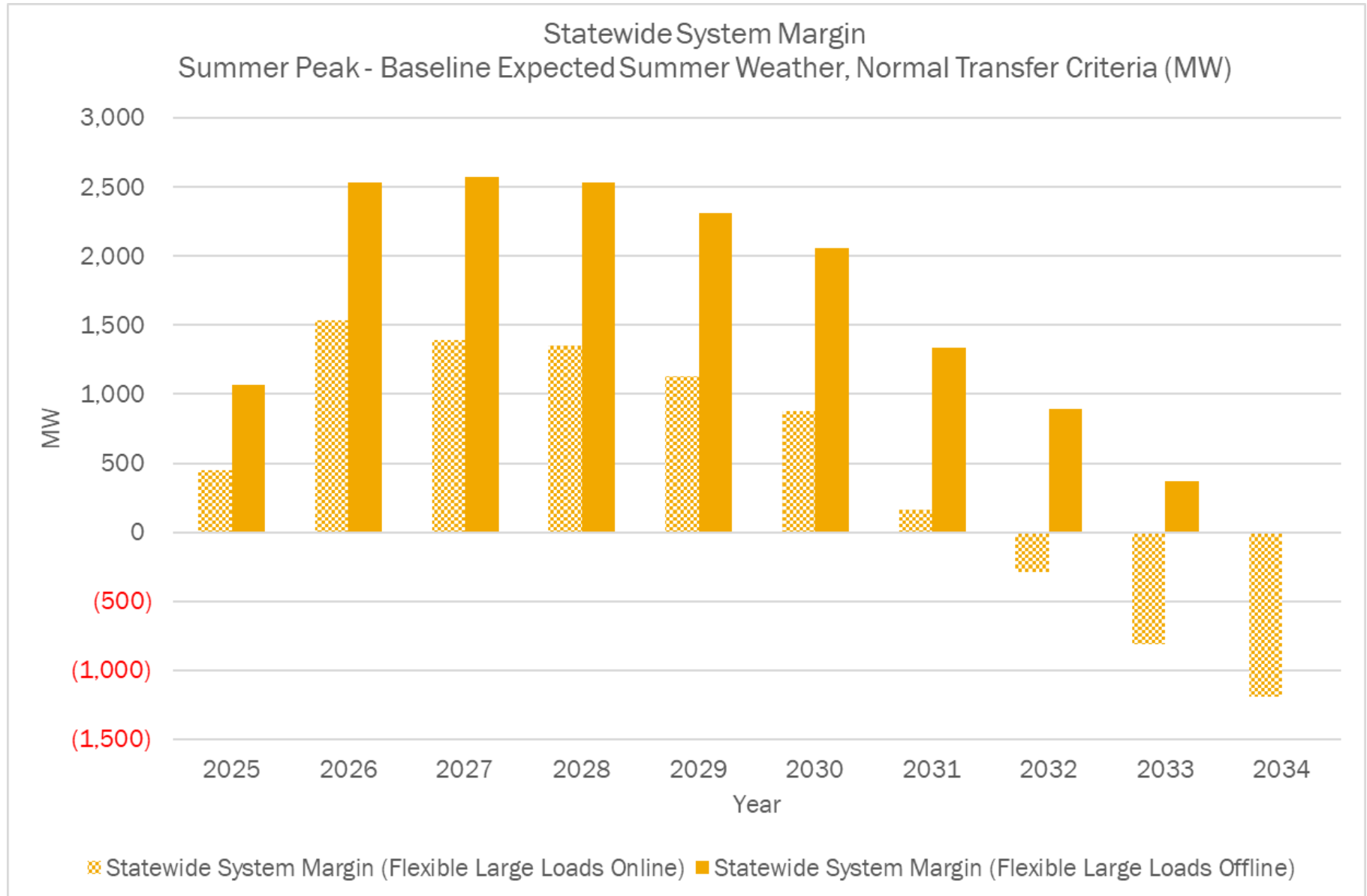
Figure 31: Summer Peak Statewide System Margin – Flexible Large Loads Comparison
