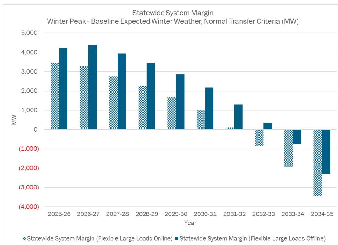
Figure 17: Statewide System Margin – Winter Peak
