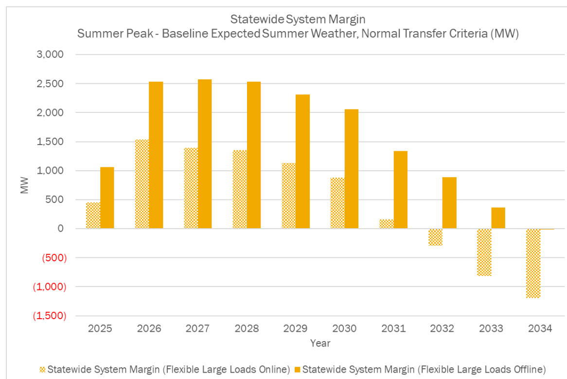
Figure 16: Statewide System Margin – Summer Peak
