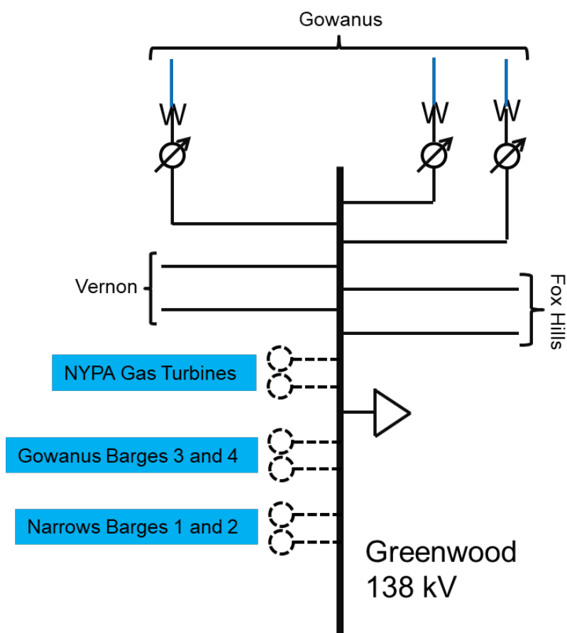
Figure 20: Greenwood 138 kV TLA
