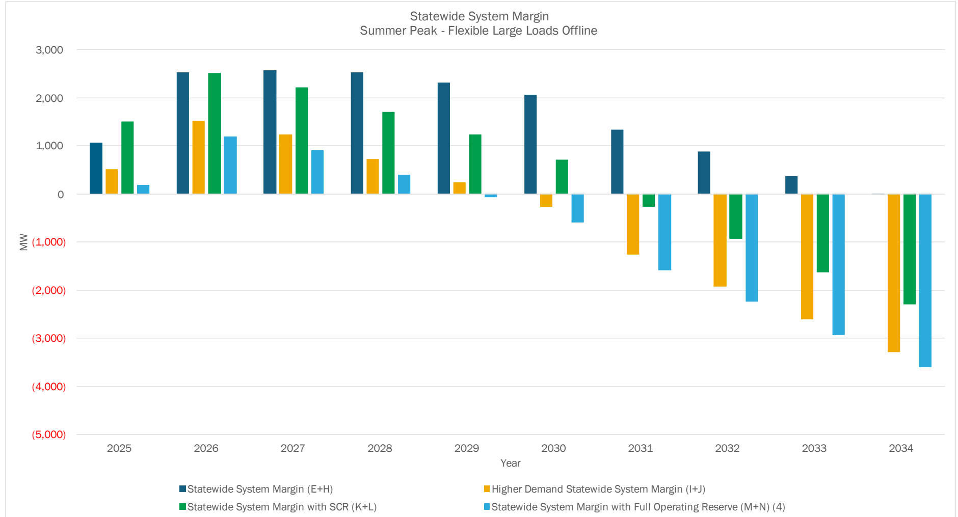
Figure 32: Summer Peak Statewide System Margin Chart (Flexible Large Loads Offline)
