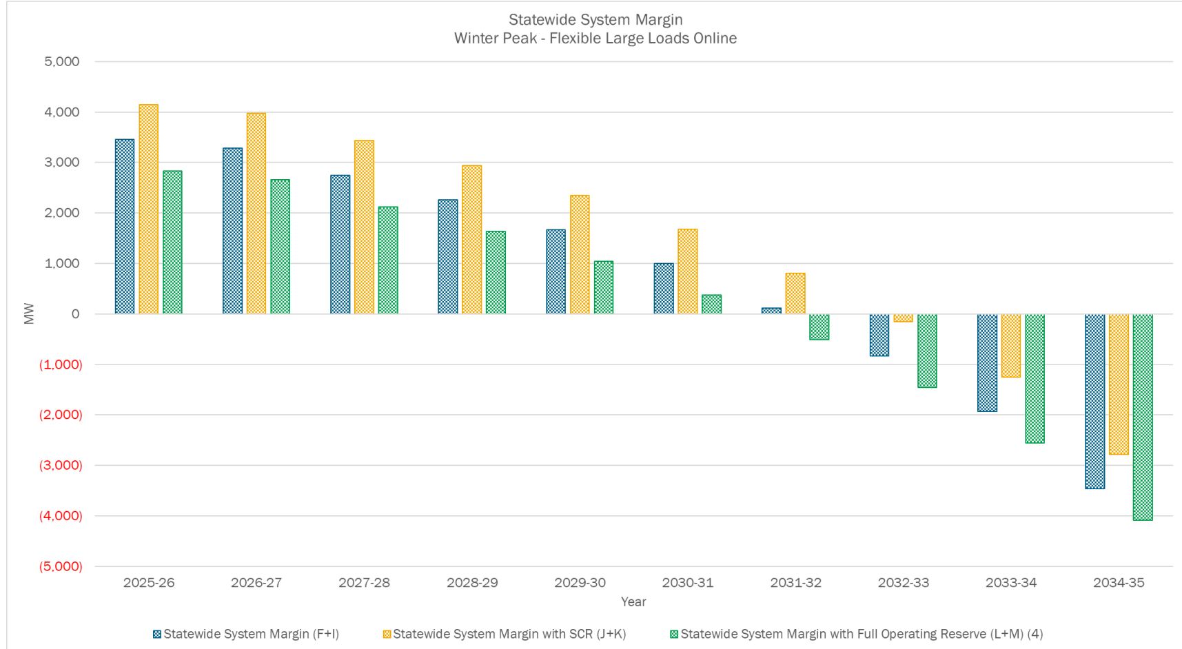
Figure 39: Winter Peak Statewide System Margin Chart (Flexible Large Loads Online)
