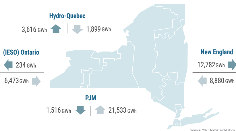
FIGURE 9: INTERREGIONAL IMPORTS AND EXPORTS: 2024
