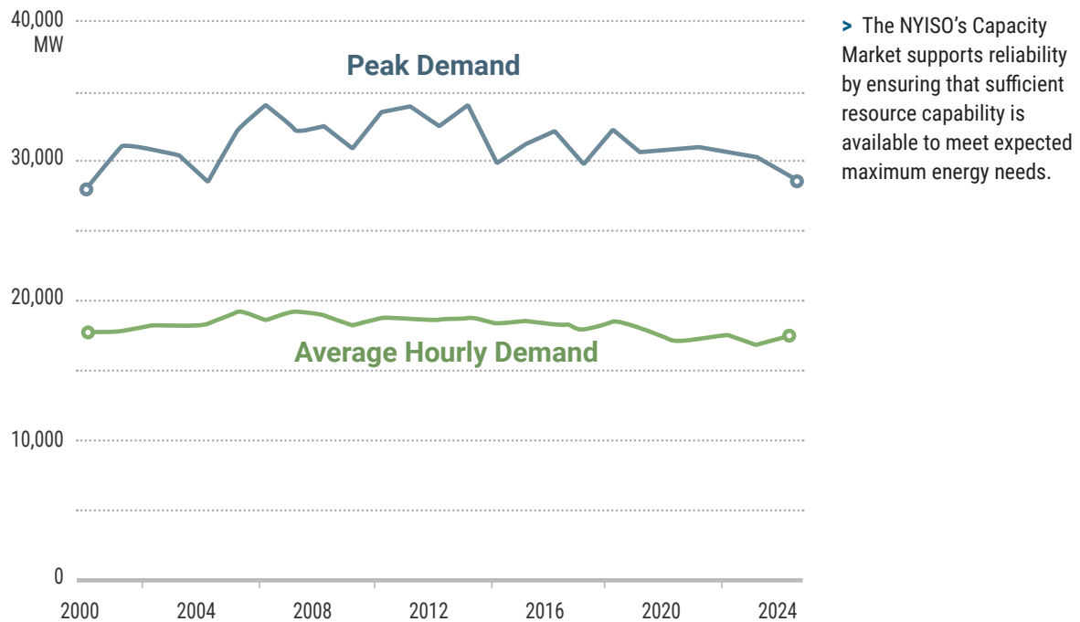
FIGURE 19: PEAK VS. AVERAGE HOURLY DEMAND
