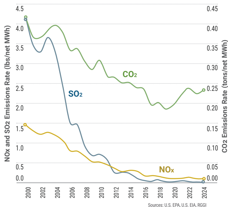
FIGURE 5: EMISSIONS RATES FROM ELECTRIC GENERATION IN NEW YORK: 2000-2024
