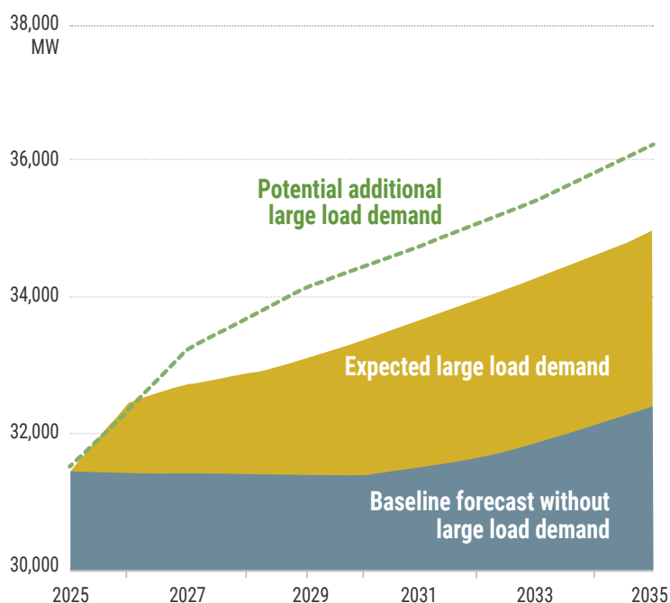
FIGURE 17: LARGE LOAD SUMMER DEMAND UNCERTAINTY
