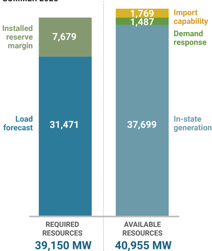
FIGURE 12: STATEWIDE RESOURCE AVAILABILITY: SUMMER 2025
