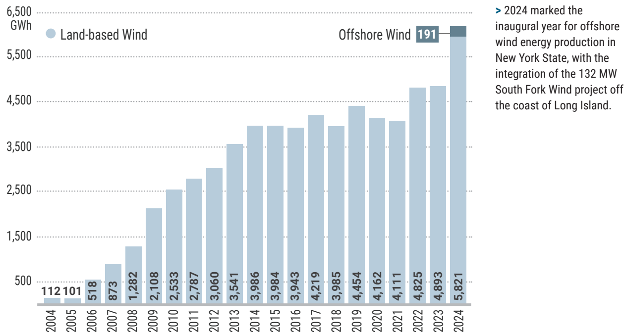
FIGURE 21: NEW YORK STATE WIND GENERATION: 2004-2024
