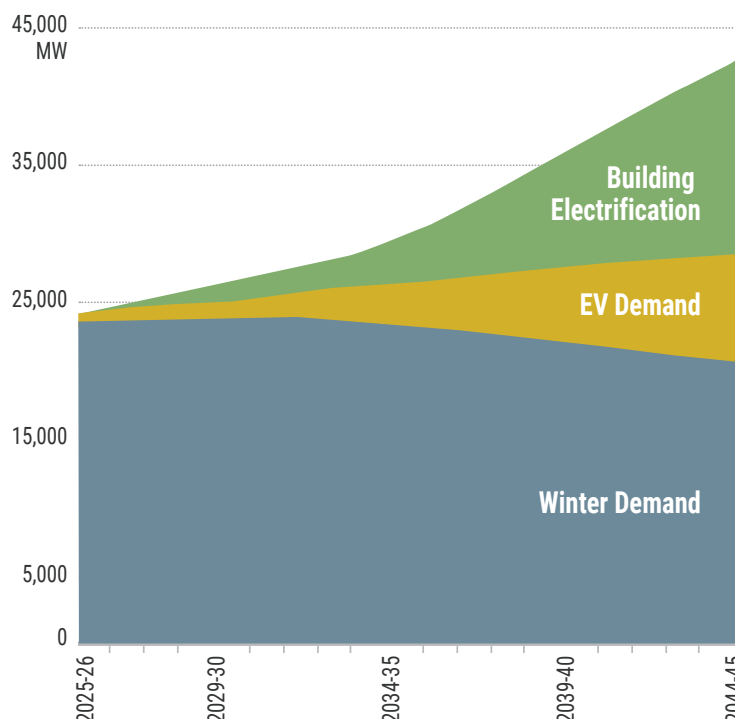
FIGURE 2: EXPECTED IMPACT OF ELECTRIFICATION ON STATEWIDE WINTER PEAK DEMAND
