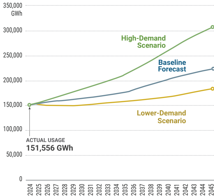
FIGURE 15: ACTUAL AND FORECAST LOAD: 2024-2045
