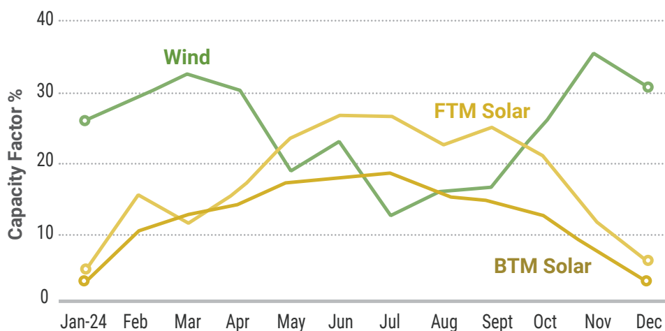
FIGURE 13: MONTHLY WIND AND SOLAR CAPACITY FACTORS
