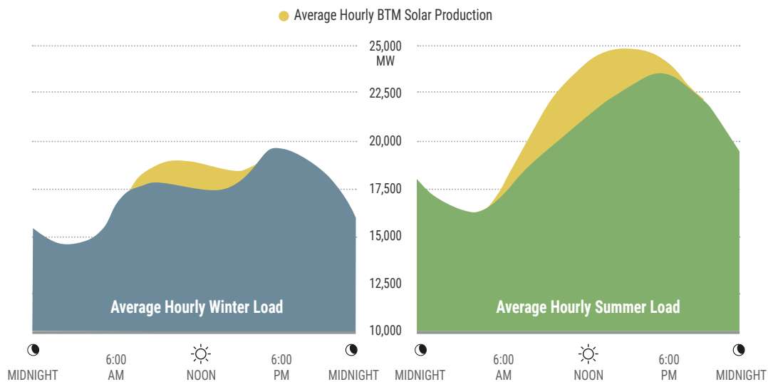
FIGURE 25: SUMMER AND WINTER BTM SOLAR PERFORMANCE
