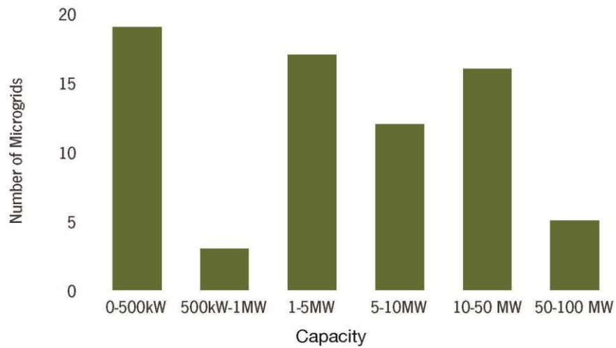
Figure 4-23. Operational Microgrid Capacity by Size Range
