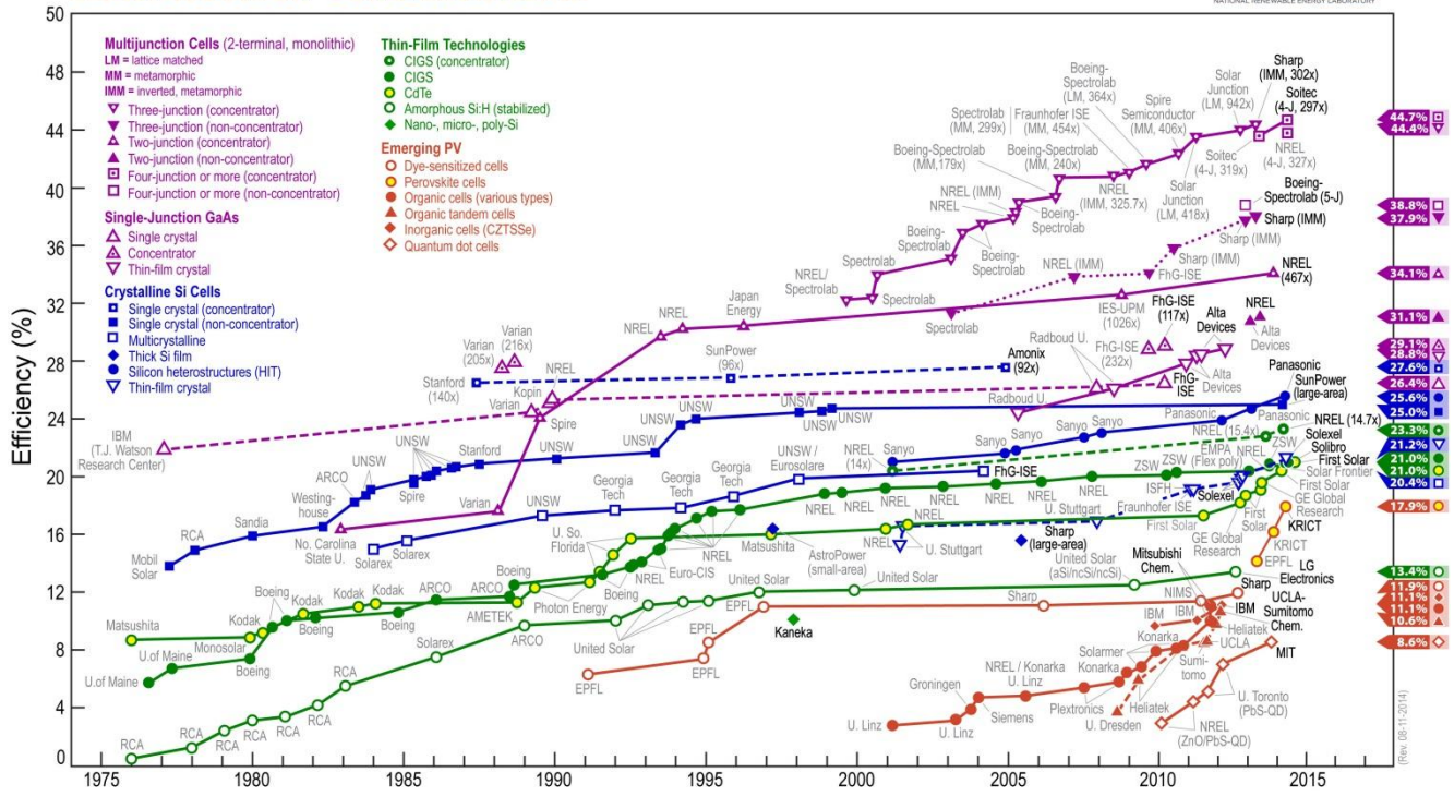
Figure 4-2. Solar Cell Efficiencies over Time
