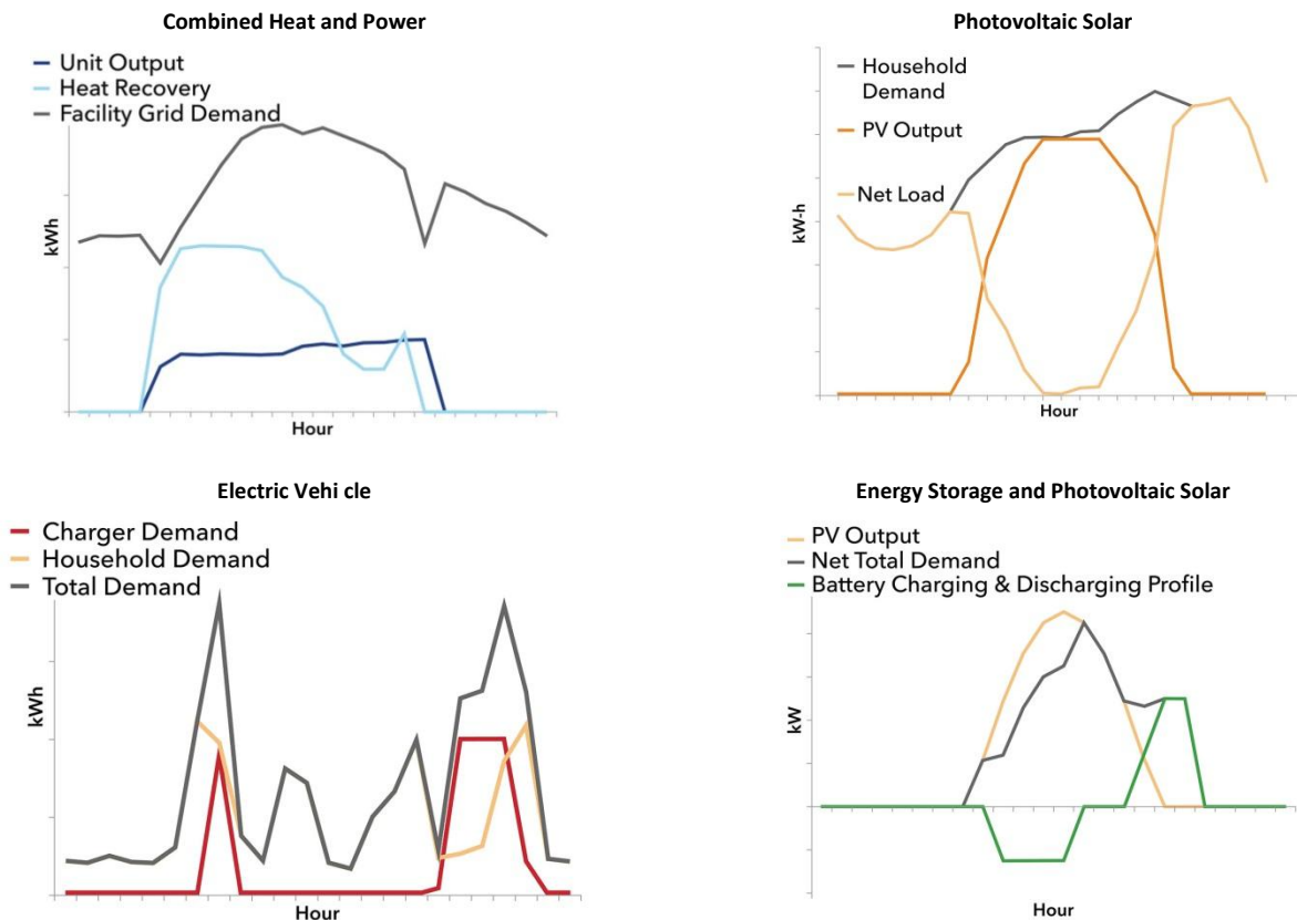
Figure 3-3. Sample DER Profiles by DER Type
