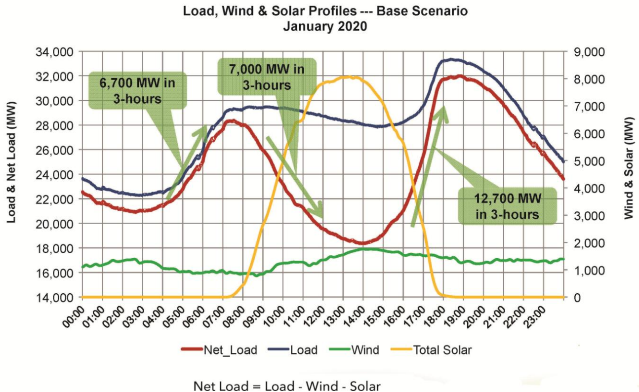
Figure 6-8. Load, Wind, and Solar Profiles: Base Scenario
