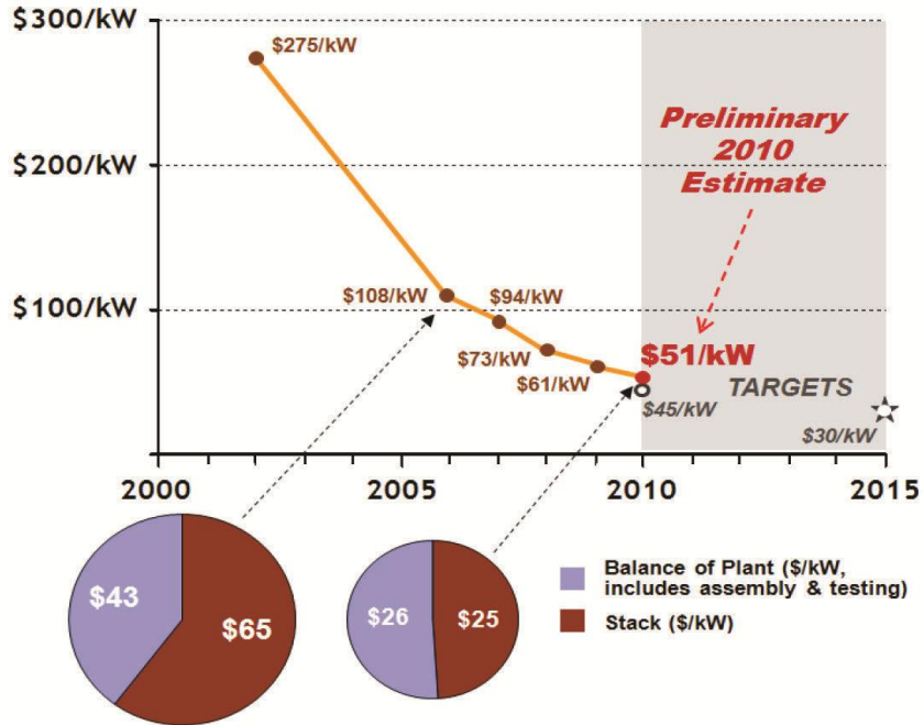
Figure 4-11. Projected Transportation Fuel Cell Costs
