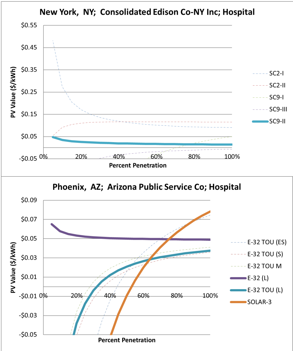
Figure 5-19. Variation in Value of PV by Tariff and Location for Two Sample Cases
