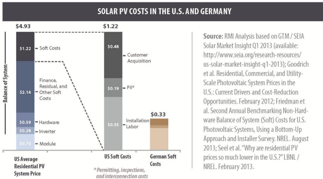
Figure 4-4. Solar PV System Costs in the U.S. and Germany
