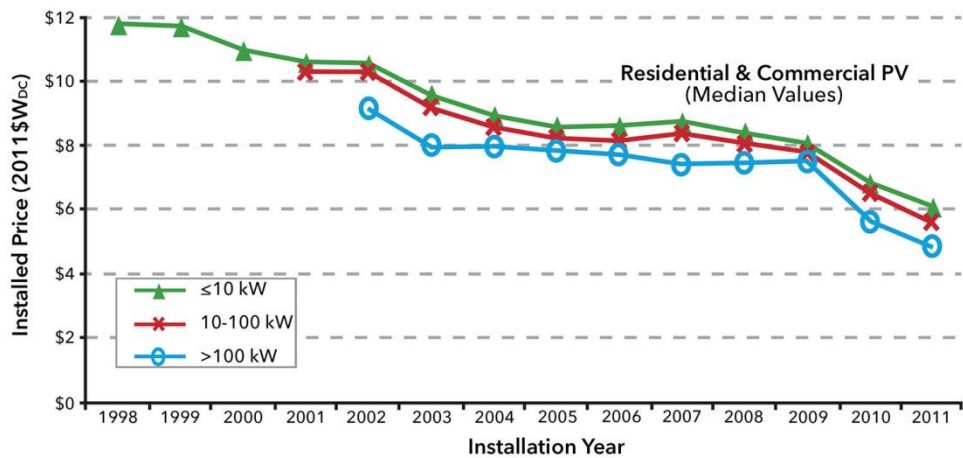
Figure 4-3. Installed Price of Residential & Commercial PV over Time
