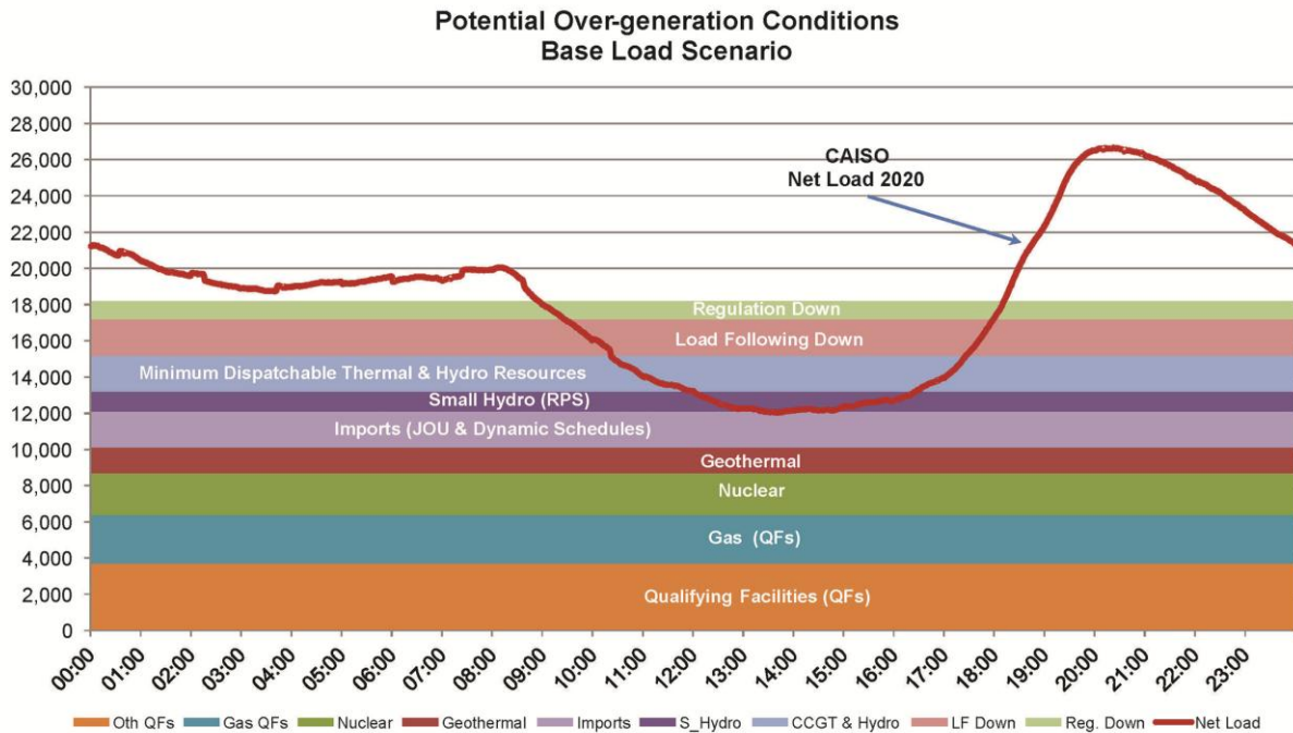
Figure 6-9. Potential Over-Generation Conditions: Base Load Scenario
