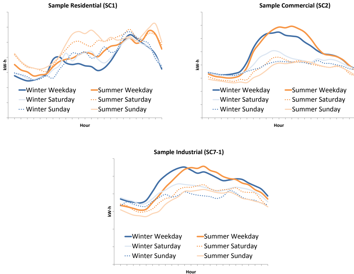
Figure 3-4. Sample Standard Load Profiles by Sector
