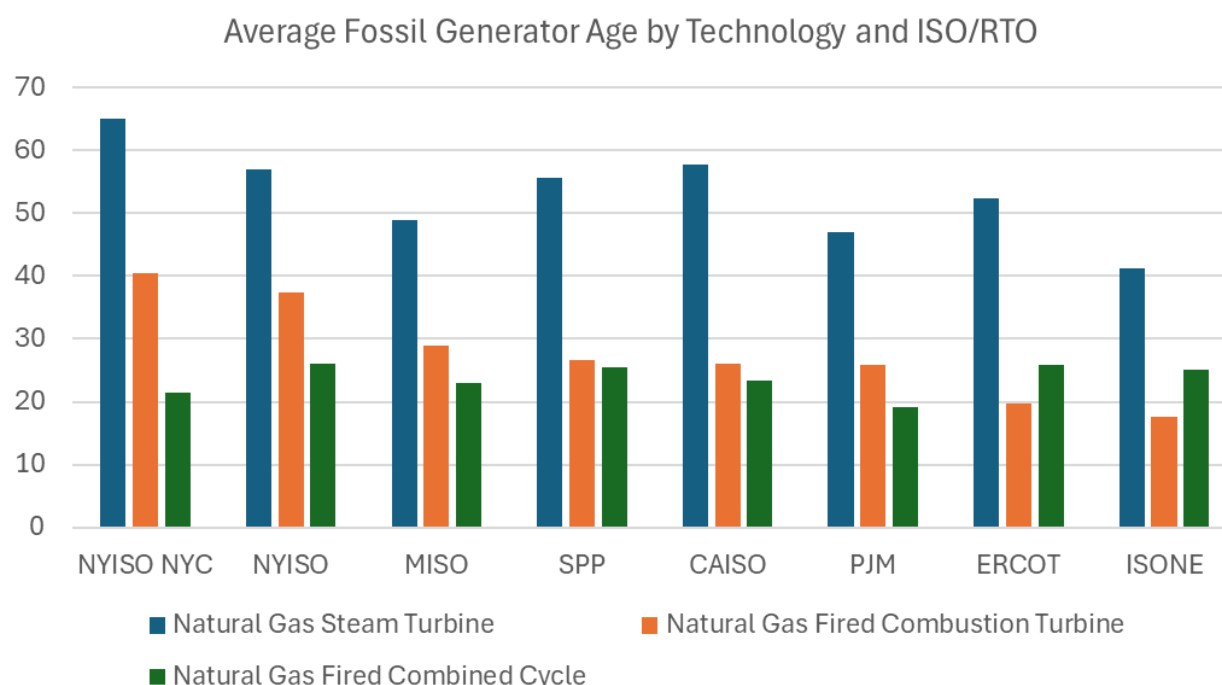
Figure 14: National Average Fossil Generator Age
