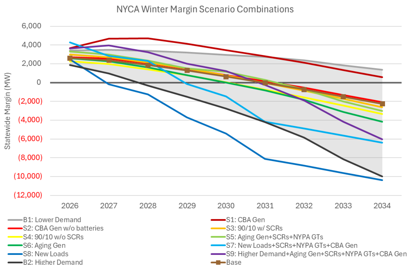
Figure 39: Winter Statewide System Margin Risks
