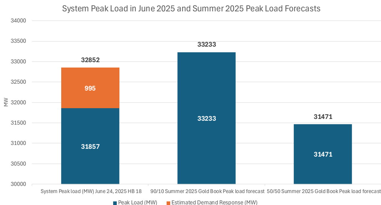
Figure 7: June Heatwave Load Comparison to Load Forecast
