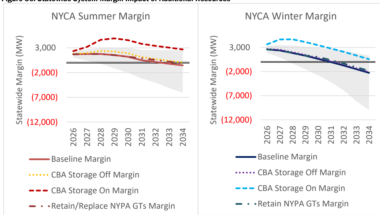
Figure 36: Statewide System Margin Impact of Additional Resources
