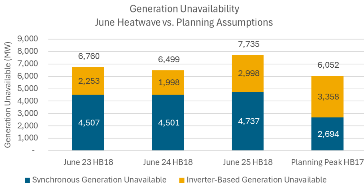
Figure 50: Generation Unavailability: June Heatwave vs. Planning Assumptions
