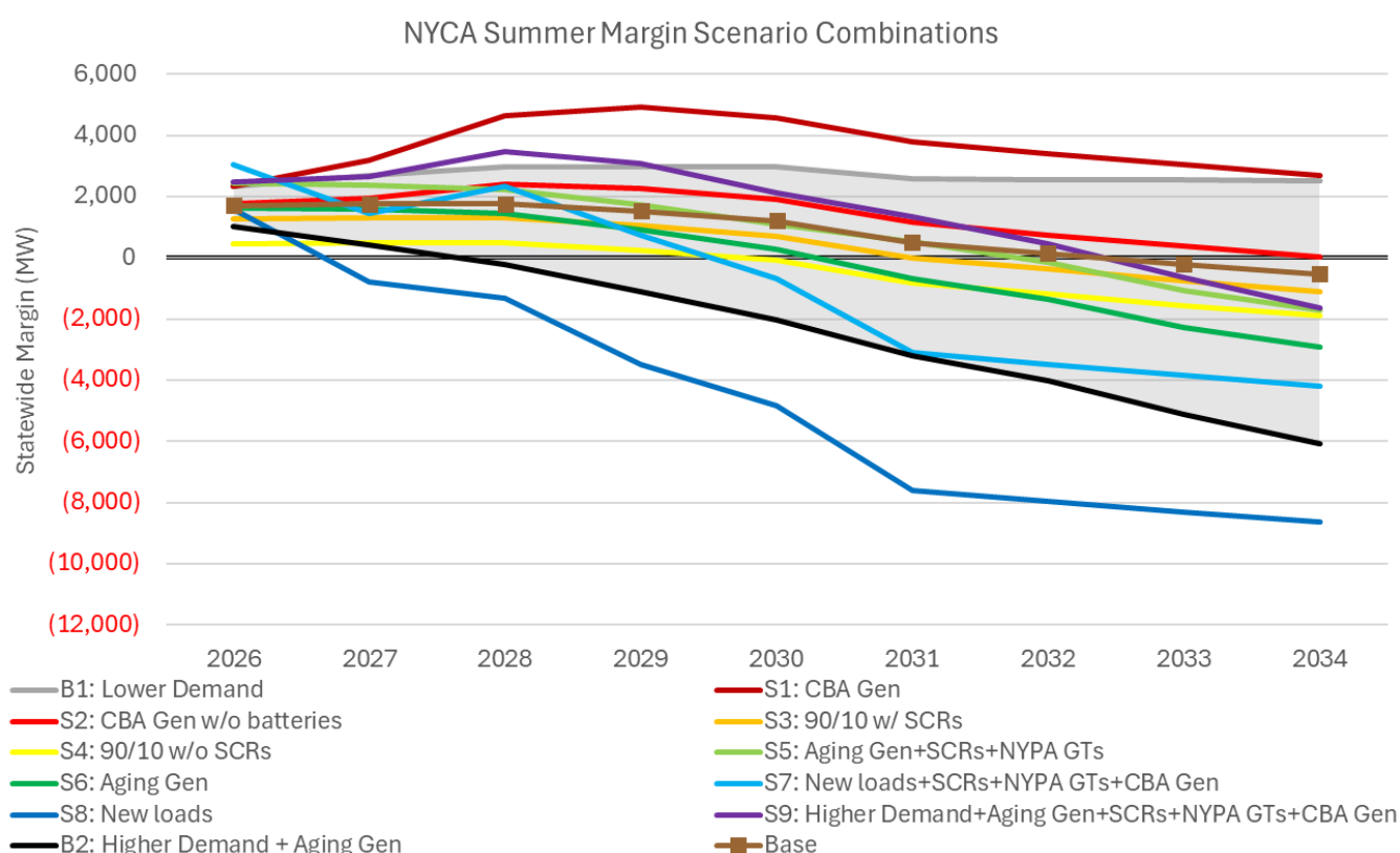
Figure 38: Summer Statewide System Margin Risks
