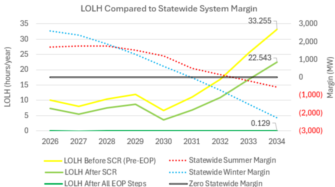
Figure 53: Comparison of LOLH and Statewide System Margin
