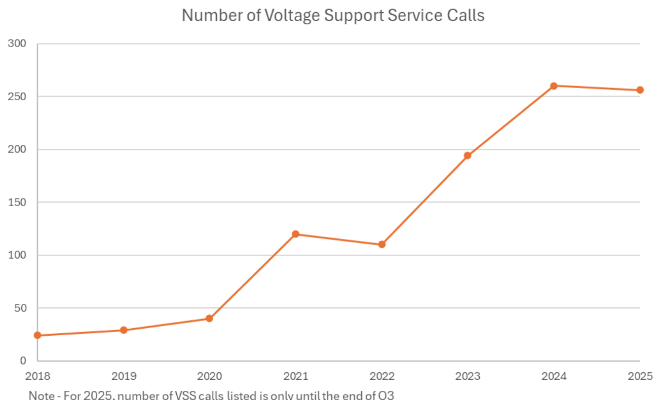
Figure 57: Number of Voltage Support Service Calls
