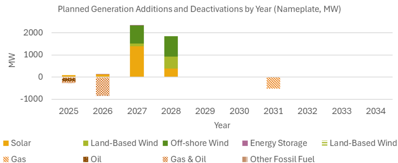
Figure 12: Planned Generation Additions and Deactivations by Year
