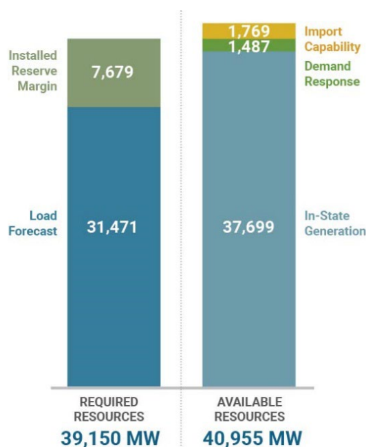
Figure 4: Statewide Resource Availability: Summer 2025
