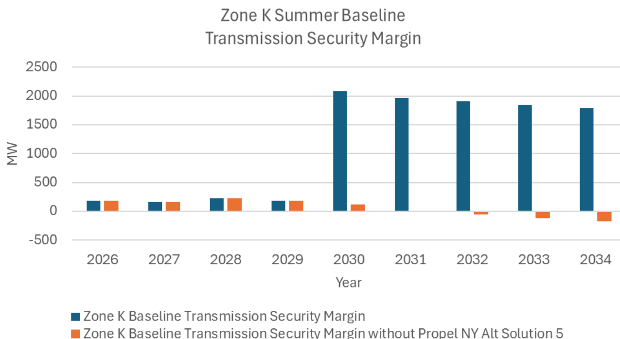
Figure 34: Zone K Transmission Security Margin with Impact of Project Delays
