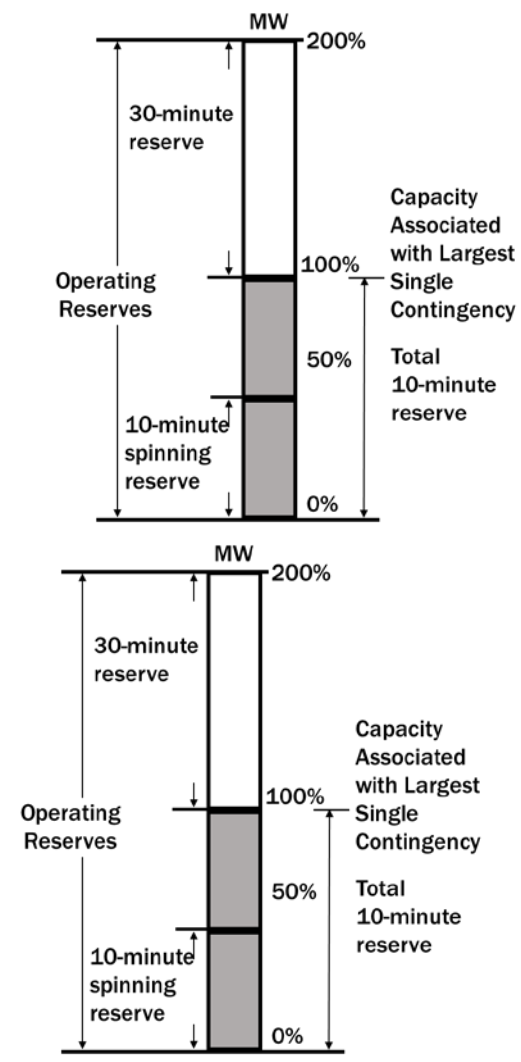
Figure 12: Minimum Operating Reserve Requirements
