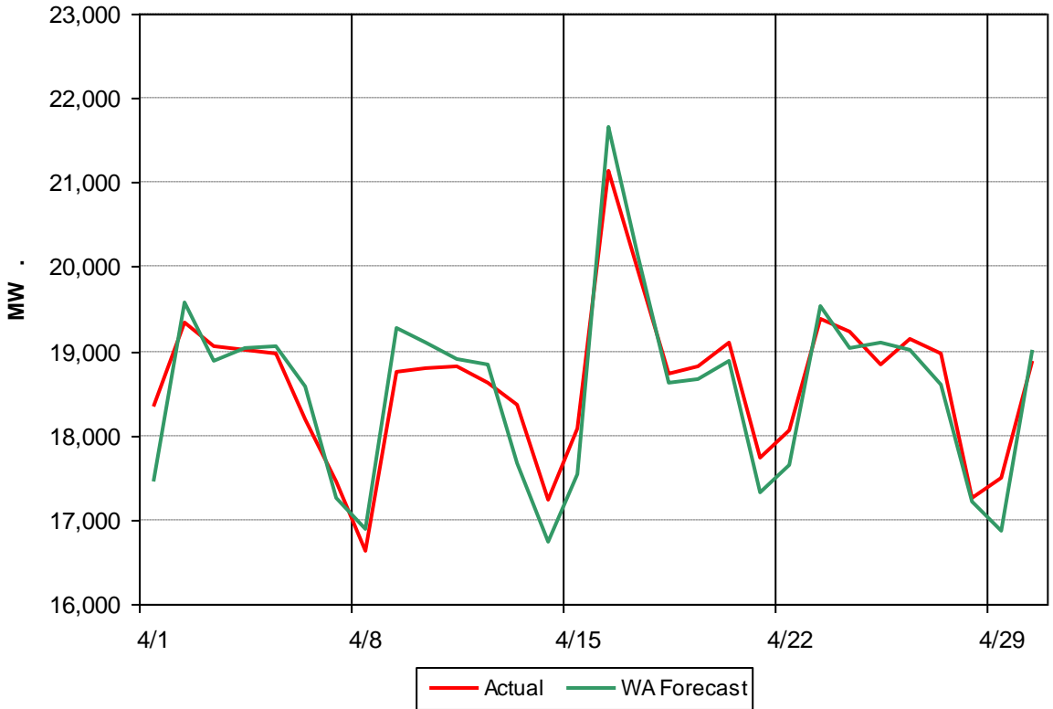
NYISO Daily Peak Load - April 2012 Actual vs Weather-Adjusted Forecast
