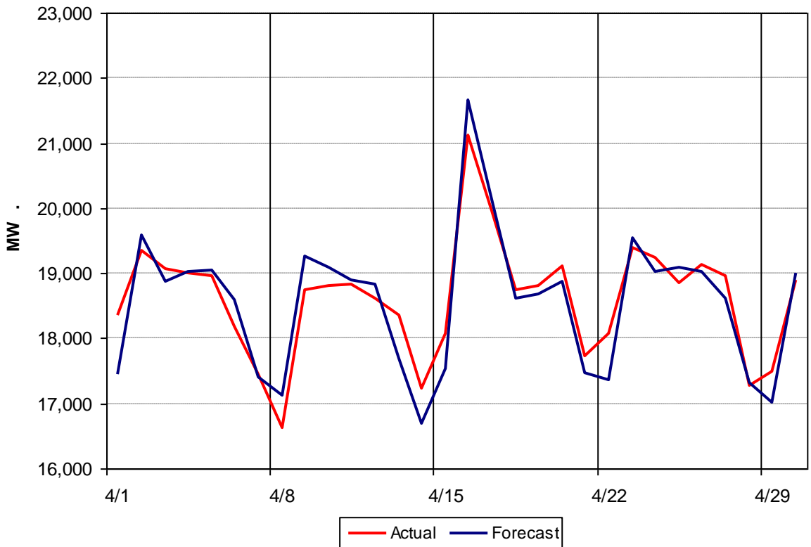
NYISO Daily Peak Load - April 2012 Actual vs Forecast
