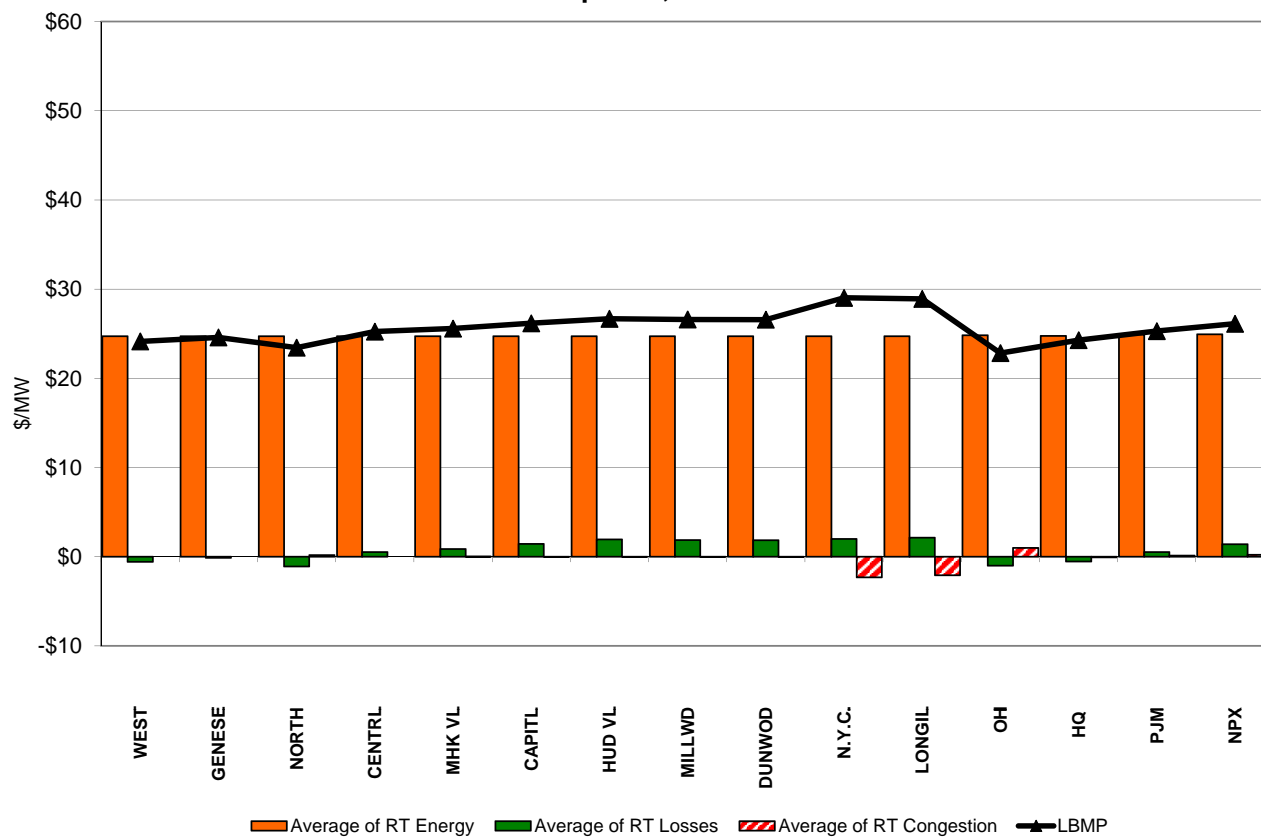
RT Zonal Unweighted Monthly Average LBMP Components thru April 30, 2012
