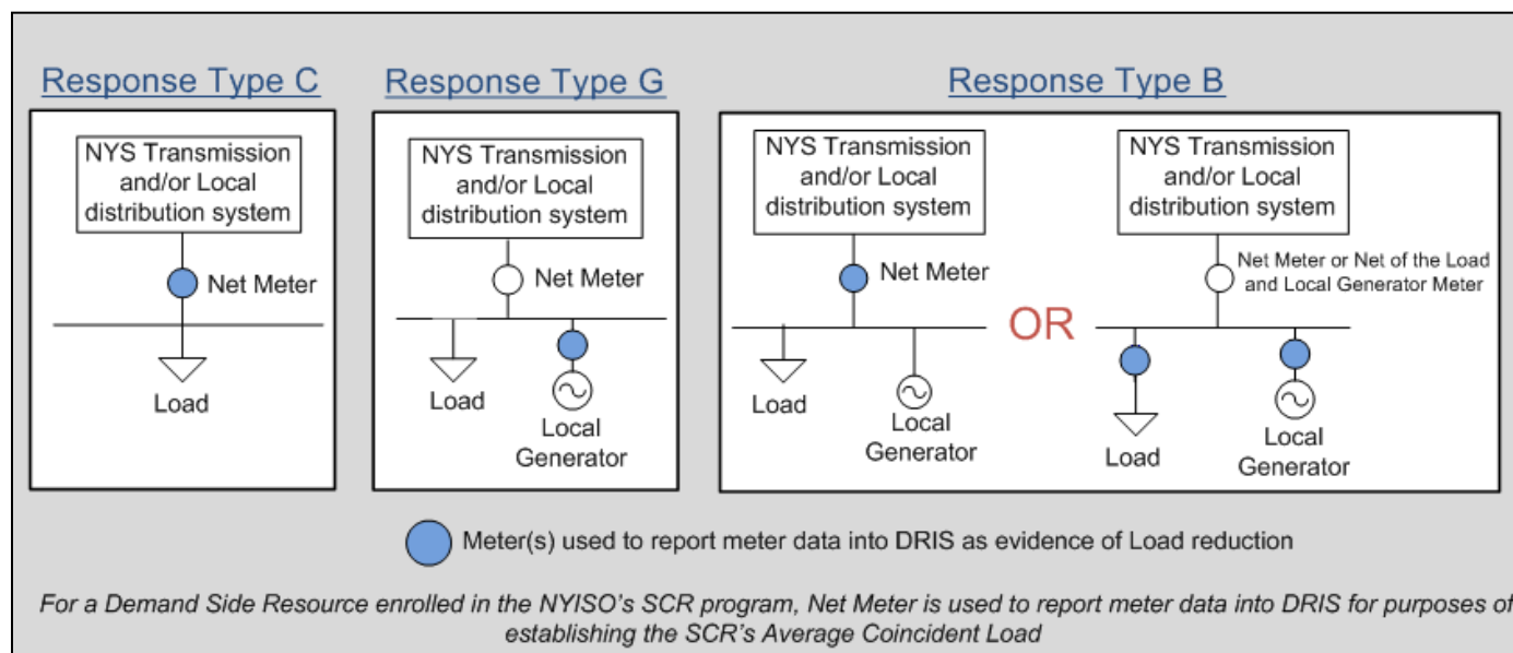
Figure 1: Examples of acceptable Meter Configurations
