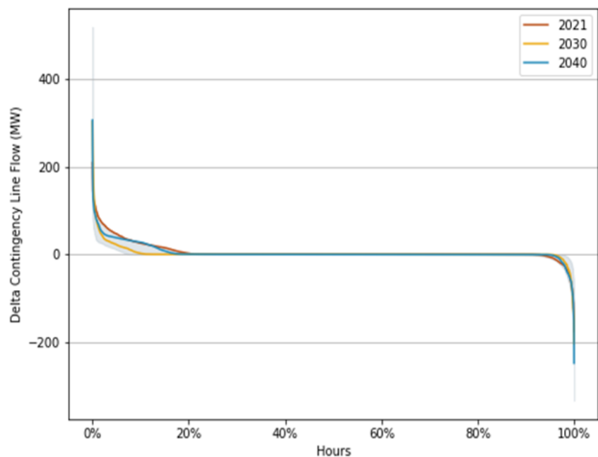
Figure 153153152: Dunwoodie-Motthaven Average Delta Flow
