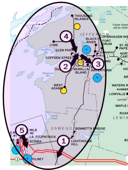
Figure 247247244: Pocket X3 Congestion and Energy Deliverability Summary(2030)
