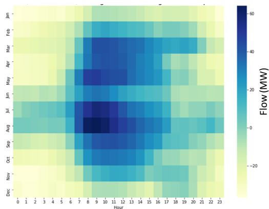
Figure 199199198: Sugarloaf-Ramapo Average Delta Flow (Contract-Baseline)
