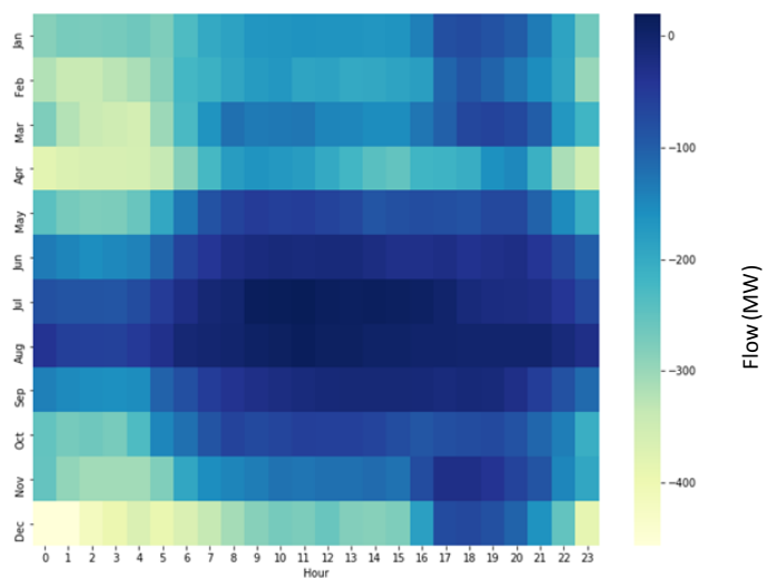
Figure 171171170: Dunwoodie-Long Island Average Delta Flow (Contract-Base)
