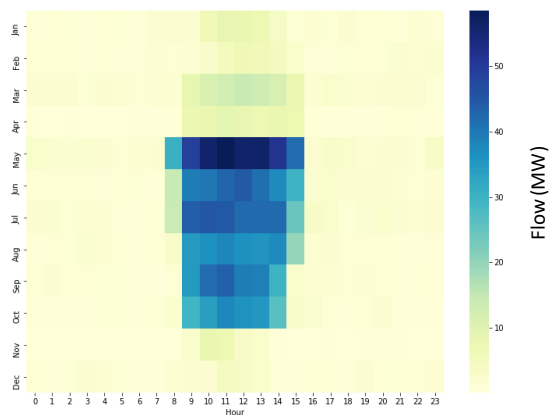
Figure 217217216: Golah-Mortimer Average Delta Flow (Relax-Contract)
