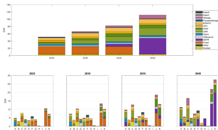
Figure 46: Scenario 1 Production Cost Capacity by Type by Zone
