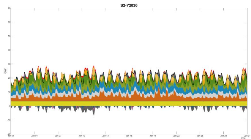
Figure 787877 : Scenario 2 2030 Winter Month Hourly Dispatch
