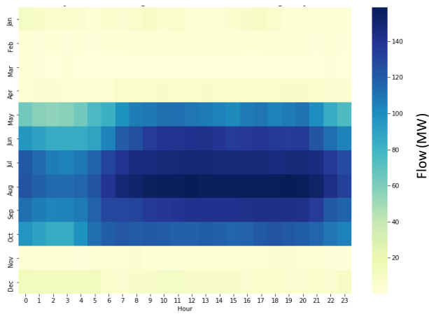
Figure 146146145 146145 : Volney-Scriba Average Delta Flow
