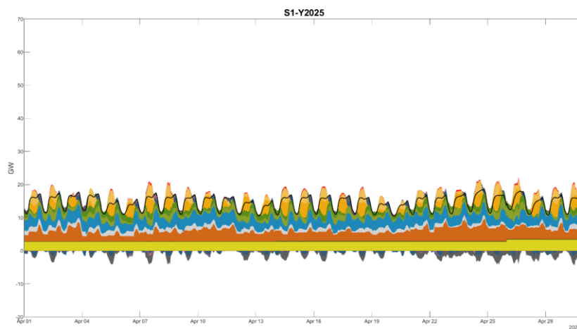
Figure 626261: Scenario 1 2025 Spring Month Hourly Dispatch
