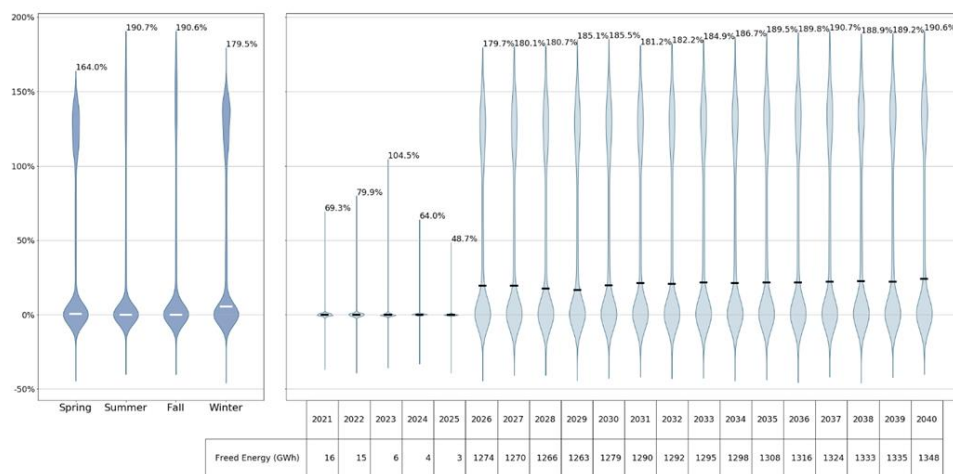
Figure 210210209: Barrett-Valley Stream Delta Hourly Line Utilization
