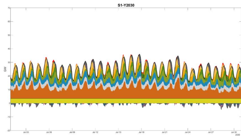
Figure 646463: Scenario 1 2030 Summer Month Hourly Dispatch
