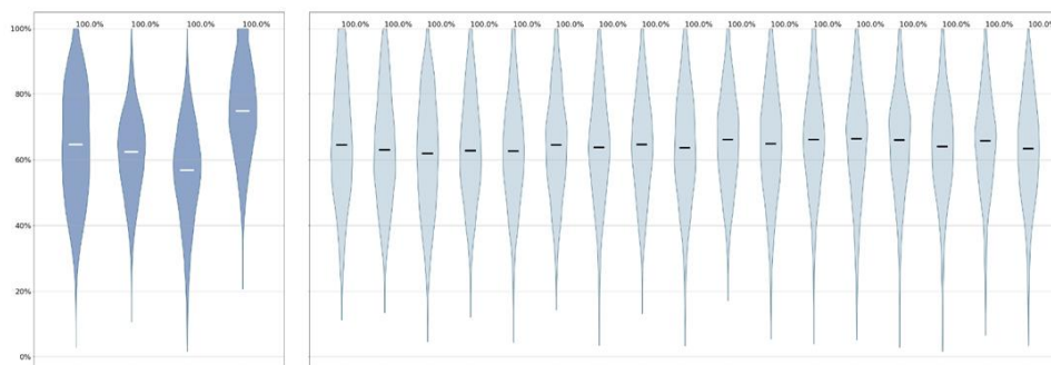
Figure 157157156: New Scotland-Knickerbocker Projected Baseline Hourly Line Utilization
