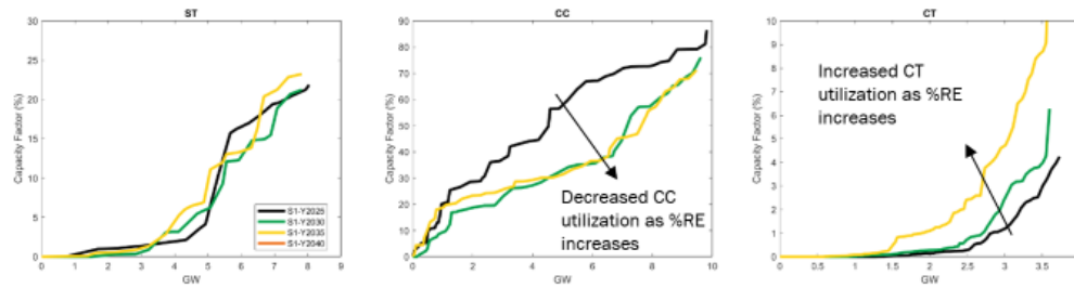
Figure 858584: Fossil Fleet Cumulative Capacity Curve: Unit Level Capacity Factors
