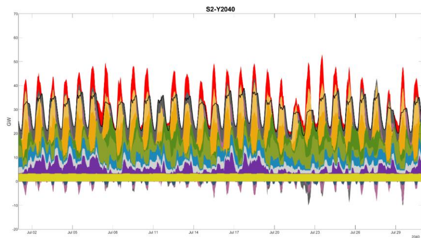
Figure 828 8281 : Scenario 2 2040 Summer Month Hourly Dispatch
