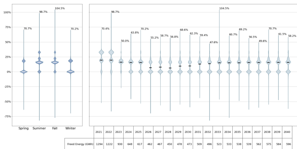
Figure 174174173: Dunwoodie-Long Island Delta Hourly Line Utilization (Relax-Contract)
