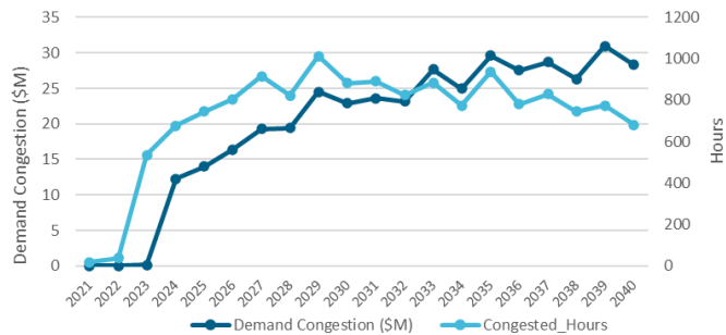
Figure 220220219: Stoner-Rotterdam Contract Case Projected Demand Congestion and Congested Hour
