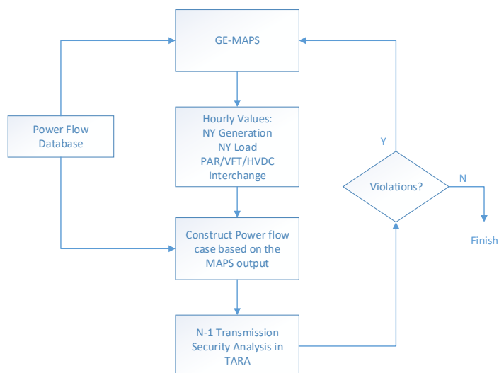
Figure 25 Figure 25 shows the flowchart for Roundtrip MAPS/TARA Analysis. This iterative analysis has three steps:
