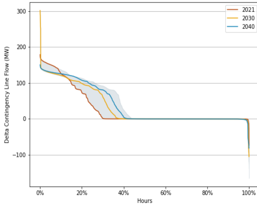
Figure 146146145 146145 : Volney-Scriba Average Delta Flow
