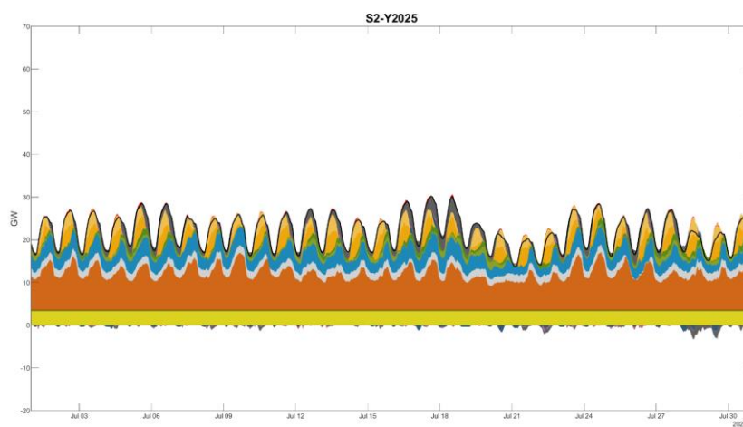
Figure 737372: Scenario 2 2025 Summer Month Hourly Dispatch
