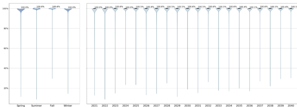
Figure 137 Dunwoodie to Long Island Baseline Case Hourly Line Utilization
