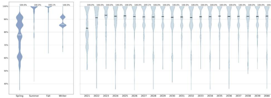
Figure 144144143: Volney-Scriba Baseline Case Hourly Line Utilization
