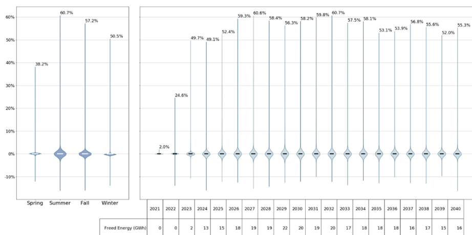
Figure 218218217: Golah-Mortimer Delta Hourly Line Utilization
