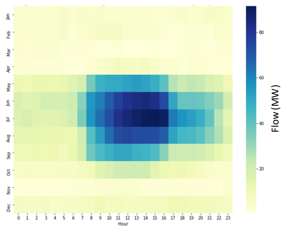
Figure 201201200 202202201 : Sugarloaf-Ramapo Average Delta Flow (Relax-Contract)
