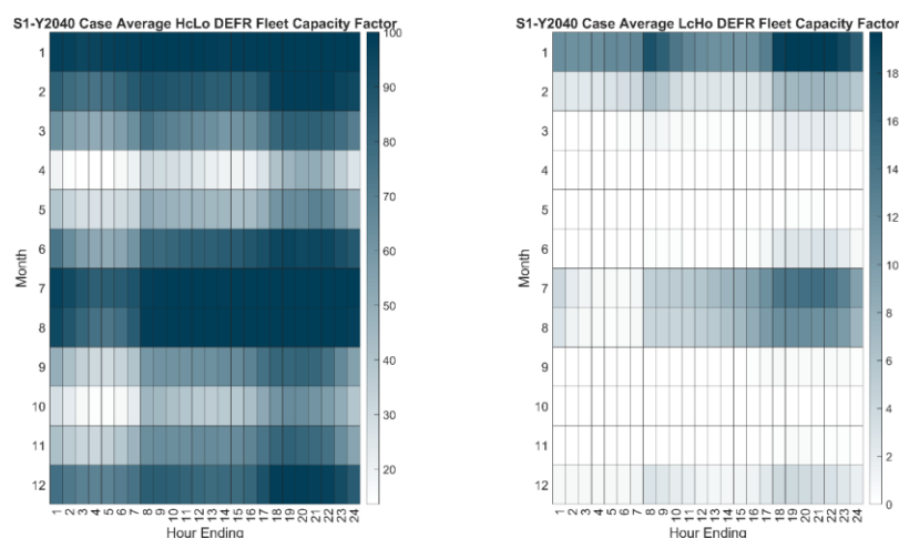
Figure 929291: Average DEFR Fleet Capacity Factor by Month and Hour: 2040 S1
