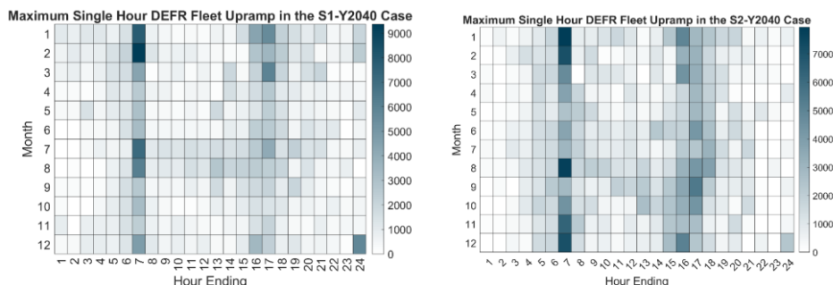
Figure 939392: Maximum DEFR Fleet Up-Ramp (MW/hour) by Month and Hour: 2040 S1 and S2
