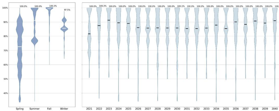
Figure 176176175: Volney-Scriba Contract Case Hourly Line Utilization
