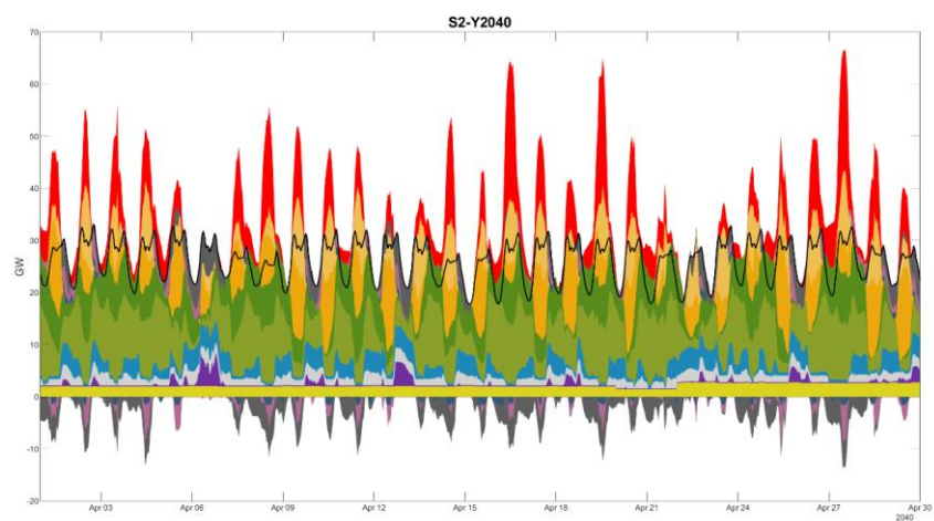
Figure 838382 : Scenario 2 2040 Spring Month Hourly Dispatch
