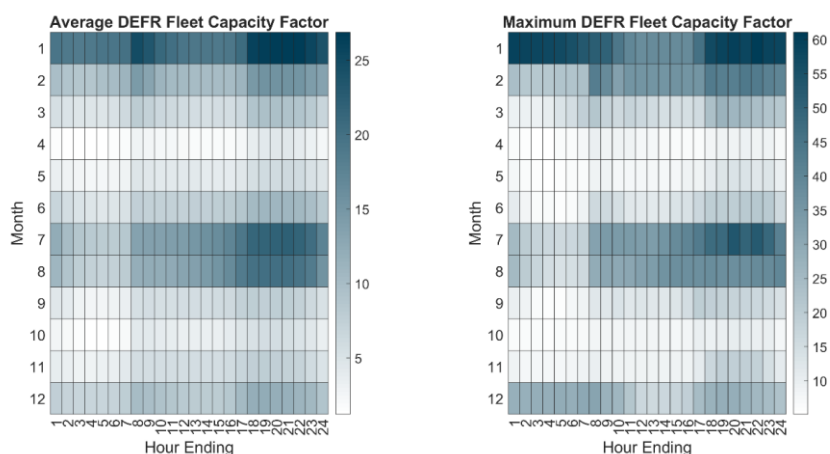
Figure 909089: Average and Maximum DEFR Fleet Capacity Factors by Month and Hour: 2040 S1
