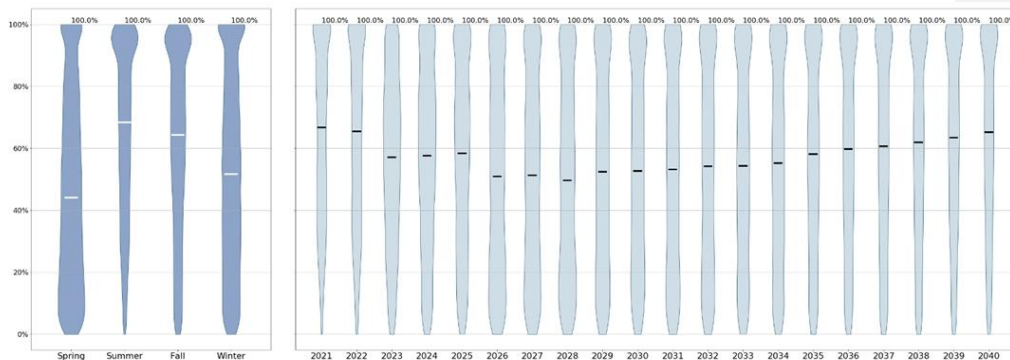
Figure 183183182: Dunwoodie-Motthaven Contract Case Hourly Line Utilization
