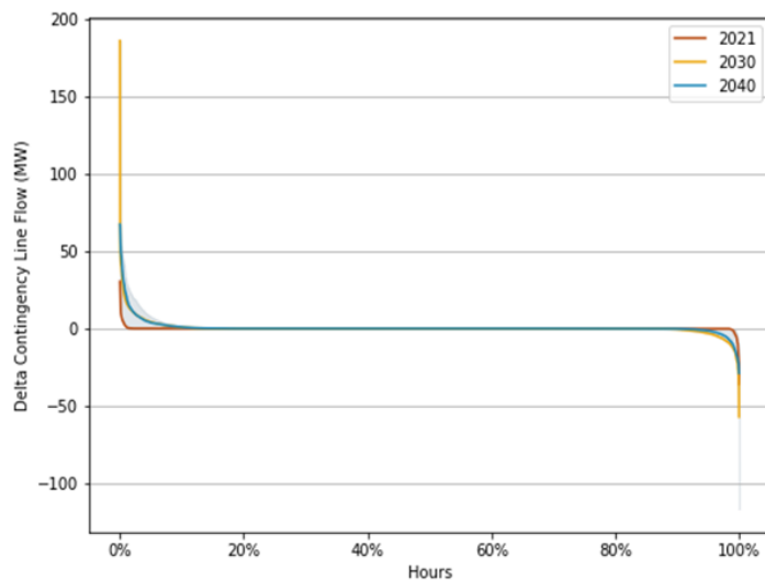
Figure 165165164: Sugarloaf-Ramapo Average Delta Flow
