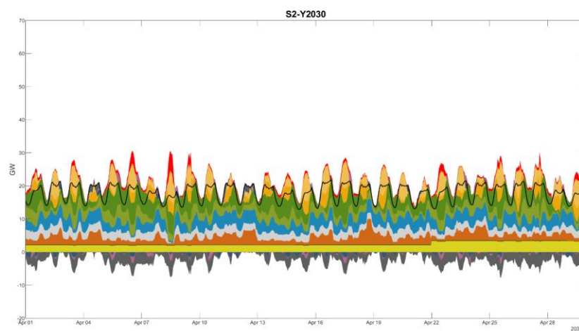
Figure 777776 : Scenario 2 2030 Spring Month Hourly Dispatch
