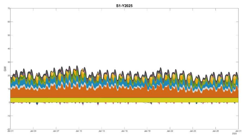
Figure 636362: Scenario 1 2025 Winter Month Hourly Dispatch
