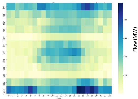
Figure 153153152: Dunwoodie-Motthaven Average Delta Flow
