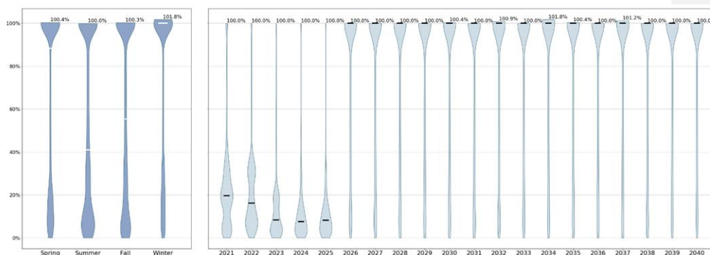
Figure 205205204: Barrett-Valley Stream Contract Case Hourly Line Utilization
