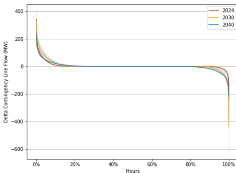
Figure 158158157: New Scotland-Knickerbocker Delta Flow Duration Curves (Relax-Baseline)
