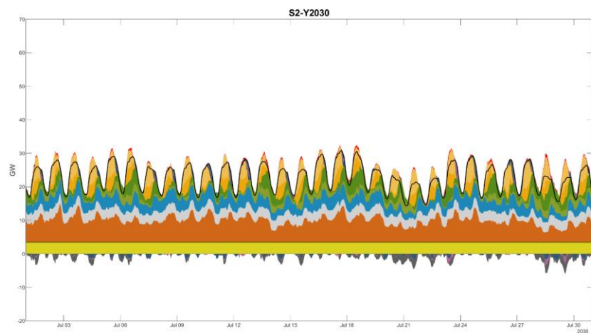
Figure 7676 75: Scenario 2 2030 Summer Month Hourly Dispatch
