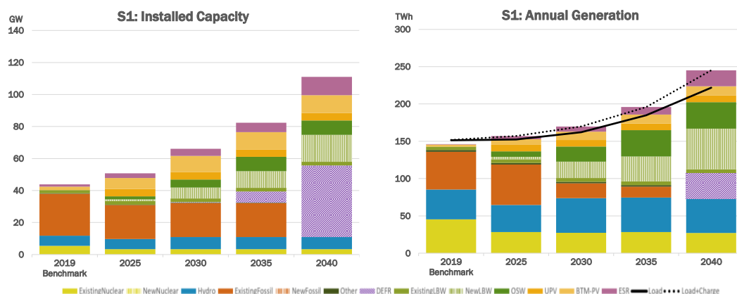
Figure 44: S1 Capacity and Generation Results
