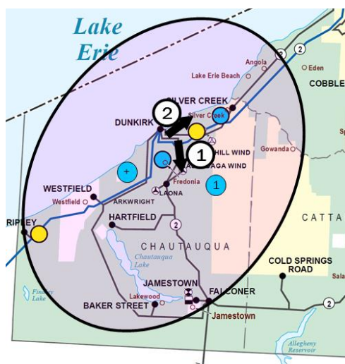
Figure 241241238: Pocket W3 Congestion and Energy Deliverability Summary (2030)
