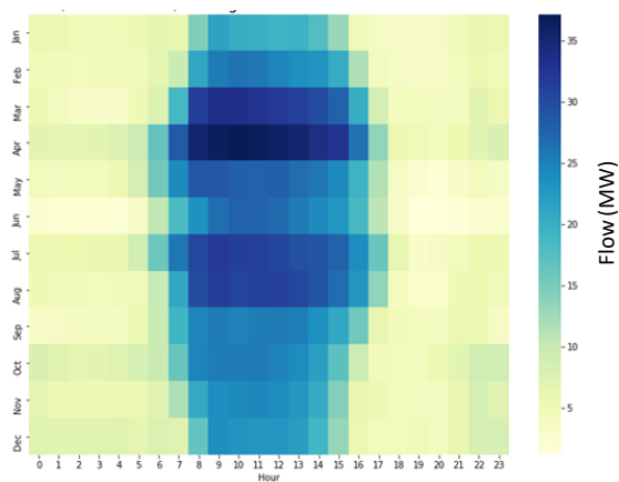
Figure 223223222: Stoner-Rotterdam Average Delta Flow (Contract-Baseline)
