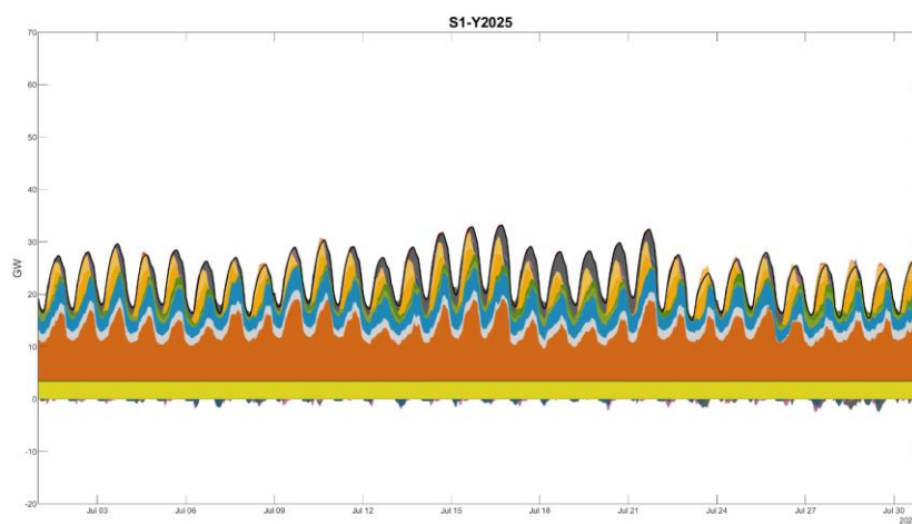
Figure 616160: Scenario 1 2025 Summer Month Hourly Dispatch
