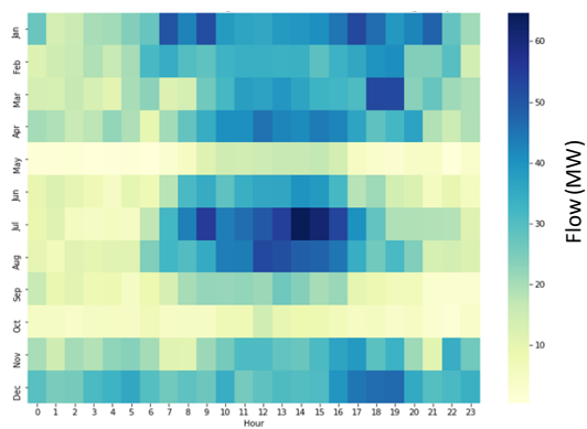
Figure 187187186: Dunwoodie-Motthaven Average Delta Flow (Relax-Contract)
