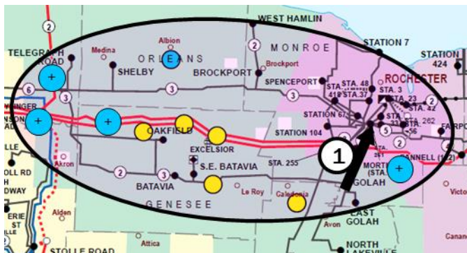
Figure 237237234: Pocket W1 Congestion and Energy Deliverability Summary (2030)
