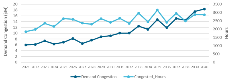
Figure 143143142: Volney-Scriba Baseline Projected Demand Congestion and Congested Hours
