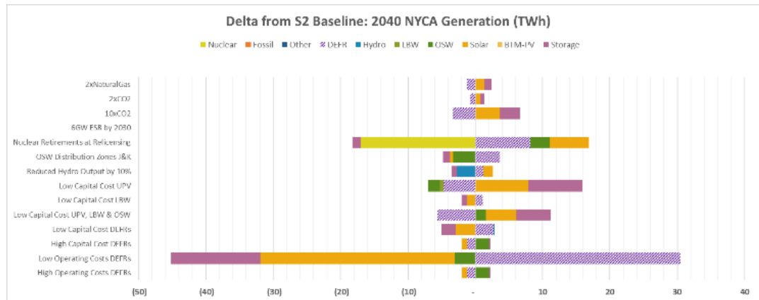
Figure 10010999 : Policy Case S2 Scenario Annual Generation Change in 2040
