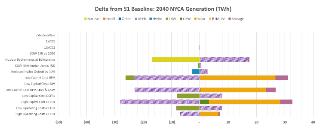
Figure 10010999 : Policy Case S2 Scenario Annual Generation Change in 2040
