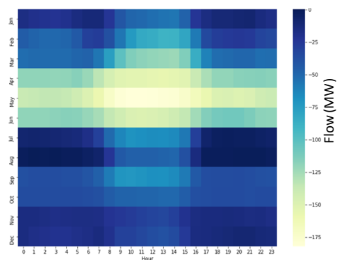
Figure 178178177: Volney-Scriba Average Delta Flow (Contract-Baseline)
