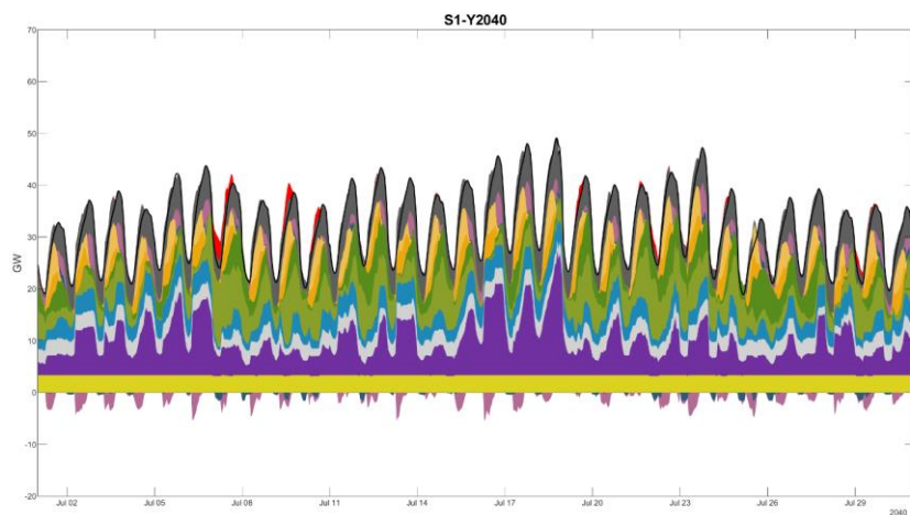
Figure 707069 : Scenario 1 2040 Summer Month Hourly Dispatch
