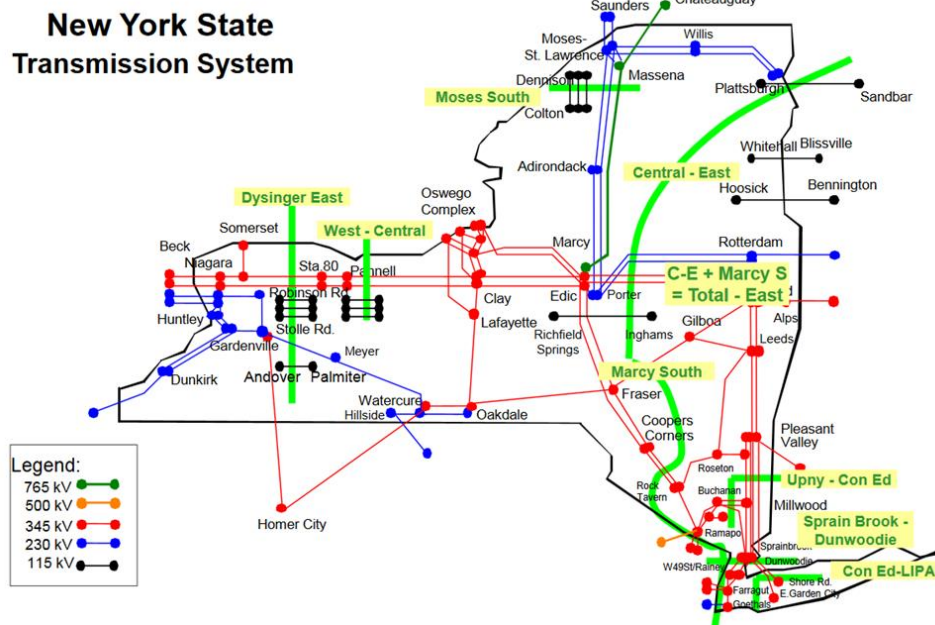
Figure 6: NYISO 115 kV and Above Transmission Map
