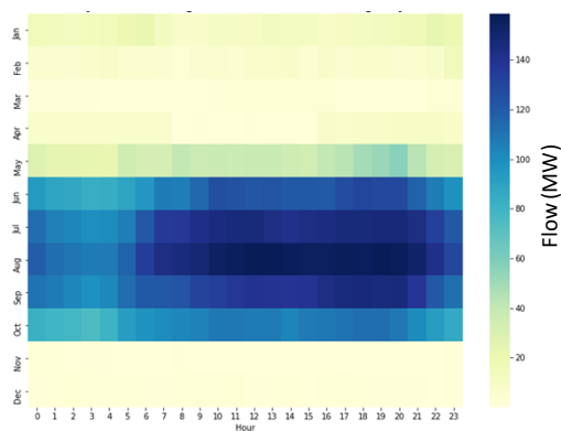
Figure 180180179: Volney-Scriba Average Delta Flow (Relax-Contract)
