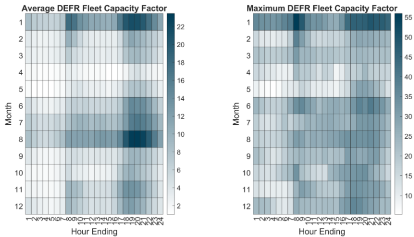
Figure 919190: Average and Maximum DEFR Fleet Capacity Factors by Month and Hour: 2040 S2
