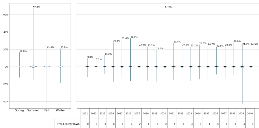
Figure 166166165: Sugarloaf-Ramapo Delta Hourly Line Utilization
