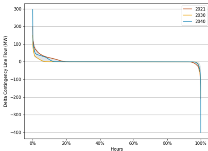
Figure 187187186: Dunwoodie-Motthaven Average Delta Flow (Relax-Contract)
