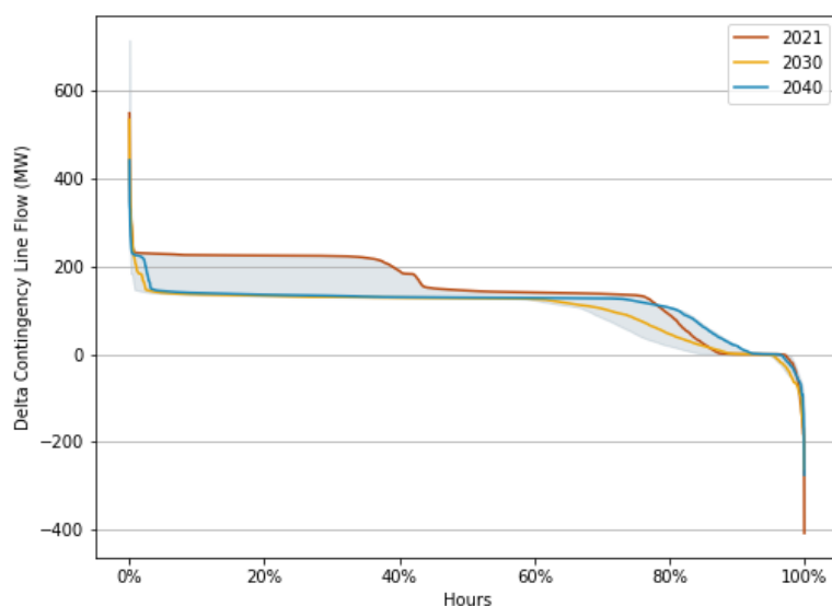
Figure 138: Dunwoodie-Long Island Flow Duration Curve (Relax-Baseline)
