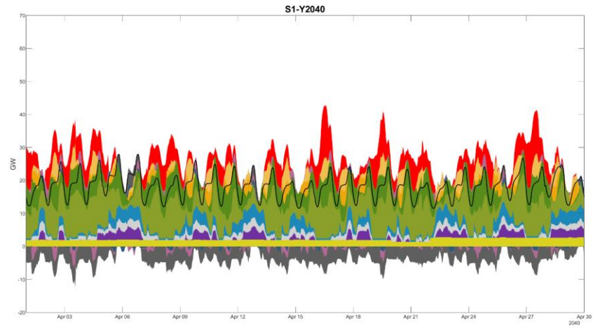
Figure 717170 727271 : Scenario 1 2040 Spring Month Hourly Dispatch
