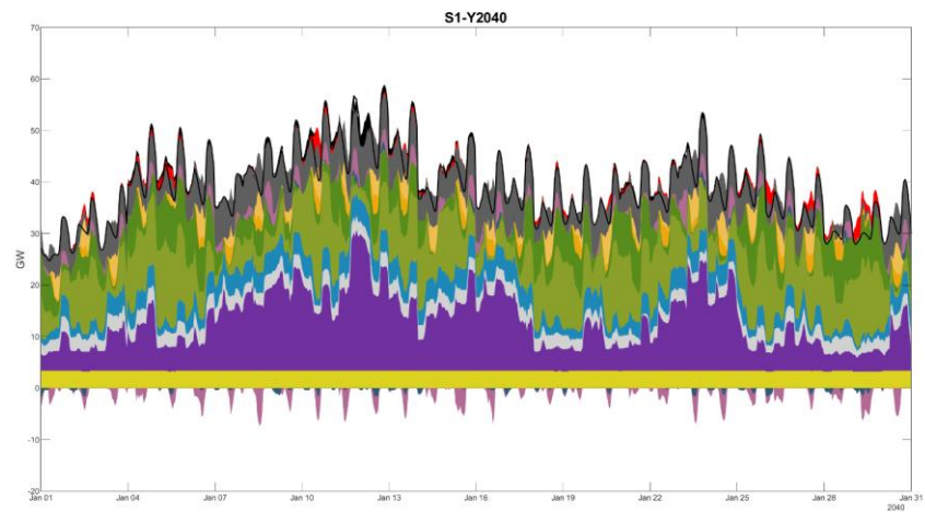
Figure 727271 727271 : Scenario 1 2040 Winter Month Hourly Dispatch
