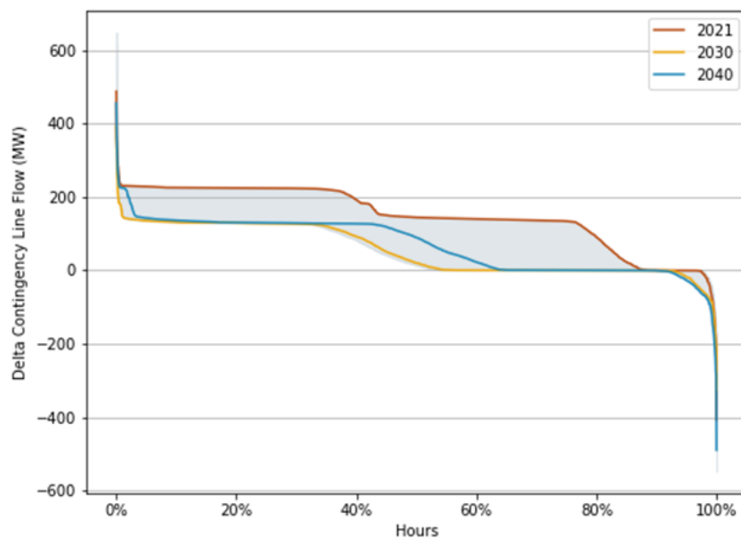
Figure 173173172: Dunwoodie-Long Island Average Delta Flow
