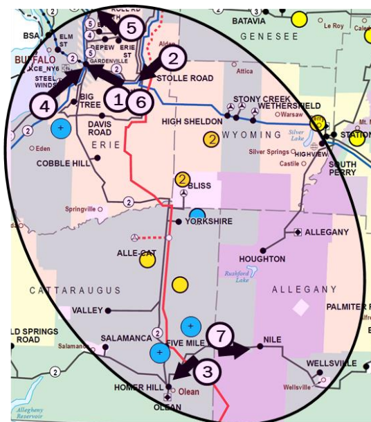
Figure 240240237: Pocket W2 Congestion and Energy Deliverability Summary (2035)
