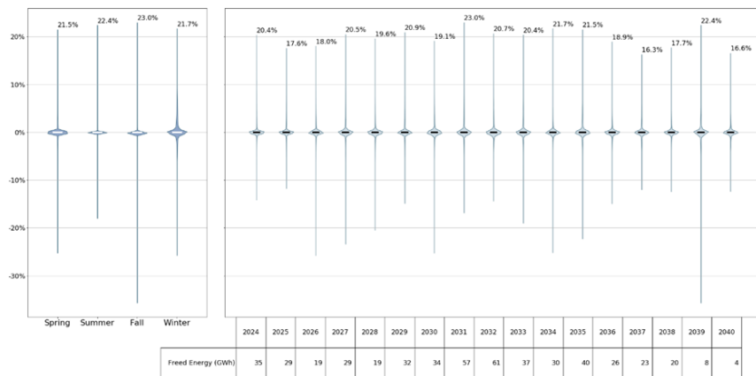
Figure 160160159: New Scotland-Knickerbocker Delta Hourly Line Utilization
