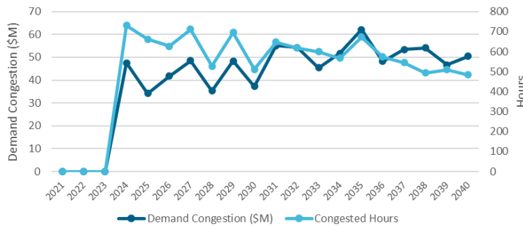
Figure 189189188: New Scotland-Knickerbocker Contract Case Projected Demand Congestion and Congested Hours
