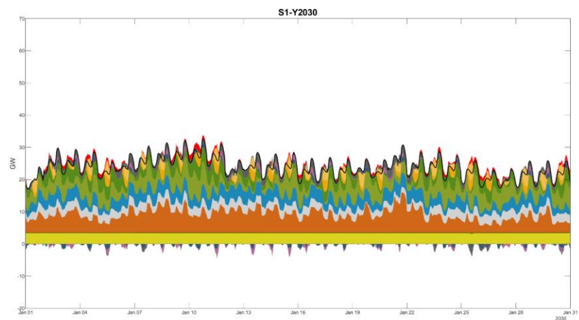
Figure 66665: Scenario 1 2030 Winter Month Hourly Dispatch
