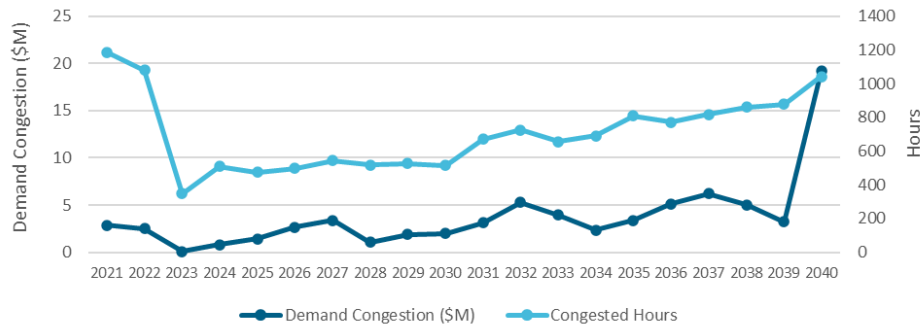
Figure 150150149: Dunwoodie-Motthaven Baseline Projected Demand Congestion and Congested Hours
