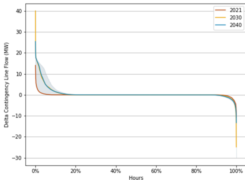
Figure 232232231: Jennison-Sidney Delta Flow Duration Curve (Relax-Contract)
