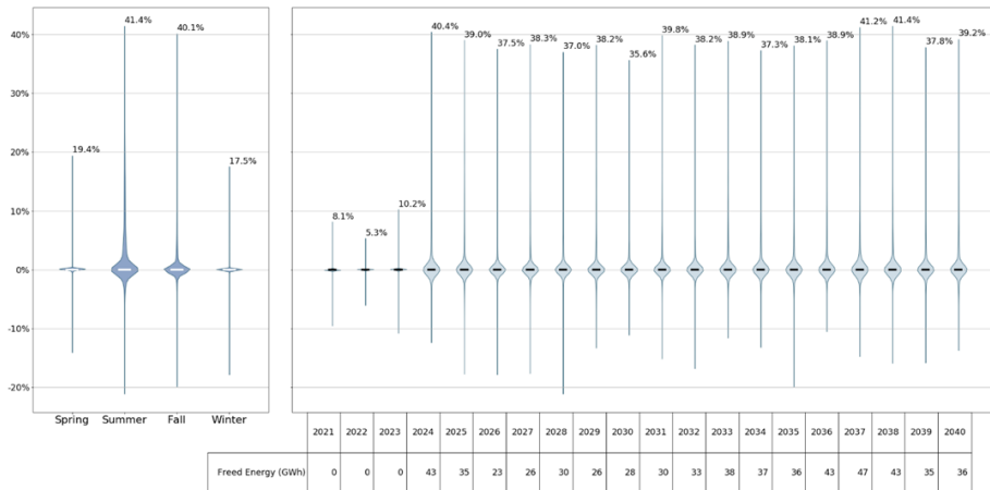
Figure 202202201 202202201 : Sugarloaf-Ramapo Delta Hourly Line Utilization
