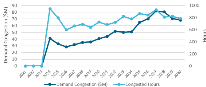
Figure 196196195: Sugarloaf-Ramapo Contract Case Projected Demand Congestion and Congested Hour
