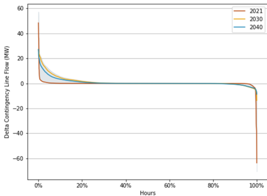
Figure 224224223: Stoner-Rotterdam Delta Flow Duration Curve (Relax-Contract)
