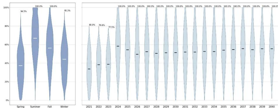
Figure 163163162: Sugarloaf-Ramapo Baseline Case Hourly Line Utilization
