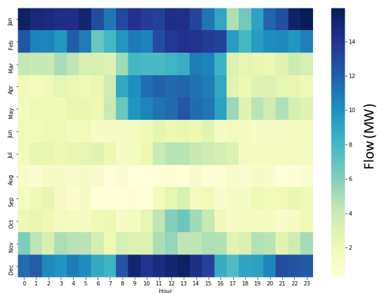
Figure 233233232: Jennison-Sidney Average Delta Flow
