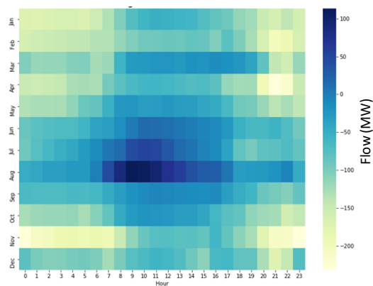
Figure 185185184: Dunwoodie-Motthaven Average Delta Flow (Contract-Baseline)
