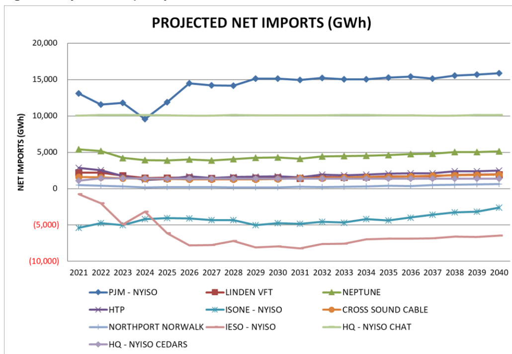
Figure 37: Projected Net Imports by Interface
