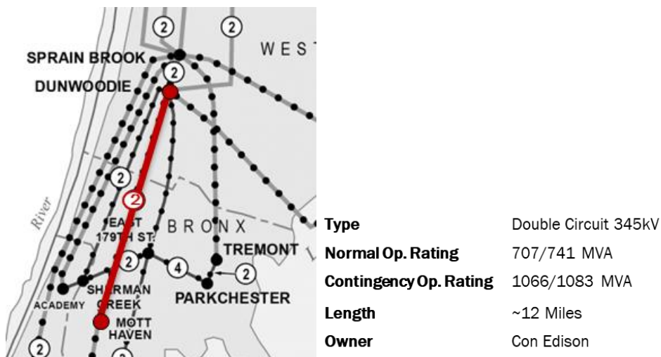
Figure 148: Dunwoodie-Motthaven 345 kV Line Location and Parameters
