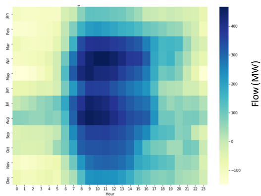
Figure 192192191 191: New Scotland-Knickerbocker Average Delta Flow
