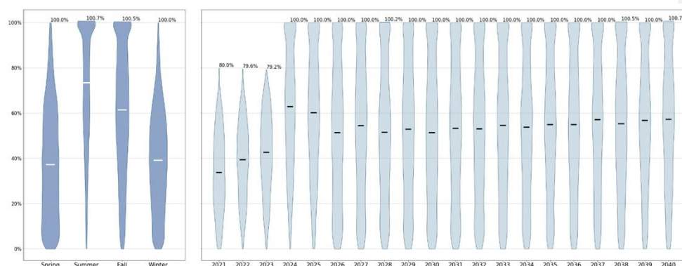
Figure 197197196: Sugarloaf-Ramapo Contract Case Hourly Line Utilization
