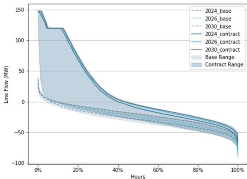
Figure 215215214: Golah-Mortimer Average Delta Flow
