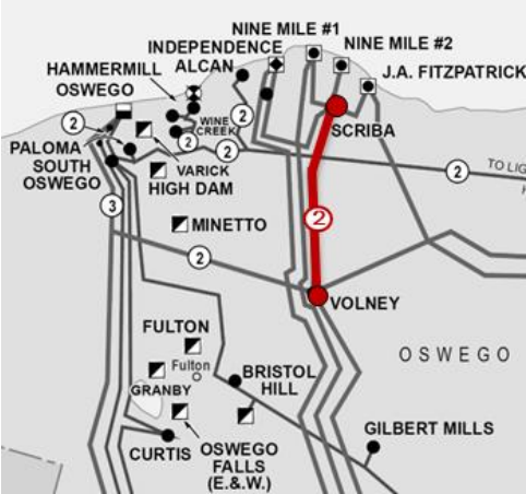
Figure 14144140: Volney-Scriba 345 kV Line Location and Parameters
