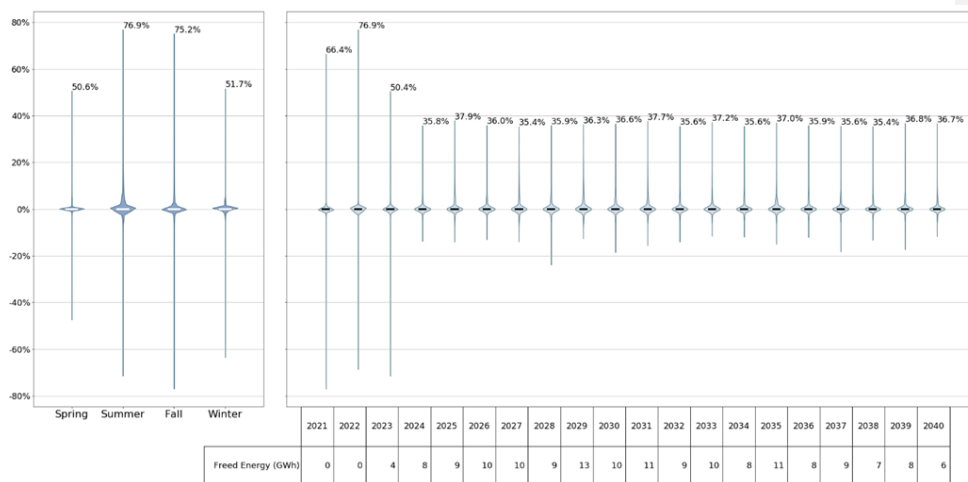
Figure 226226225: Stoner-Rotterdam Delta Hourly Line Utilization
