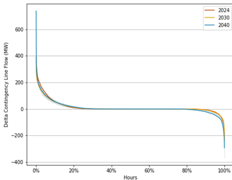
Figure 194194193: New Scotland-Knickerbocker Average Delta Flow (Relax-Contract)
