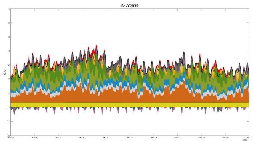
Figure 696968 : Scenario 1 2035 Winter Month Hourly Dispatch
