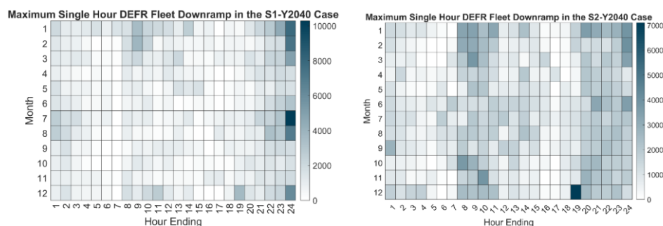
Figure 949493: Maximum DEFR Fleet Down-Ramp (MW/hour) by Month and Hour: 2040 S1 and S2
