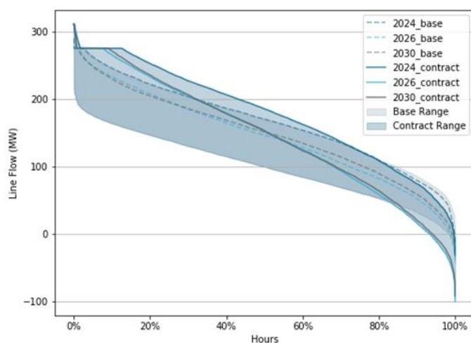
Figure 198198197: Sugarloaf-Ramapo Flow Duration
