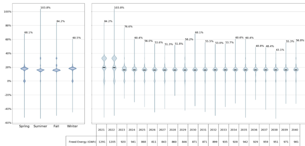
Figure 140140139: Dunwoodie-Long Island Delta Hourly Line Utilization
