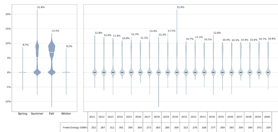
Figure 147 Volney-Scriba Delta Hourly Line Utilization (Relax-Baseline)
