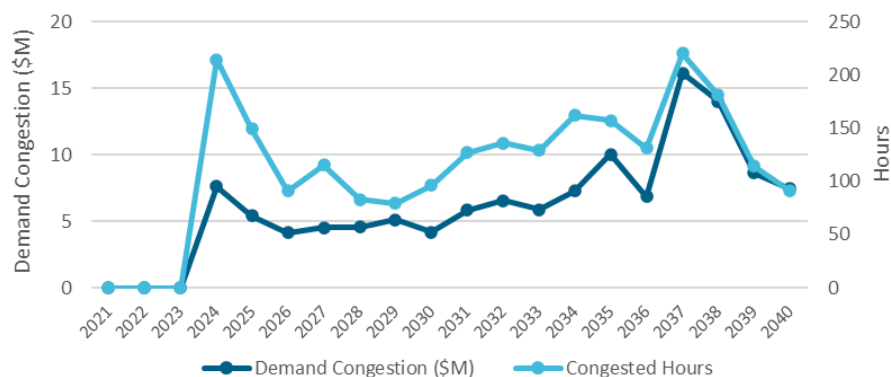
Figure 162162161: Sugarloaf-Ramapo Baseline Case Projected Demand Congestion and Congested Hours
