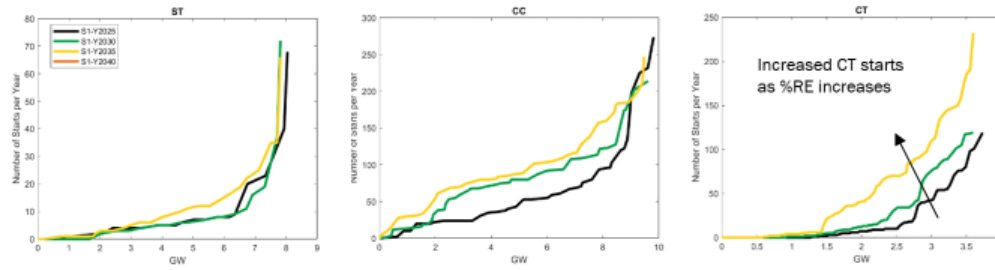
Figure 868685: Fossil Fleet Cumulative Capacity Curve: Unit Level Number of Starts
