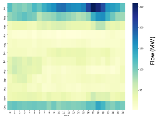
Figure 159159158: New Scotland-Knickerbocker Average Delta Flow
