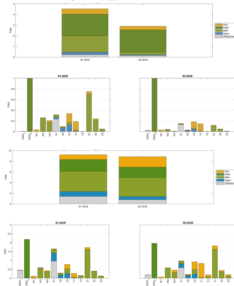
Figure 55554: Curtailment by Generation Type Across the Identified Generation Pockets
