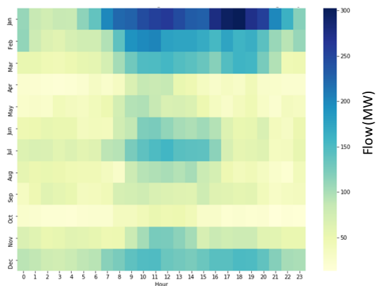
Figure 194194193: New Scotland-Knickerbocker Average Delta Flow (Relax-Contract)
