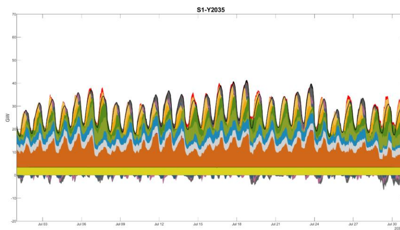
Figure 676766 : Scenario 1 2035 Summer Month Hourly Dispatch
