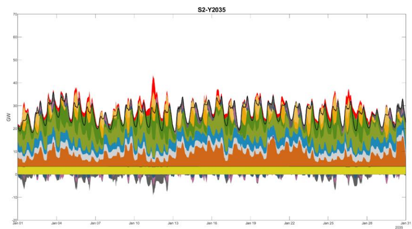
Figure 818 8180 : Scenario 2 2035 Winter Month Hourly Dispatch
