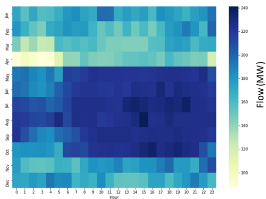
Figure 173173172: Dunwoodie-Long Island Average Delta Flow
