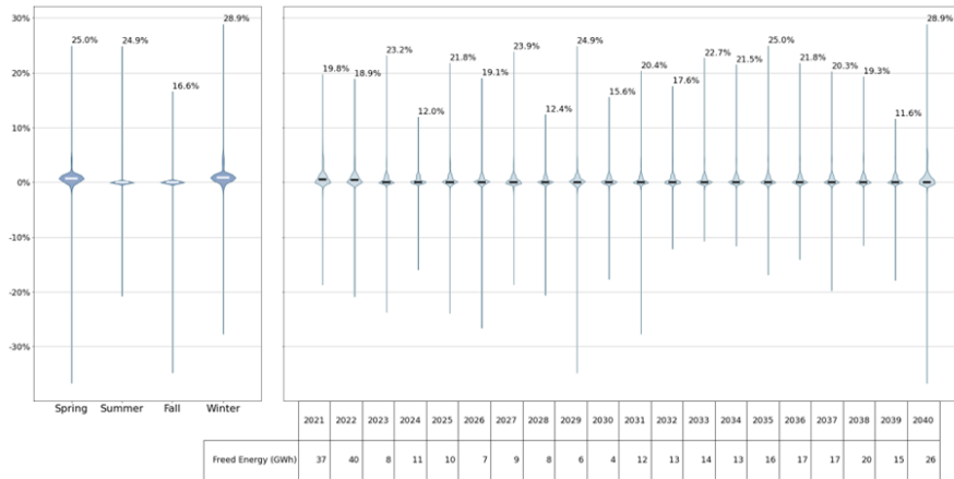
Figure 188188187: Dunwoodie-Motthaven Delta Hourly Line Utilization
