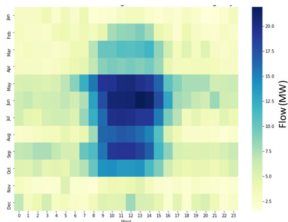
Figure 225225224: Stoner-Rotterdam Average Delta Flow (Relax-Contract)
