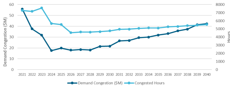
Figure 168168167: Dunwoodie-Long Island Contract Case Projected Demand Congestion and Congested Hours
