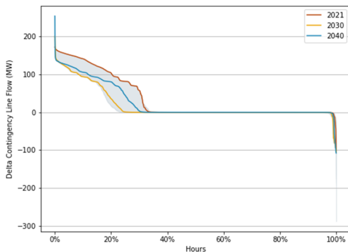
Figure 180180179: Volney-Scriba Average Delta Flow (Relax-Contract)
