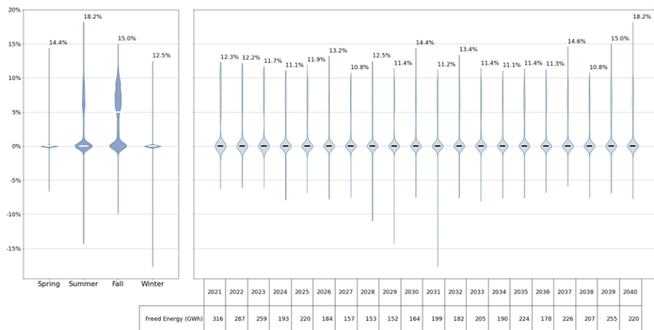
Figure 181181180: Volney-Scriba Delta Hourly Line Utilization
