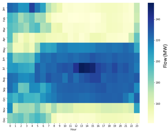
Figure 139139138: Dunwoodie-Long Island Average Delta Flow (MW)
