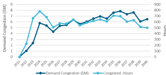
Figure 228228227: Jennison-Sidney Projected Contract Case Demand Congestion and Congested Hour
