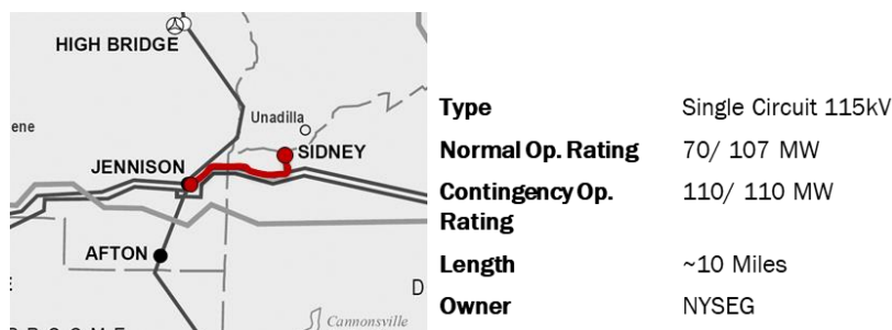
Figure 227227226: Jennison-Sidney Line Location and Parameters
