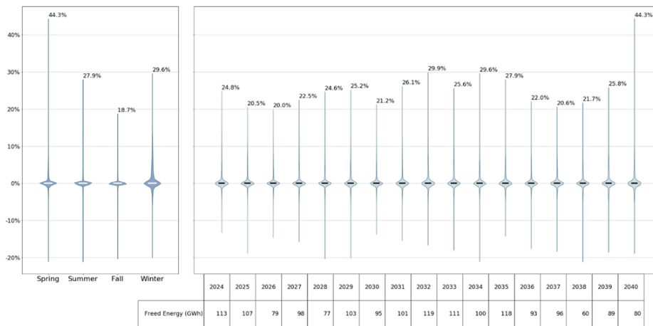
Figure 195195194: New Scotland-Knickerbocker Delta Hourly Line Utilization
