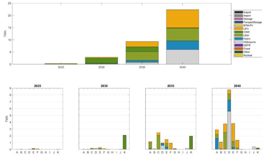
Figure 51: Scenario 2 Production Cost Curtailment by Type by Zone
