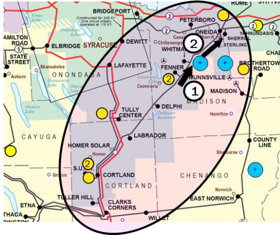
Figure 258258255: Pocket Z3 Congestion and Energy Deliverability Summary (2035)
