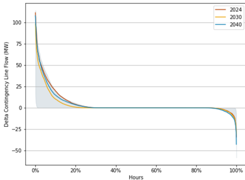
Figure 200200199: Sugarloaf-Ramapo Delta Flow Duration Curve (Relax-Contract)
