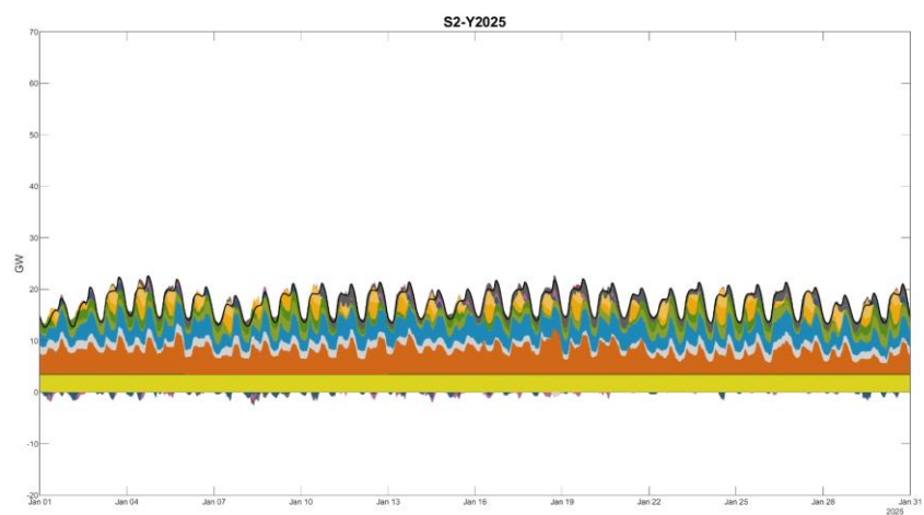
Figure 7575 74: Scenario 2 2025 Winter Month Hourly Dispatch
