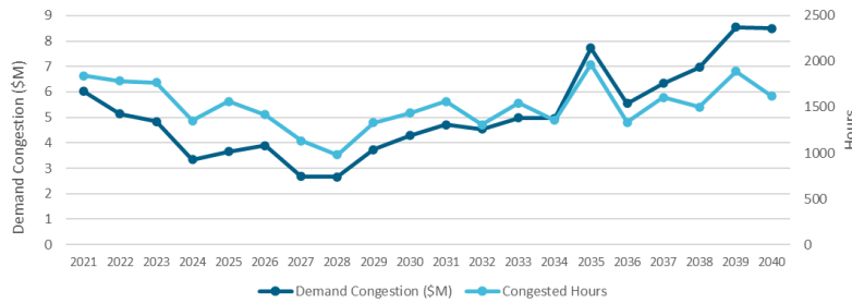
Figure 175175174: Contract Case Projected Demand Congestion and Congested Hours
