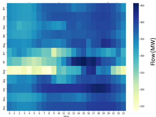
Figure 209209208: Barrett-Valley Stream Average Delta Flows
