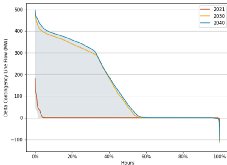
Figure 209209208: Barrett-Valley Stream Average Delta Flows
