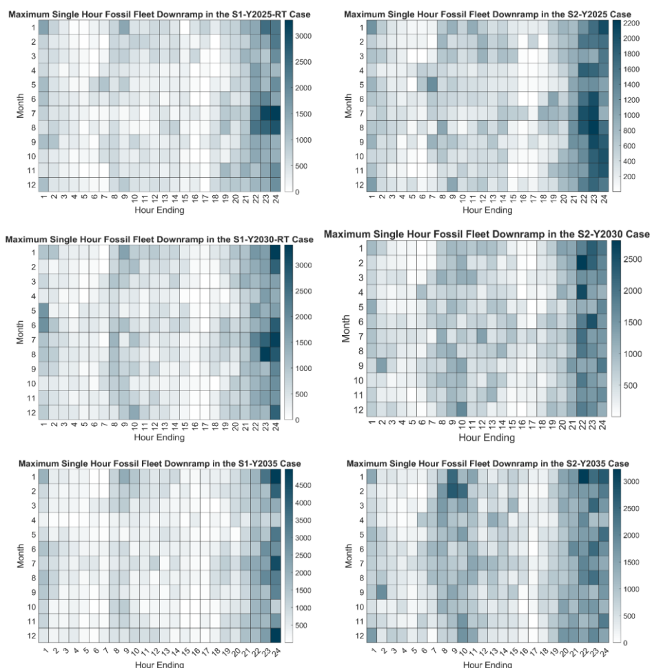
Figure 898988: Maximum Fossil Fleet Down-Ramp (MW/hour) by Month and Hour
