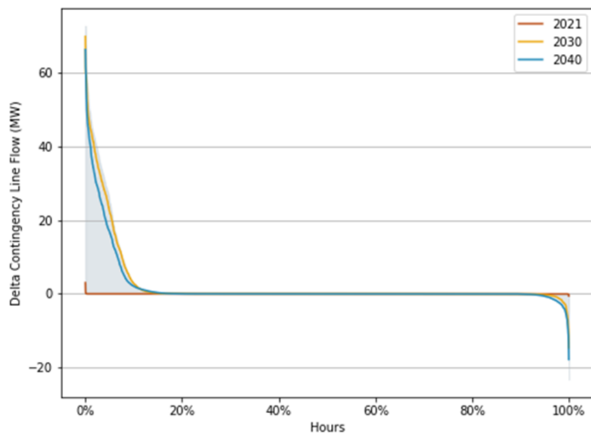
Figure 217217216: Golah-Mortimer Average Delta Flow (Relax-Contract)
