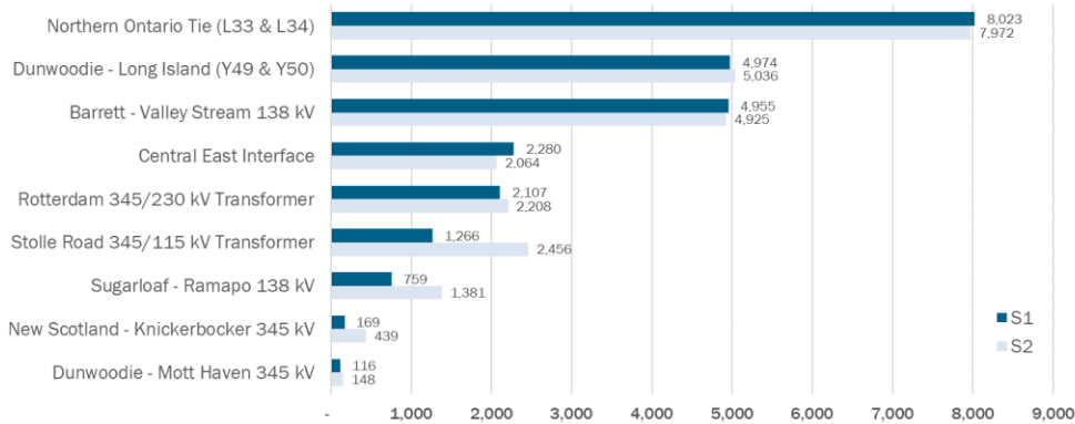
Congested Hours for Bulk Constraints (2035)
