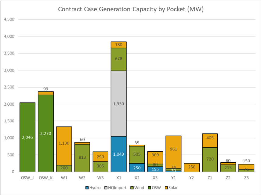
Figure 20: Contract Case Generation Capacity by Pocket (MW)
