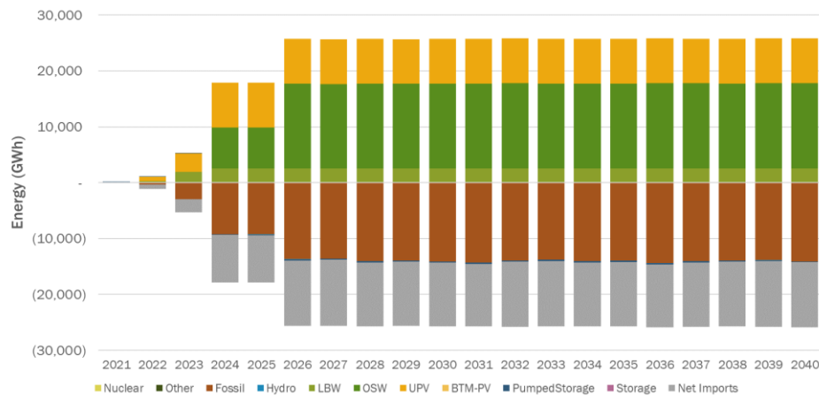
Figure 151415: Projected Change in NYCA Energy Generated by Fuel Type, Contract Case
