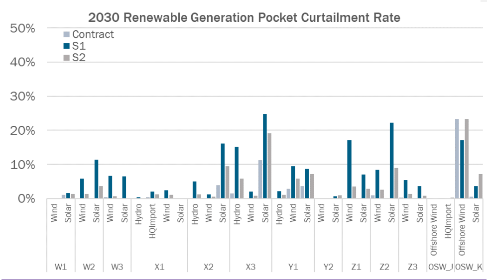
Figure 30: Renewable Generation Pocket Curtailment Rates by Generation Type in 2030 and 2035
