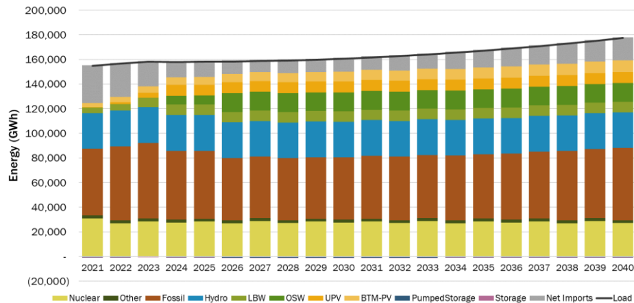
Figure 141314: Projected NYCA Energy Generated by Fuel Type, Contract Case
