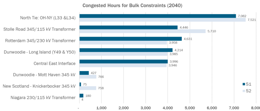
Figure 243424: Number of Congested Hours for Bulk Constraints, Year 2040
