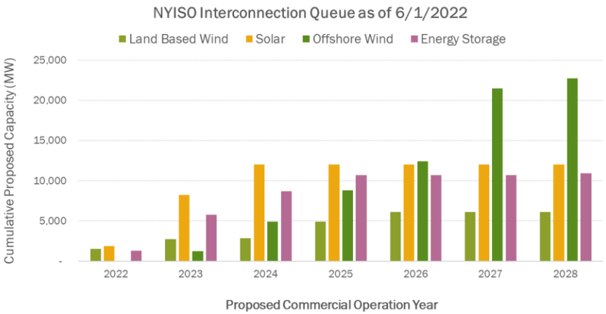
Figure 9.89: Proposed Renewable Energy Capacity in the NYISO Interconnection Queue
