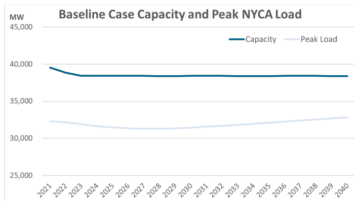
Figure 10910: Baseline Case NYCA Capacity and Peak Loads
