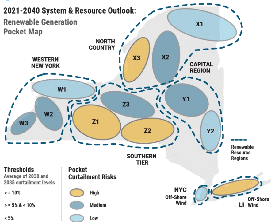
Figure 29: Renewable Generation Pocket Map
