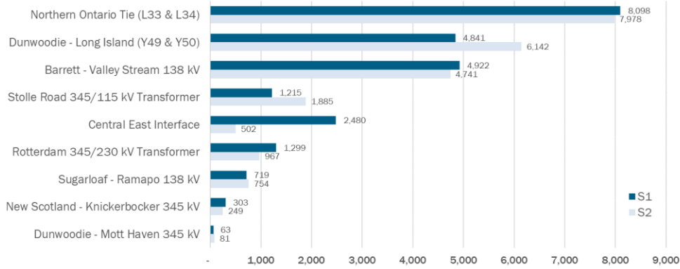
Congested Hours for Bulk Constraints (2030)
