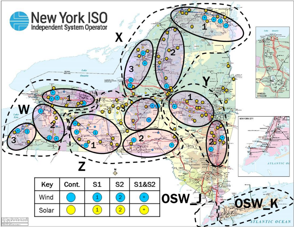
Figure 27: 2035 Policy Case Pocket Map
