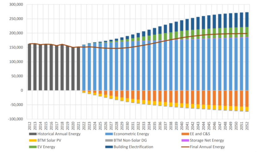
Figure 4: NYCA Baseline Annual Energy Forecast Components (GWh)
