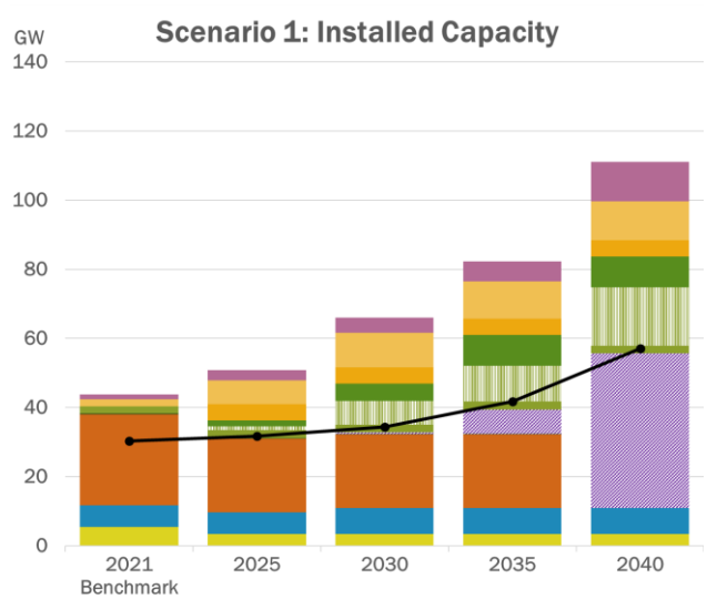
Figure 202420: Policy Case New York Capacity Expansion Results
