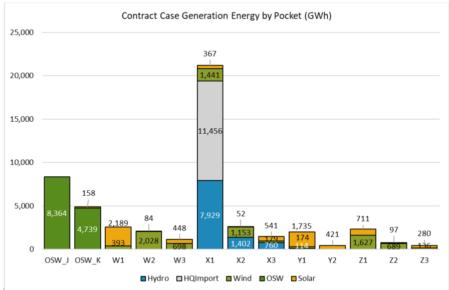
Figure 21: Contract Case Generation Energy by Pocket After Curtailment in 2030 (GWh)
