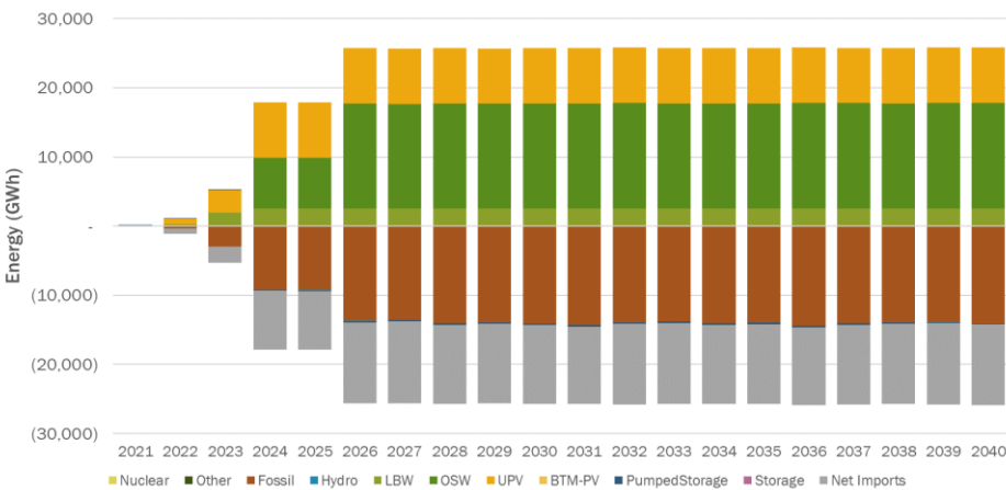
Figure 11: Baseline Case NYCA Generation and Net Imports (GWh)
