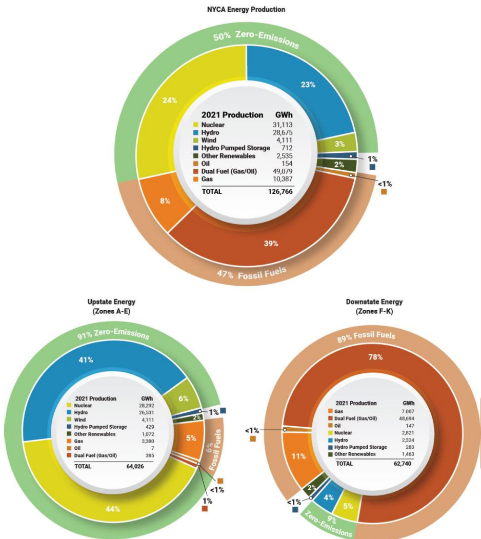
Figure 3: Energy Production by Fuel Source (GWh) – Statewide, Upstate, & Downstate New York: 2021 Statewide, Upstate, & Downstate New York: 2021
