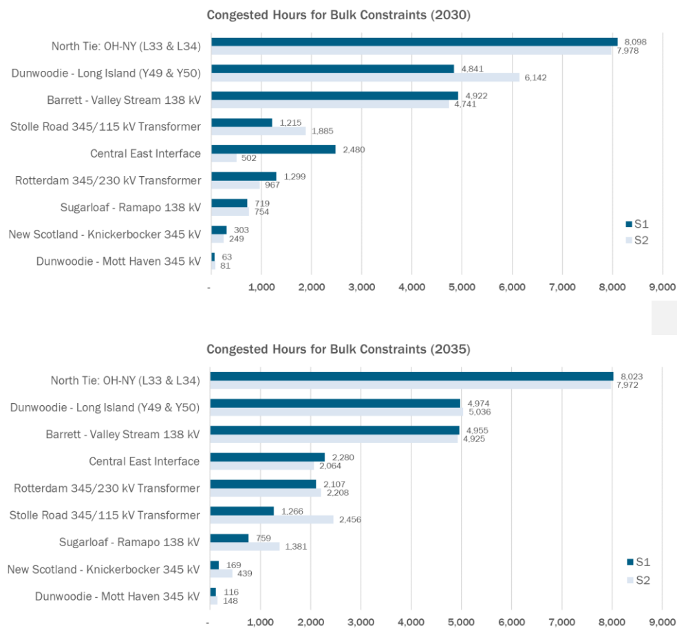
Figure 233323: Number of Congested Hours for Bulk Constraints, Years 2030 and 2035
