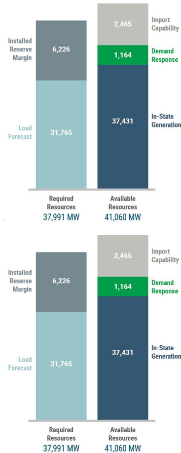
Figure 167: Statewide Resource Availability: Summer 2022
