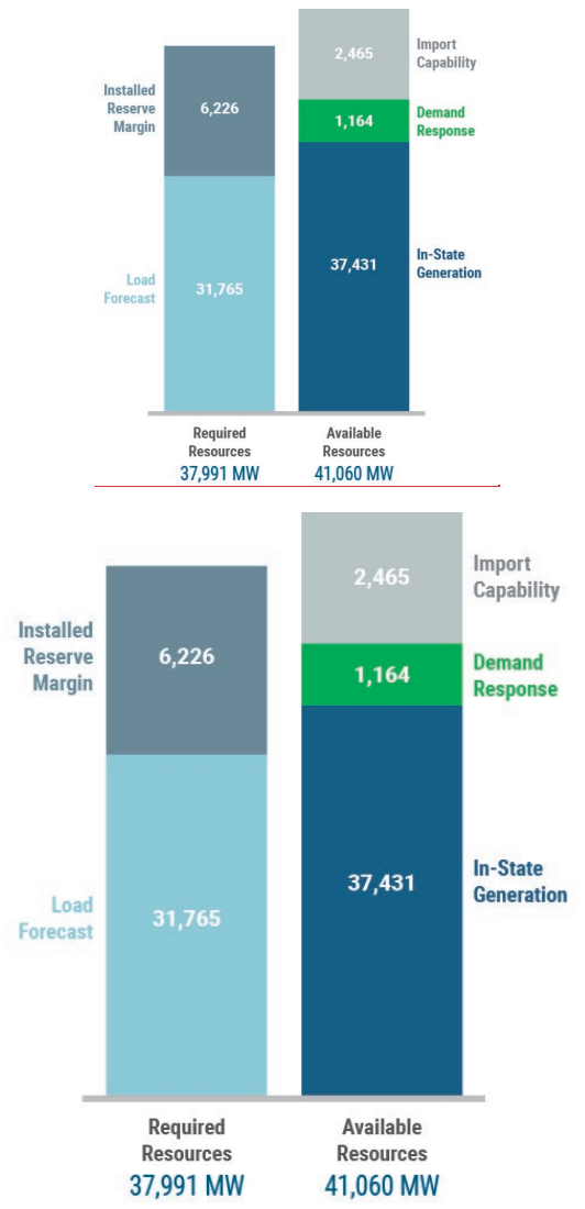
Figure 7: Statewide Resource Availability: Summer 2022
