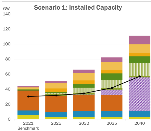
Figure 20: Policy Case New York Capacity Expansion Results
