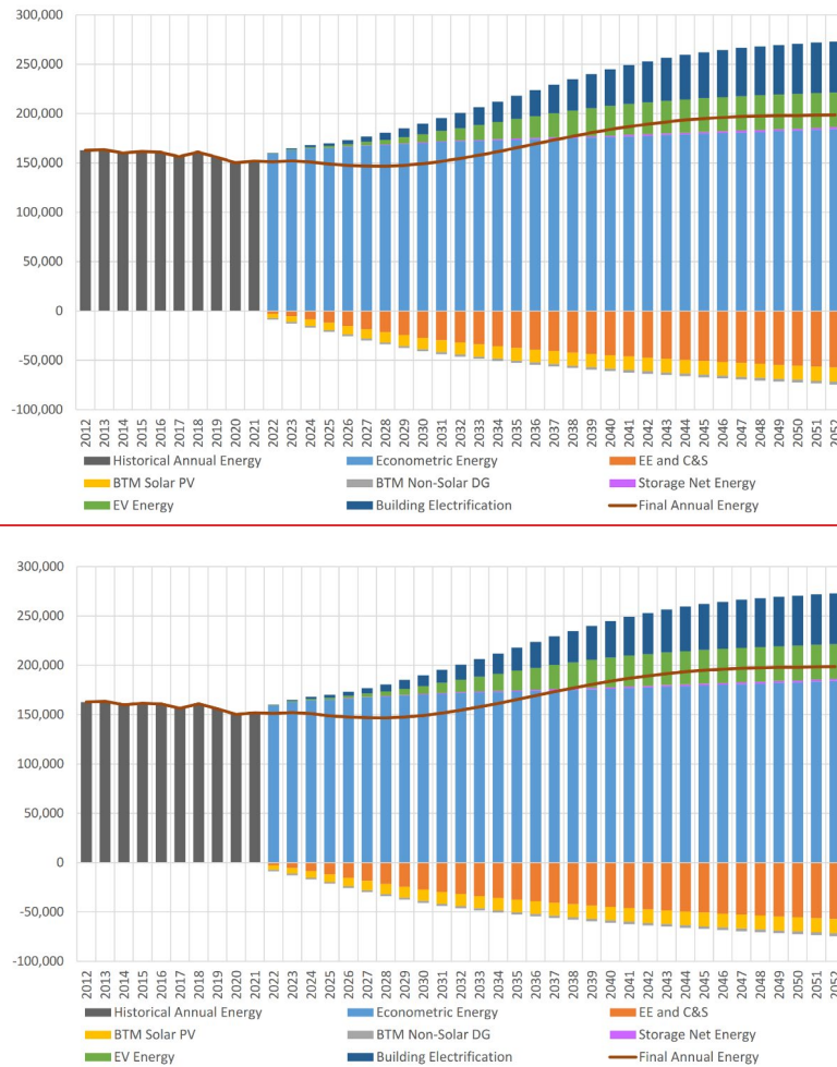
Figure 4: NYCA Baseline Annual Energy Forecast Components (GWh)
