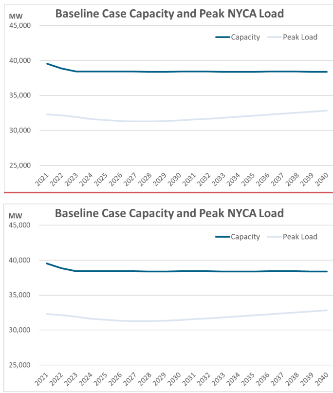
Figure 10: Baseline Case NYCA Capacity and Peak Loads
