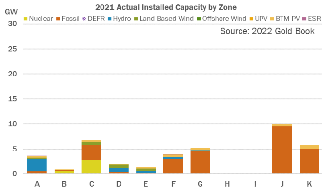
Figure 21: 2021 Actual Installed Capacity By Zone
