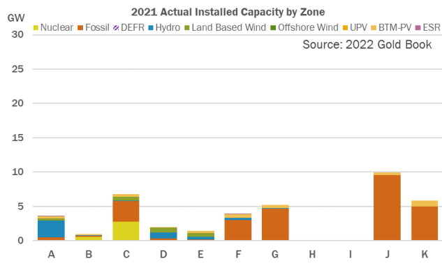
Figure 22: Policy Case 2040 Installed Capacity by Zone
