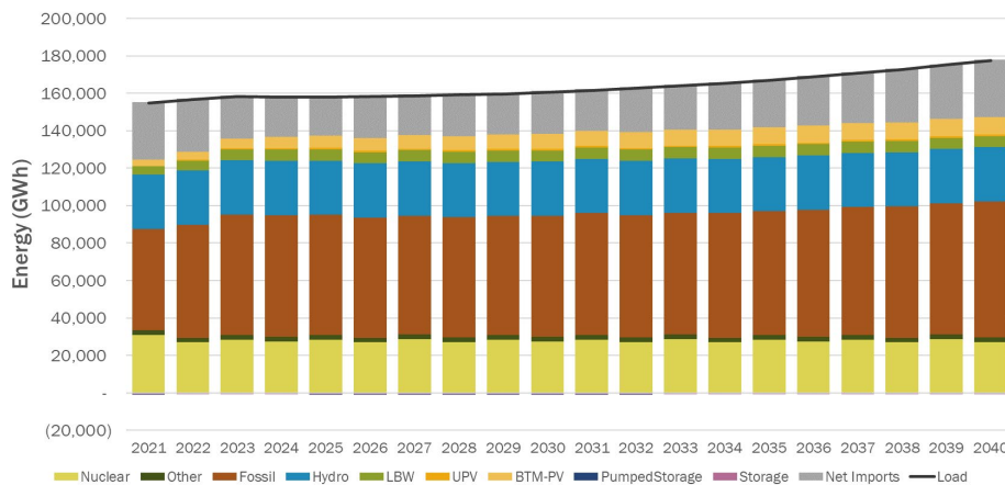
Figure 11: Projected NYCA Energy Generated by Fuel Type, Baseline Case NYCA Generation and Net Imports
