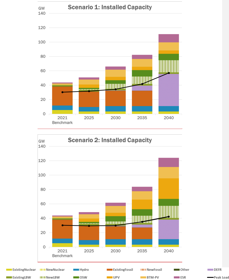
Figure 20: Policy Case New York Capacity Expansion Results
