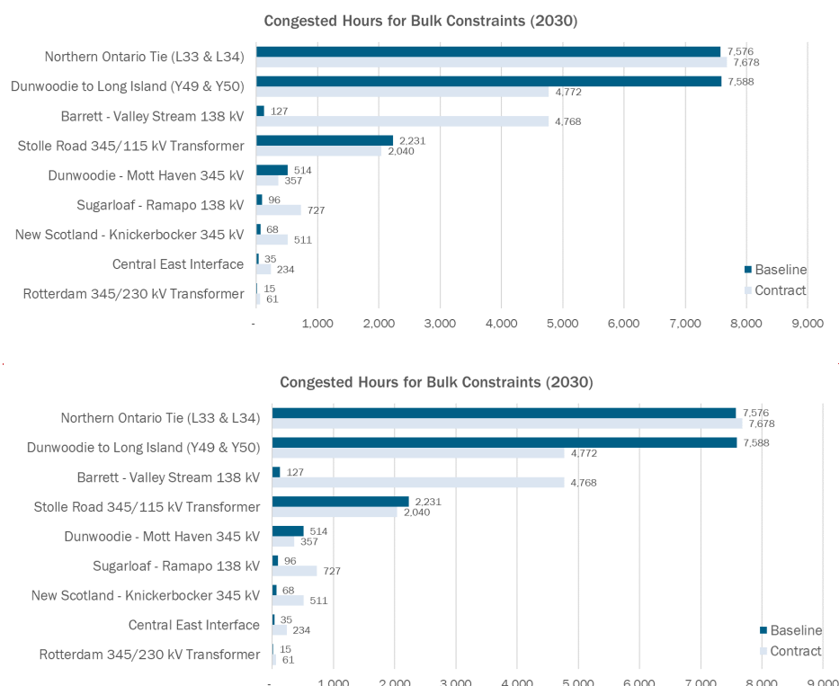
Figure 16: Number of Congested Hours by Constraint, Baseline and Contract Cases 24
