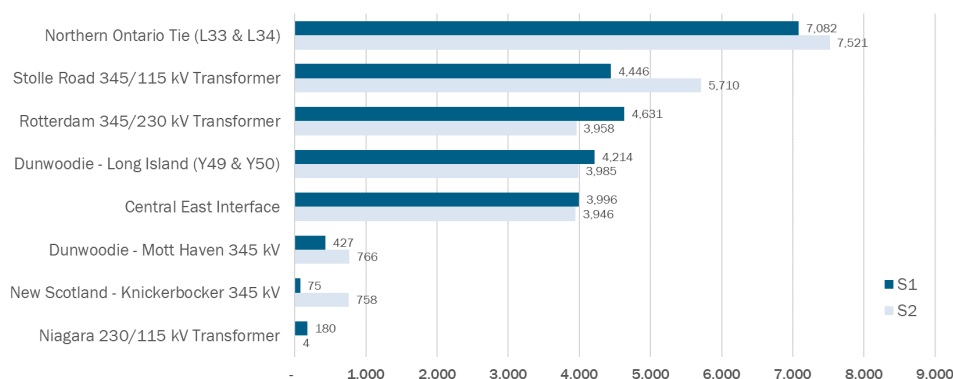
Congested Hours for Bulk Constraints (2040)
