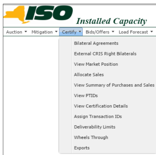
Figure 4: Certify Menus
