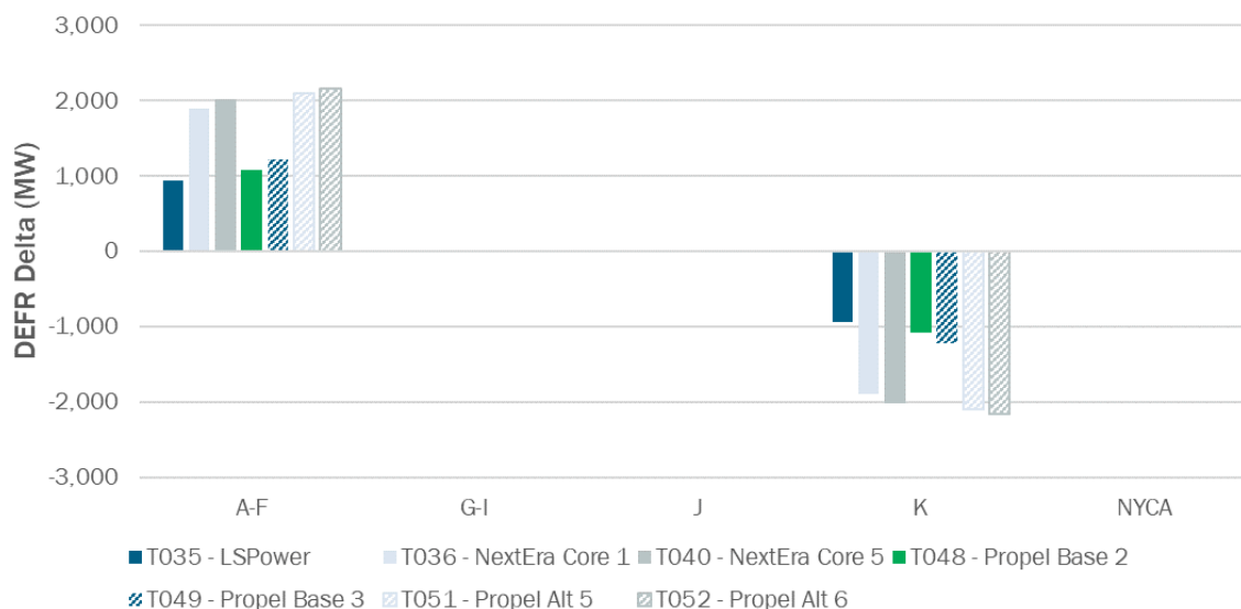
Figure 14: Policy Scenario: 2040 DEFR Installed Capacity Delta to Pre-Project (MW)
