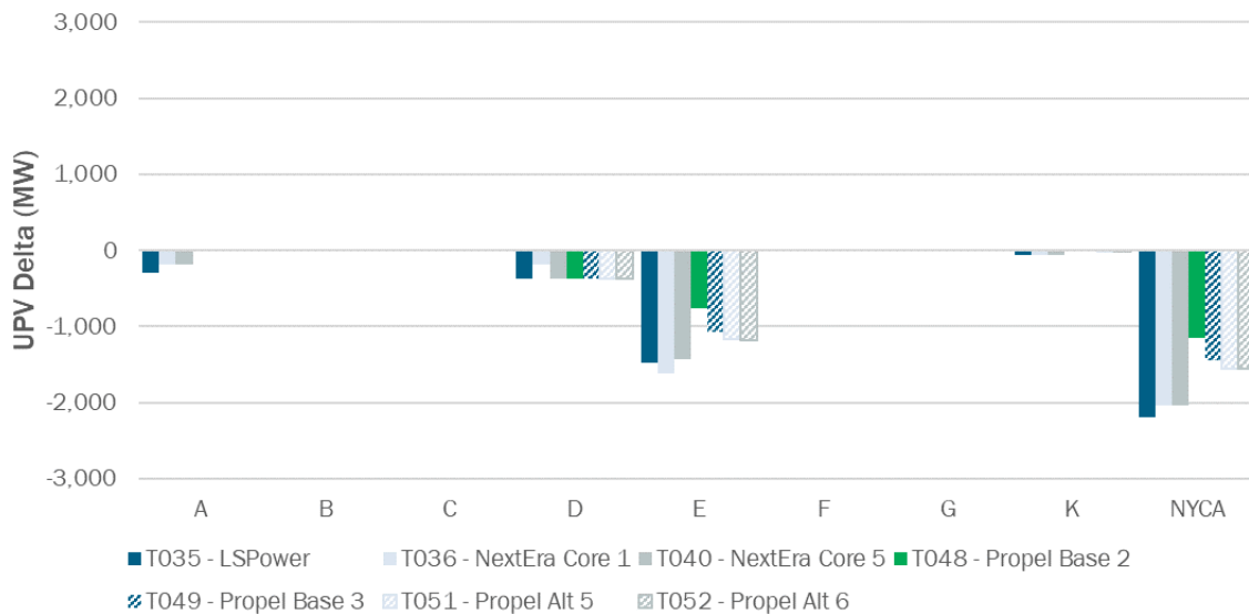
Figure 9: Policy + B-VS Scenario: 2040 Solar (UPV) Installed Capacity Delta to Pre-Project
