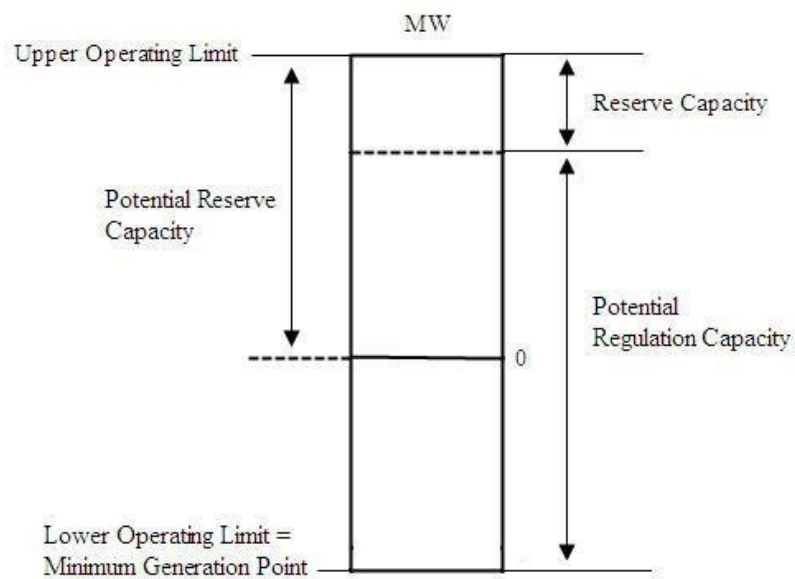
Figure 5: Demand Side Resources Operating Characteristics
