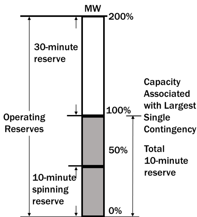
Figure 12: Minimum Operating Reserve Requirements
