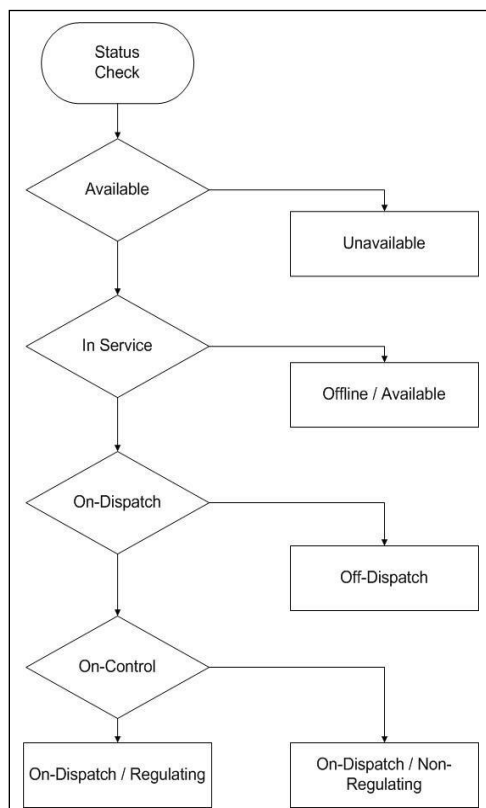
Figure 9: Generating Unit Operating States
