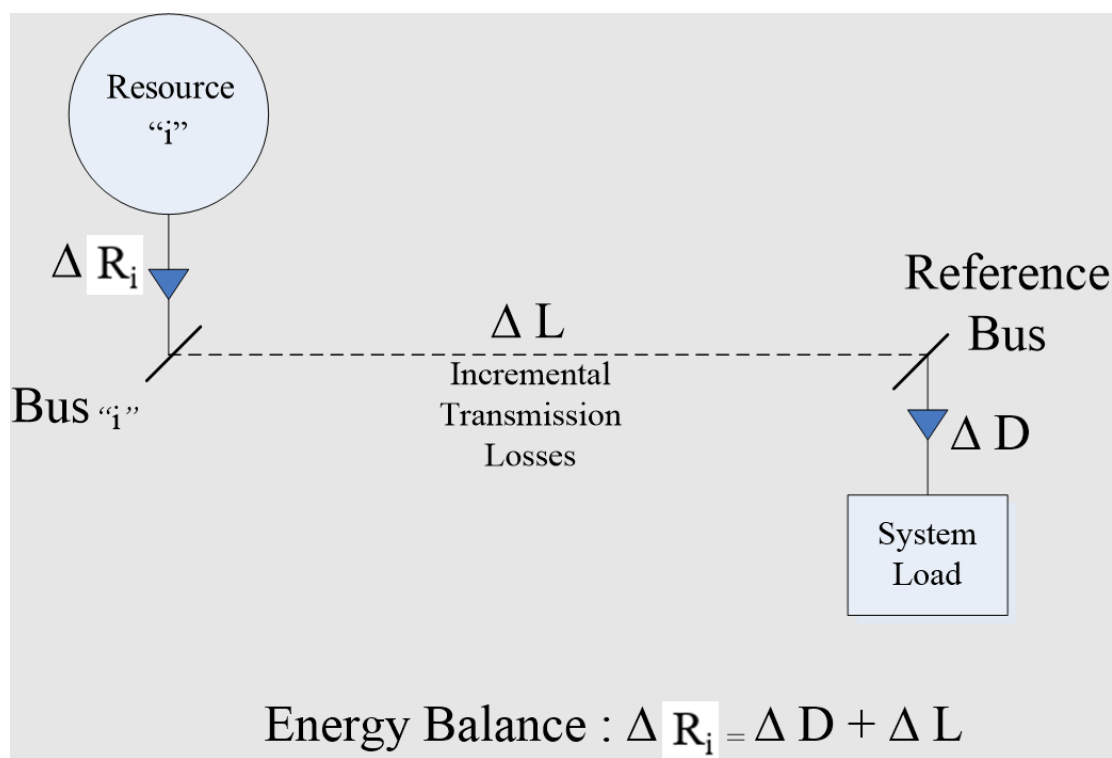
Figure 6: Incremental Transmission Losses
