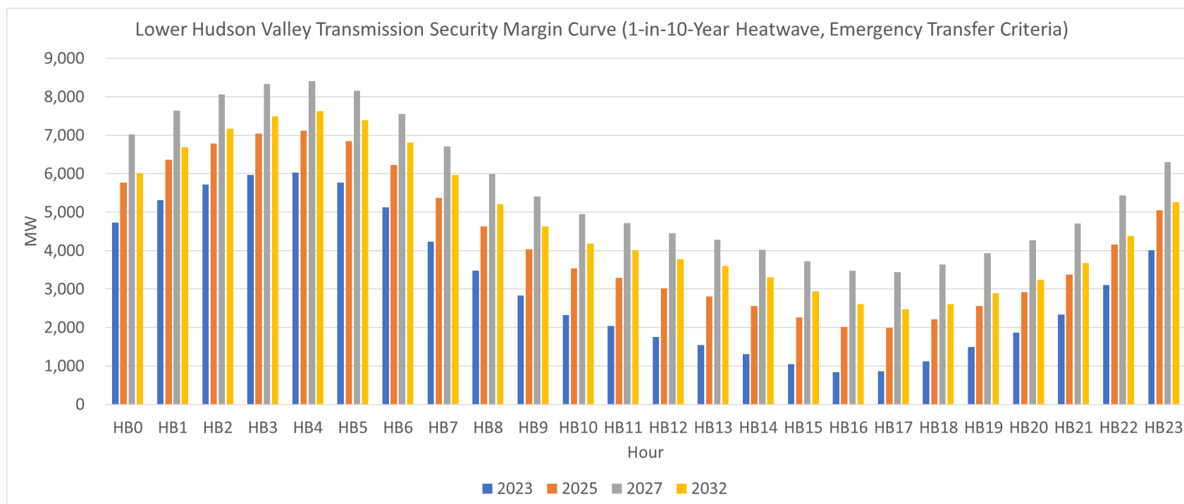
Figure 39: Lower Hudson Valley Transmission Security Margin Hourly Curve (1-in-10-Year Heatwave, Emergency Transfer Criteria)
