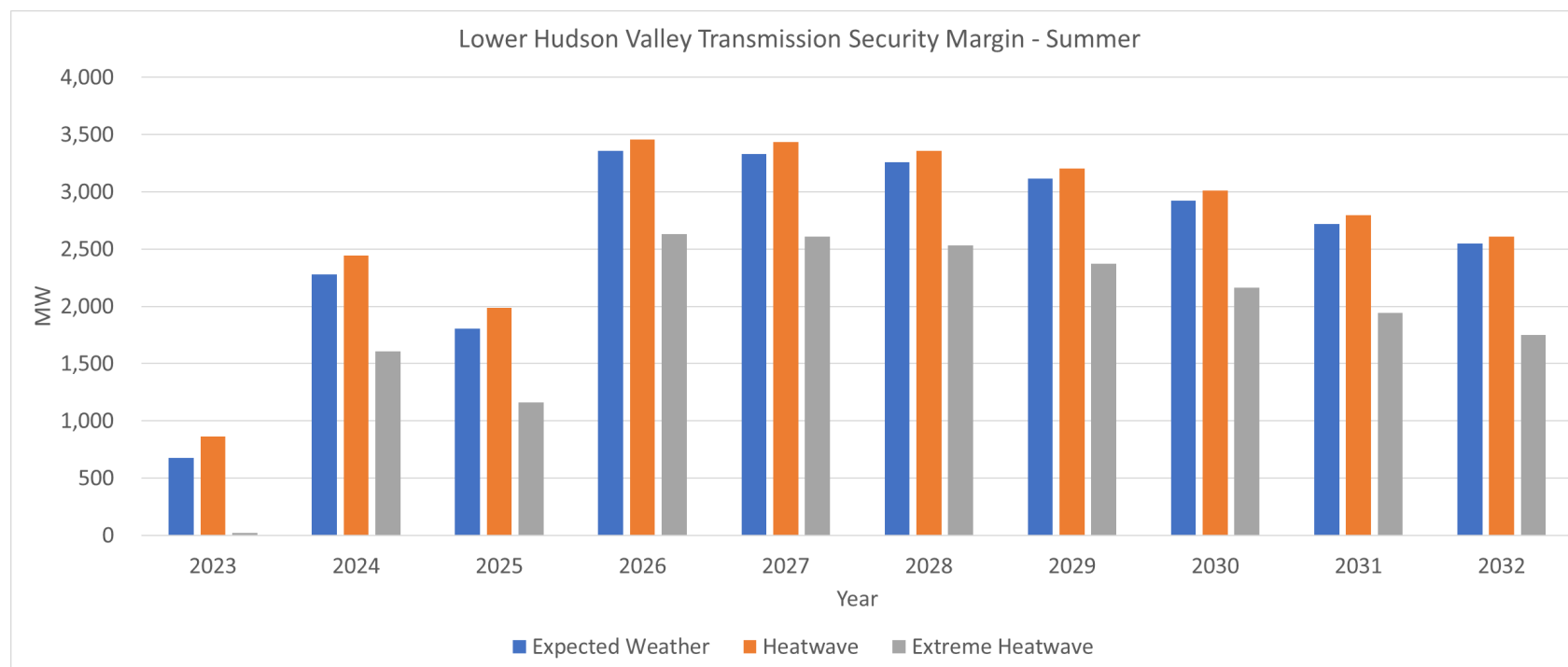
Figure 46: Summary of Lower Hudson Valley Summer Transmission Security Margin – Summer
