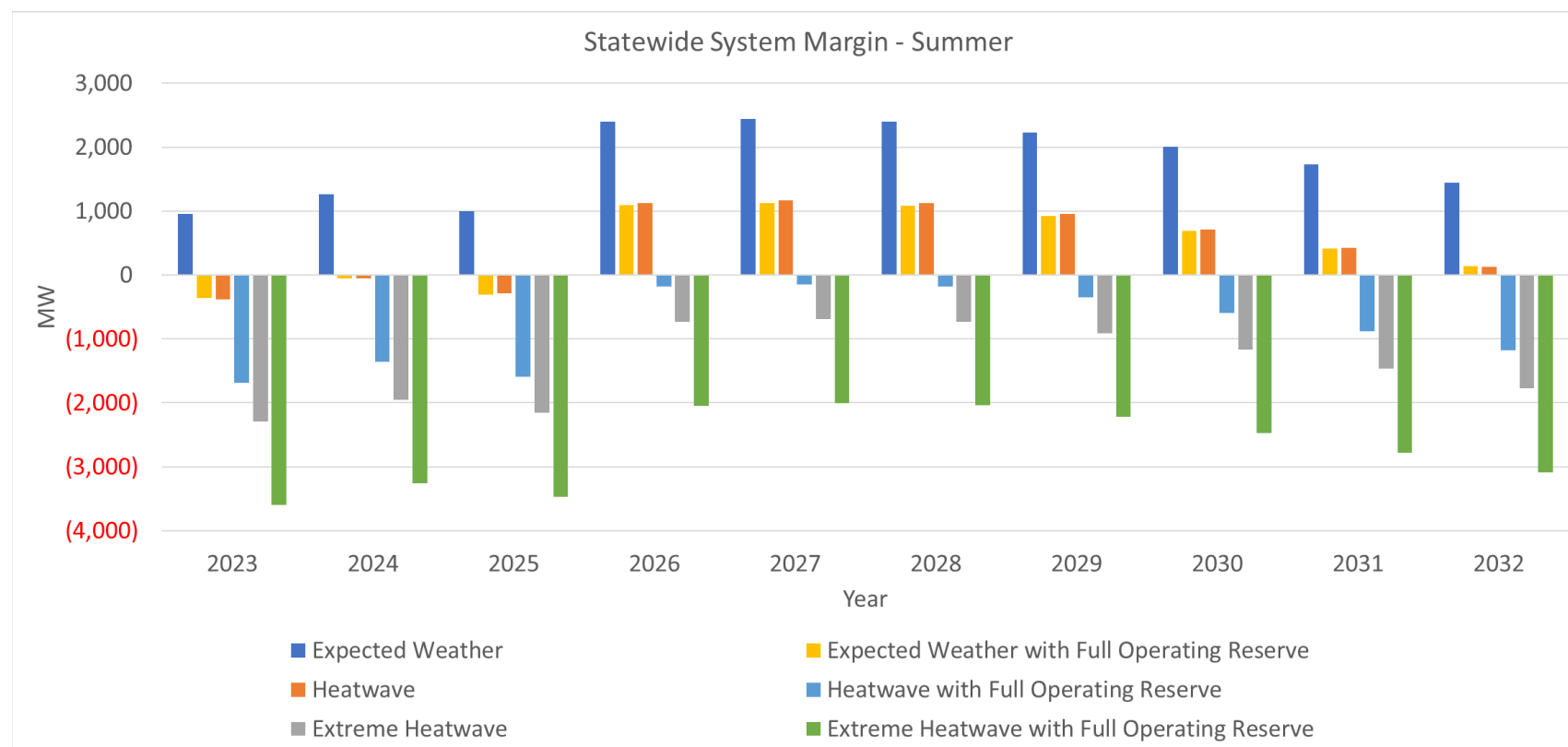
Figure 31: Summary of Statewide System Margin – Summer
