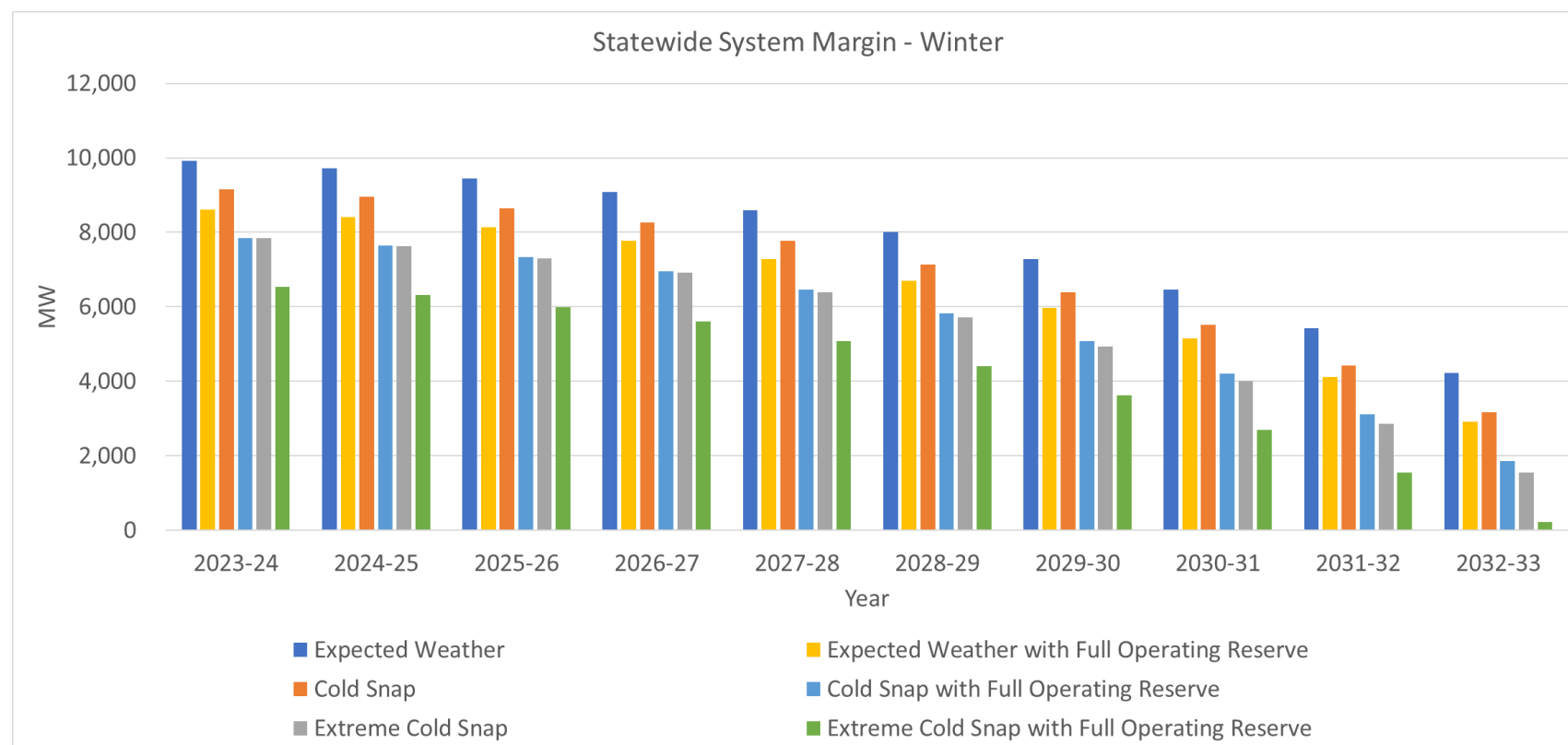
Figure 32: Summary of Statewide System Margin – Winter
