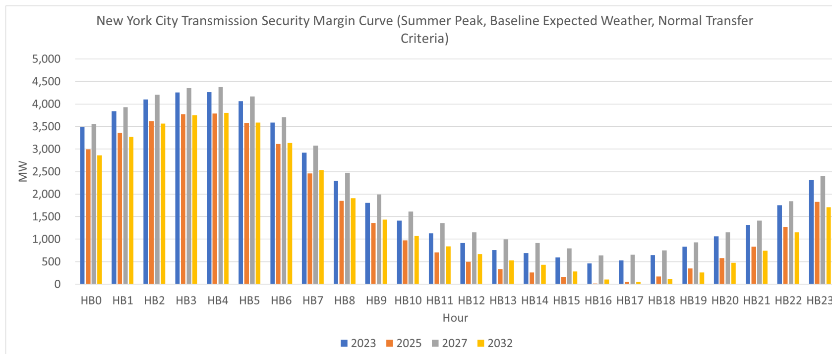
Figure 51: New York City Transmission Security Margin Hourly Curve (Summer Peak – Baseline Expected Weather, Normal Transfer Criteria)
