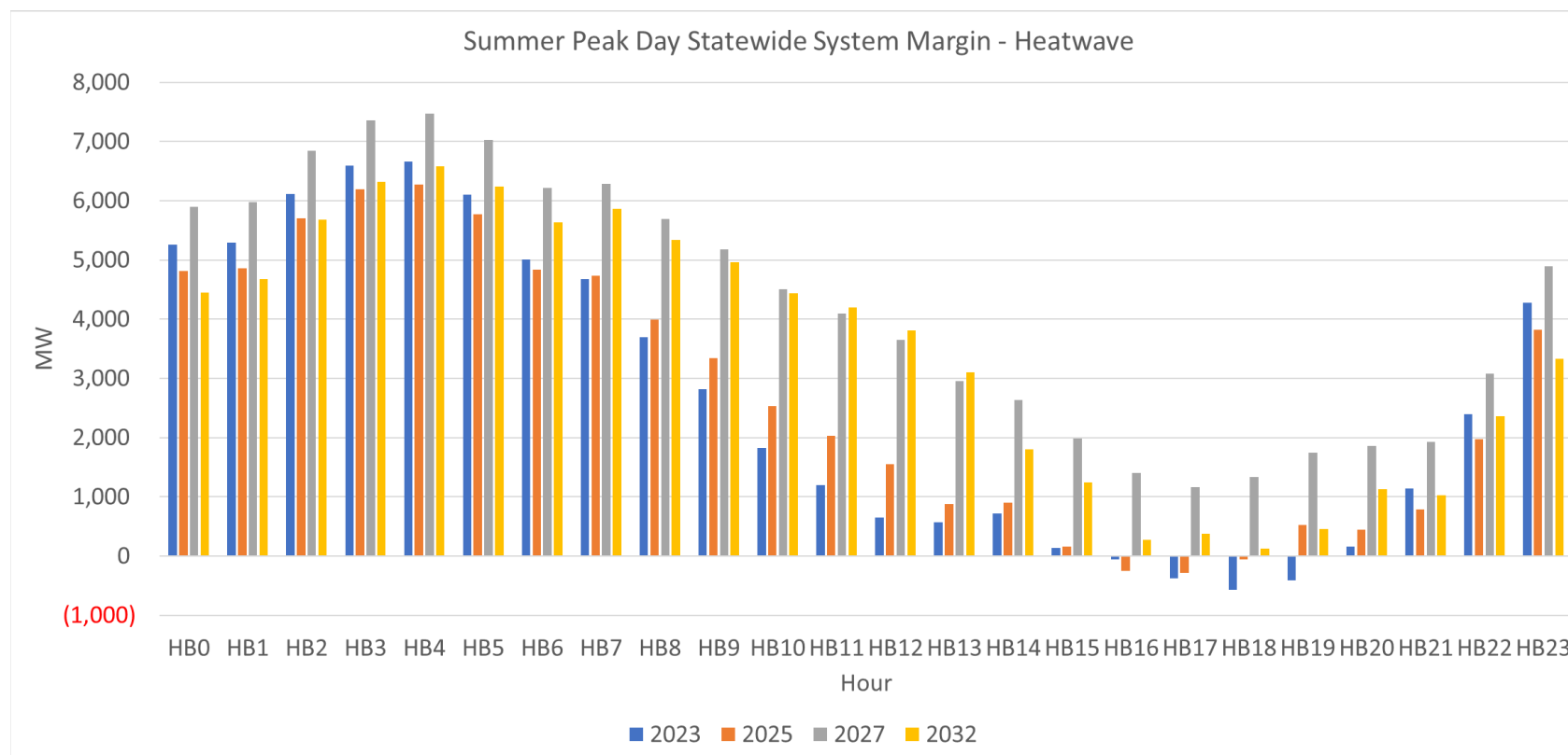
Figure 24: Statewide System Margin Hourly Curve (1-in-10-Year Heatwave, Emergency Transfer Criteria)
