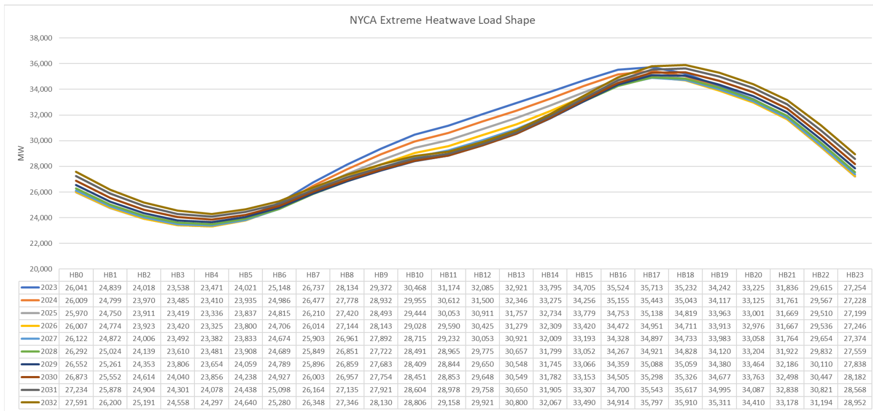
Figure 91: NYCA Extreme Heatwave Load shape
