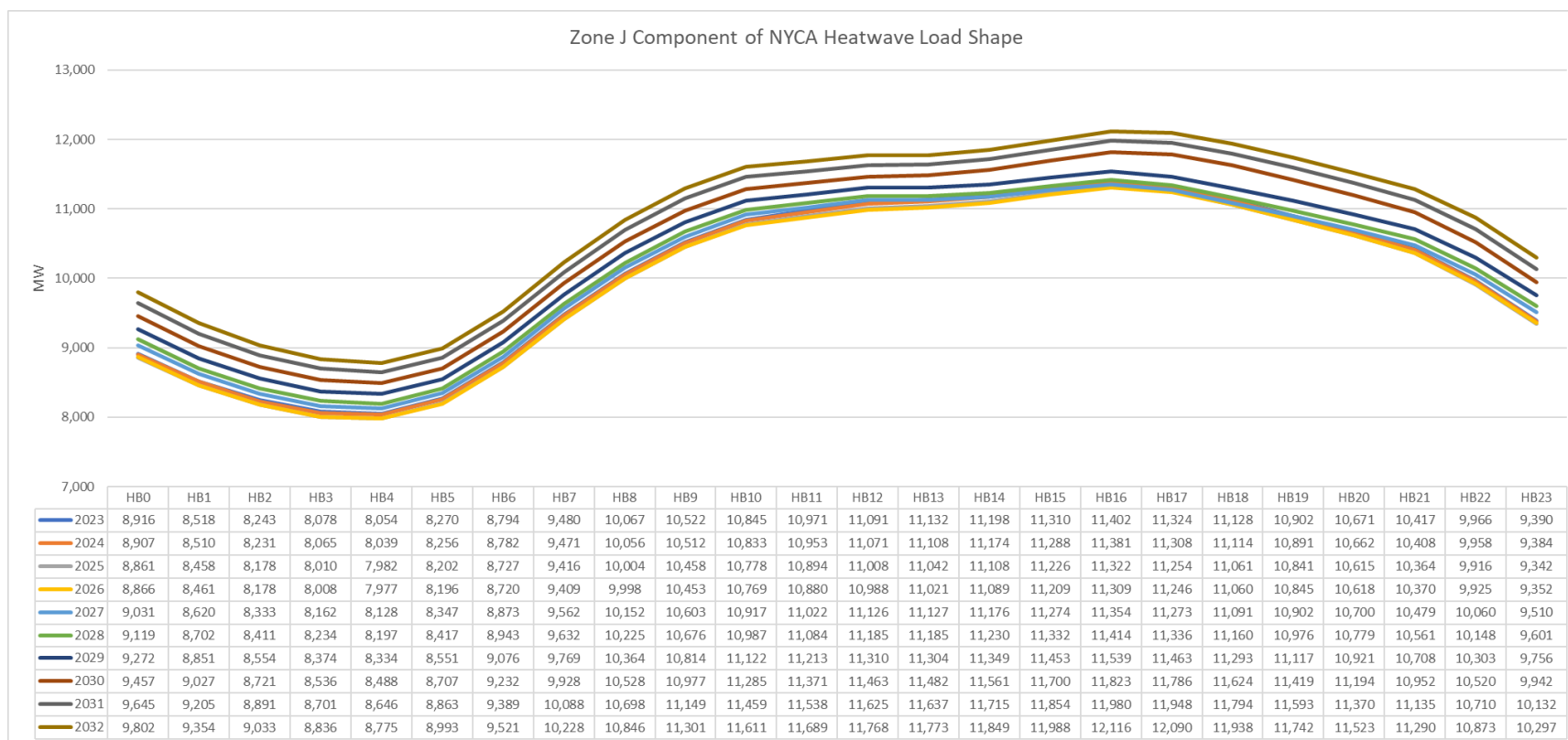
Figure 89: Zone J Component of NYCA Heatwave Load shape
