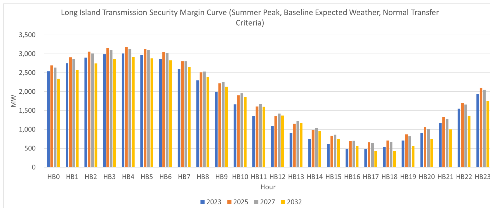
Figure 67: Long Island Transmission Security Margin Hourly Curve (Summer Peak – Baseline Expected Weather, Normal Transfer Criteria)
