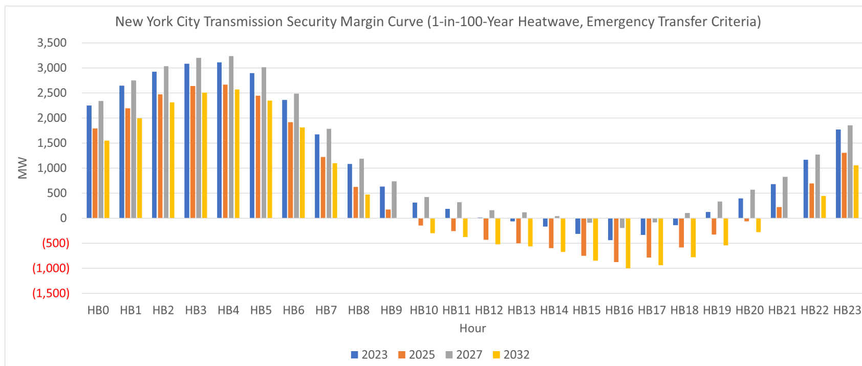
Figure 57: New York City Transmission Security Margin Hourly Curve (1-in-100-Year Extreme Heatwave, Emergency Transfer Criteria)
