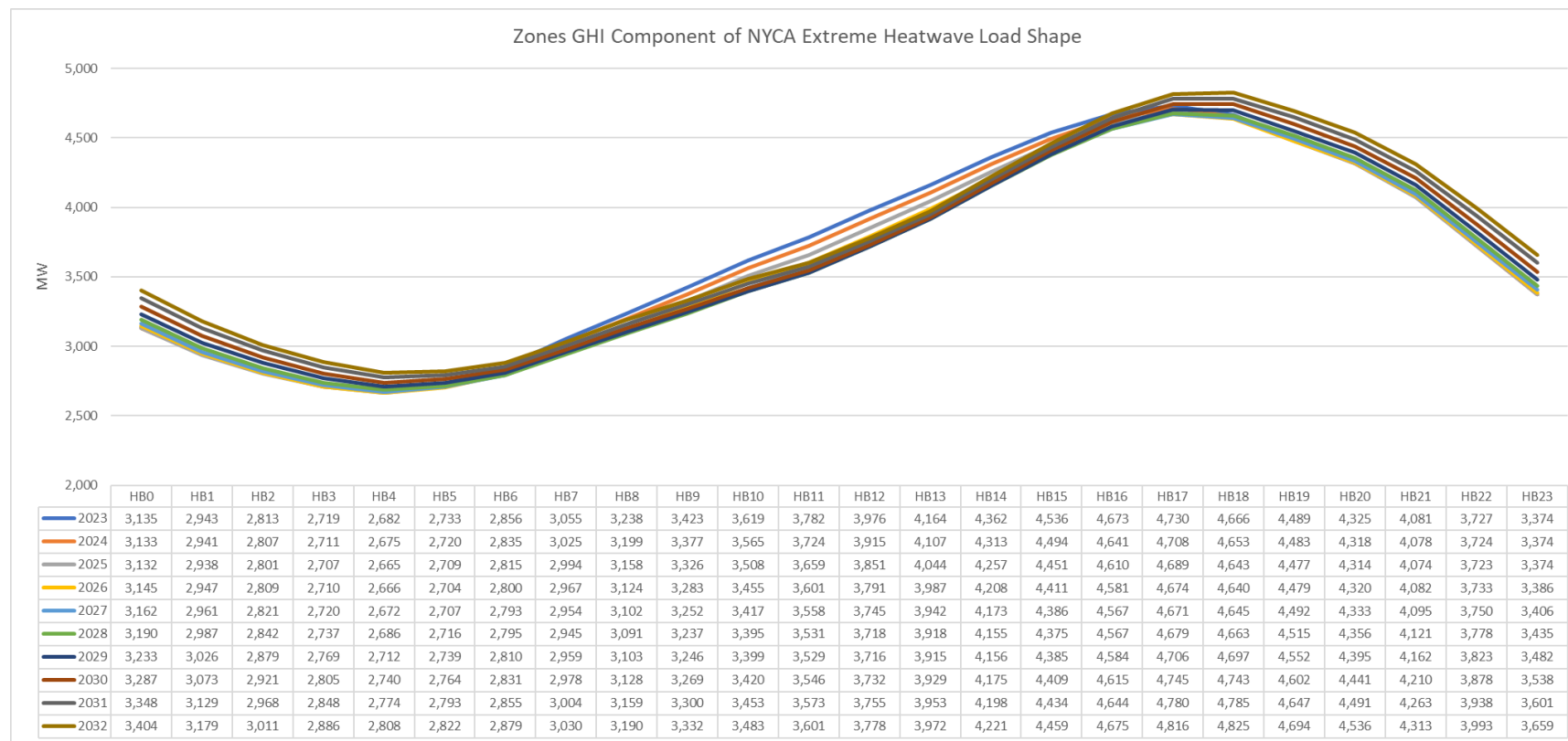
Figure 93: Zones GHI Component of NYCA Extreme Heatwave Load shape
