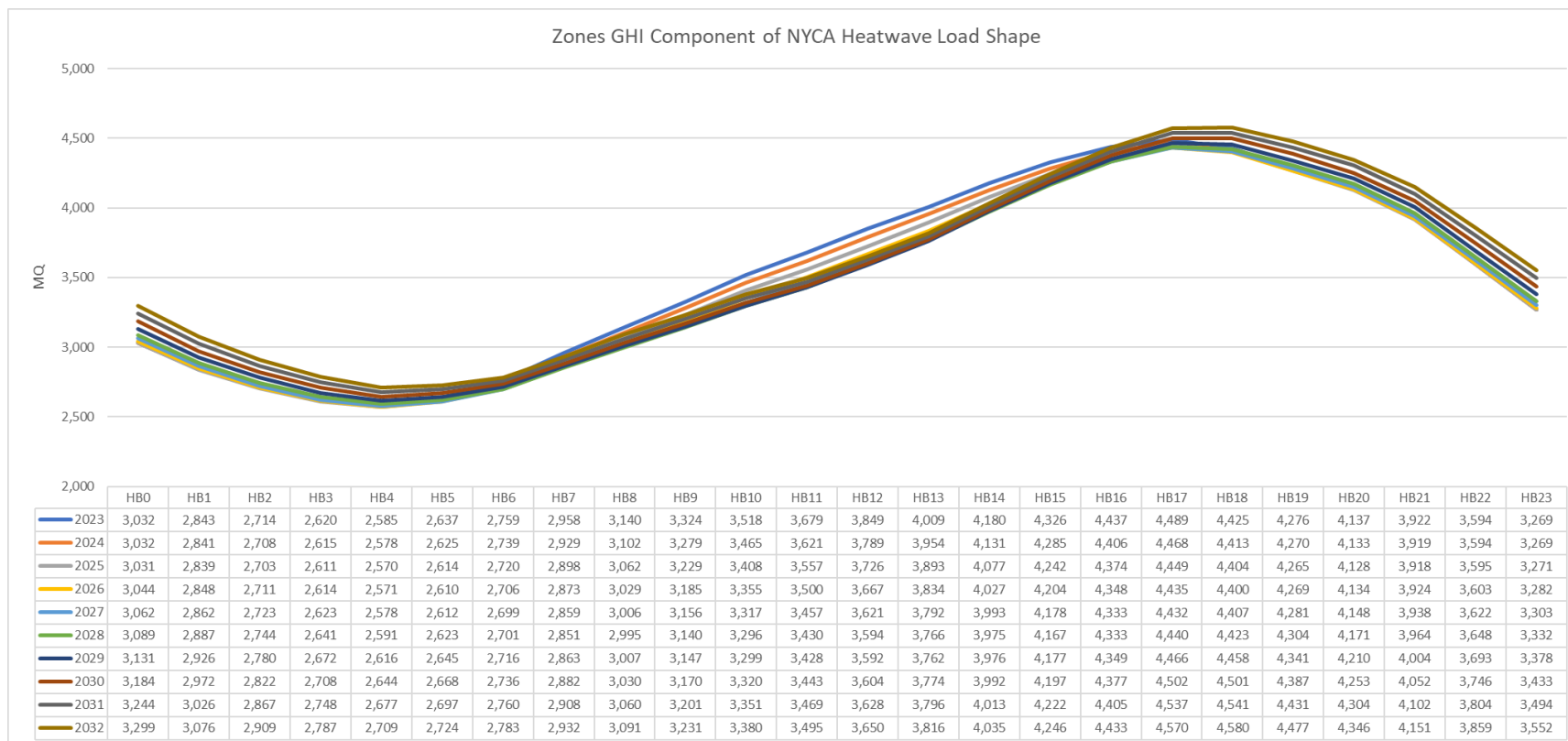
Figure 88: Zones GHI Component of NYCA Heatwave Load shape
