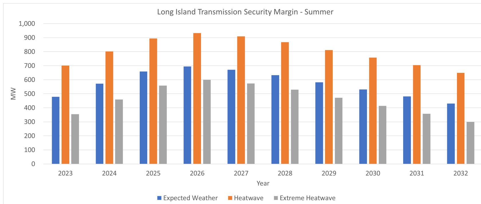
Figure 78: Summary of Long Island Summer Transmission Security Margin – Summer
