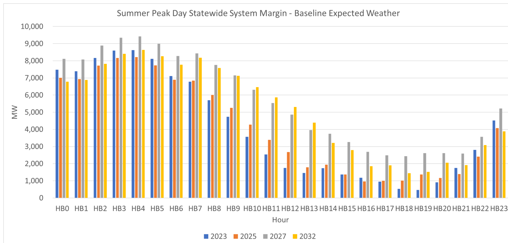
Figure 21: Statewide System Margin Hourly Curve (Summer Peak - Baseline Expected Weather, Normal Transfer Criteria)
