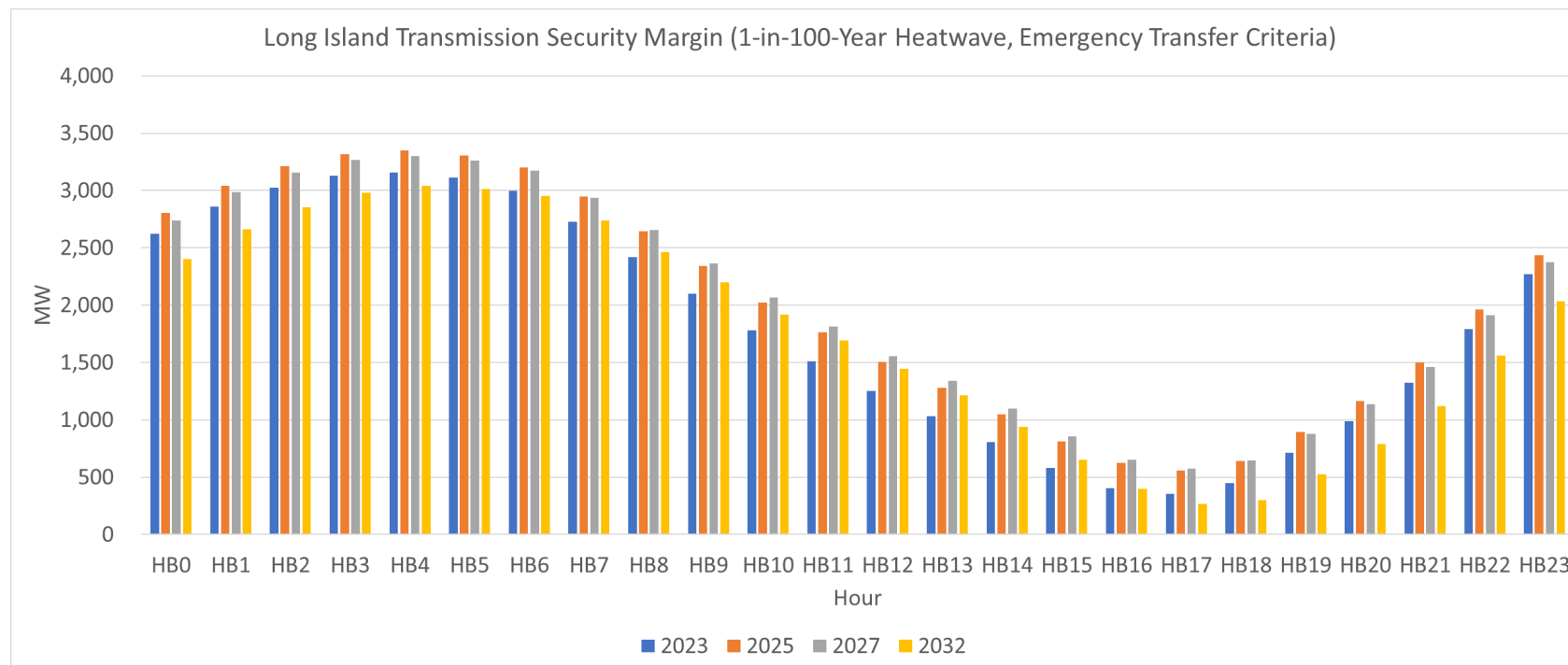
Figure 73: Long Island Transmission Security Margin Hourly Curve (1-in-100-Year Extreme Heatwave, Emergency Transfer Criteria)
