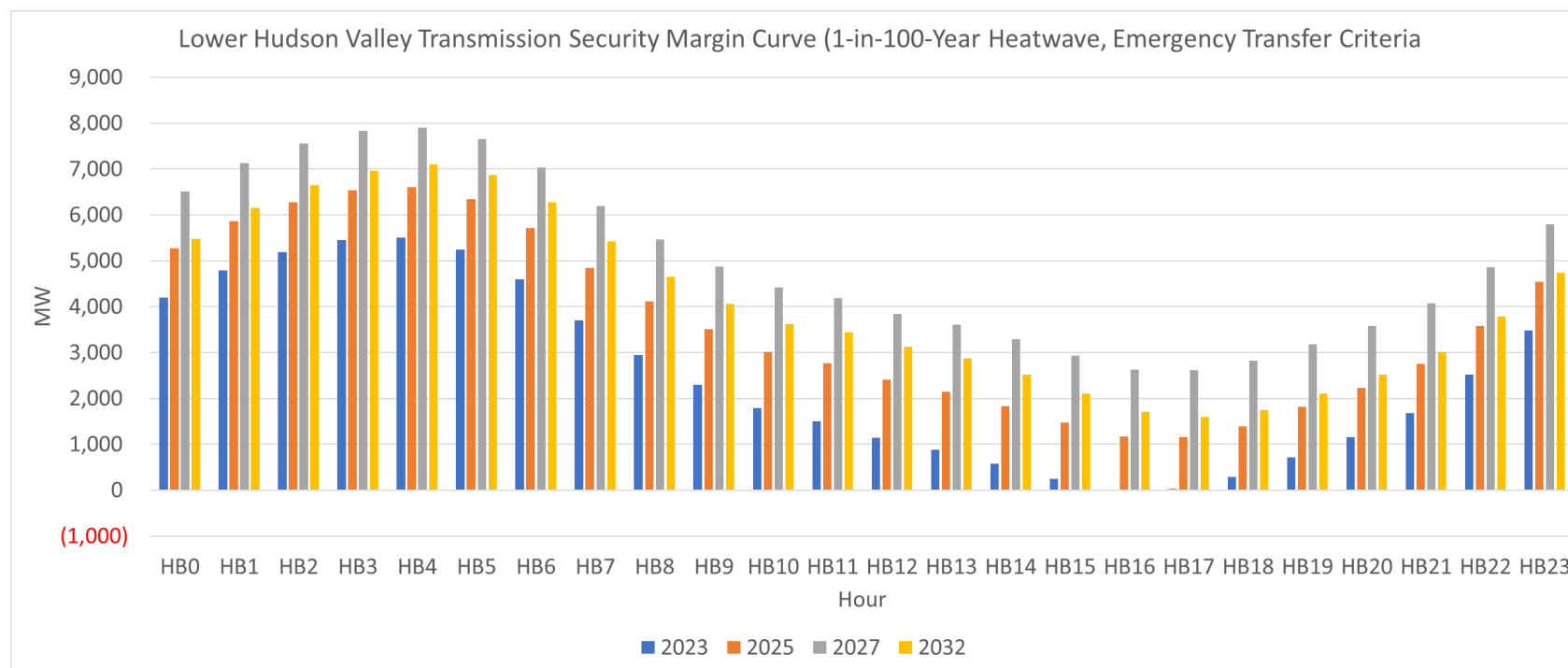
Figure 42: Lower Hudson Valley Transmission Security Margin Hourly Curve (1-in-100-Year Extreme Heatwave, Emergency Transfer Criteria)
