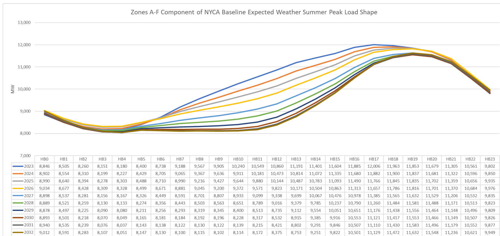
Figure 82: Zones A-F Component of NYCA Baseline Expected Weather Summer Peak Load shape
