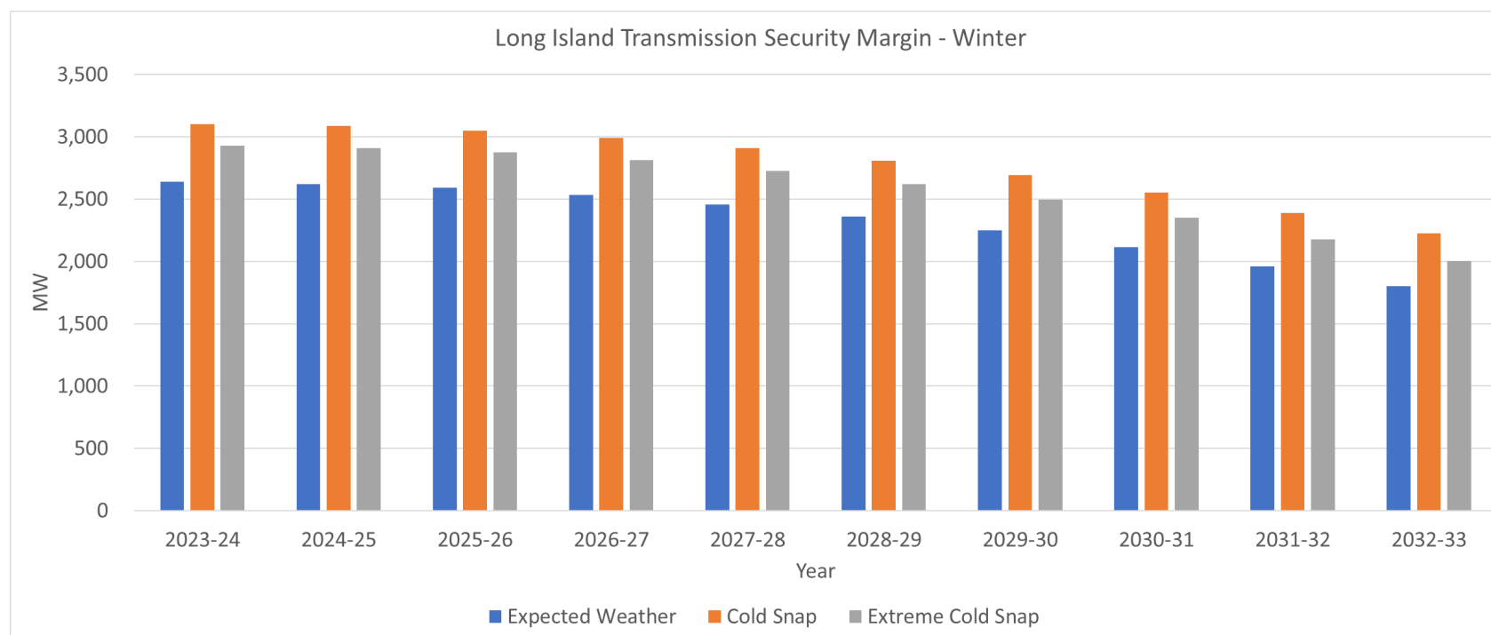
Figure 79: Summary of Long Island Summer Transmission Security Margin – Winter
