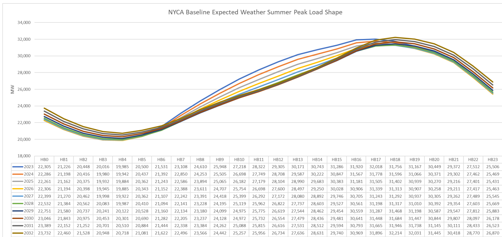
Figure 81: NYCA Baseline Expected Weather Summer Peak Load shape
