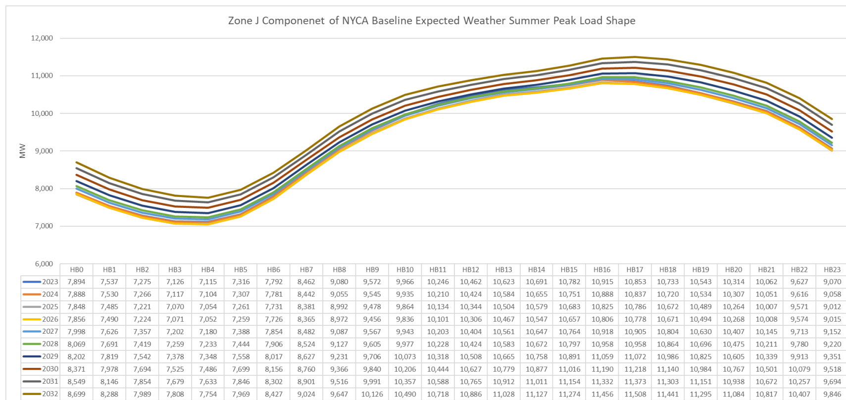
Figure 84: Zone J Component of NYCA Baseline Expected Weather Summer Peak Load shape
