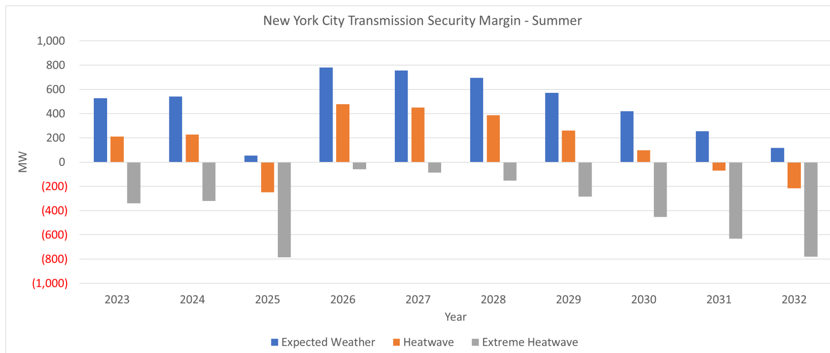
Figure 62: Summary of New York City Summer Transmission Security Margin – Summer
