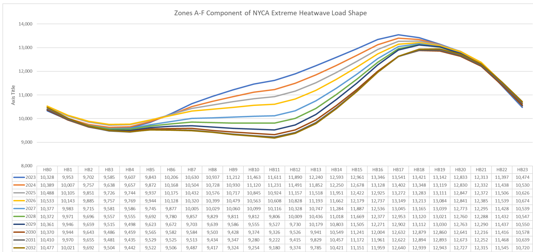
Figure 92: Zones A-F Component of NYCA Extreme Heatwave Load shape
