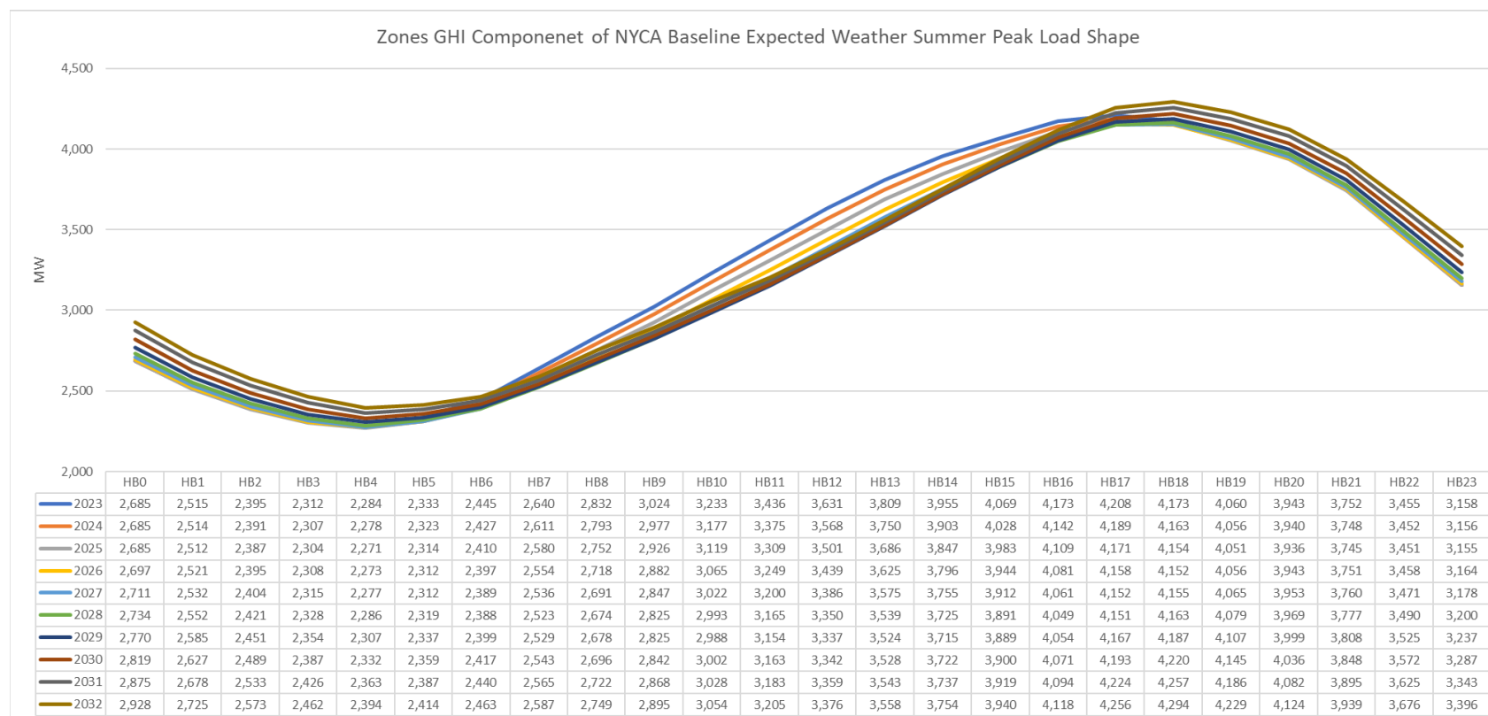
Figure 83: Zones GHI Component of NYCA Baseline Expected Weather Summer Peak Load shape
