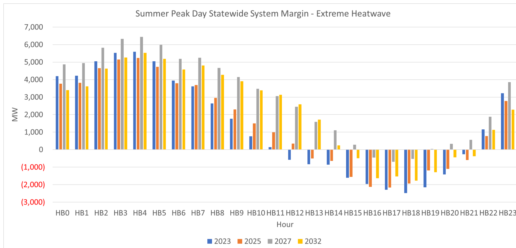
Figure 27: Statewide System Margin Hourly Curve (1-in-100-Year Extreme Heatwave, Emergency Transfer Criteria)
