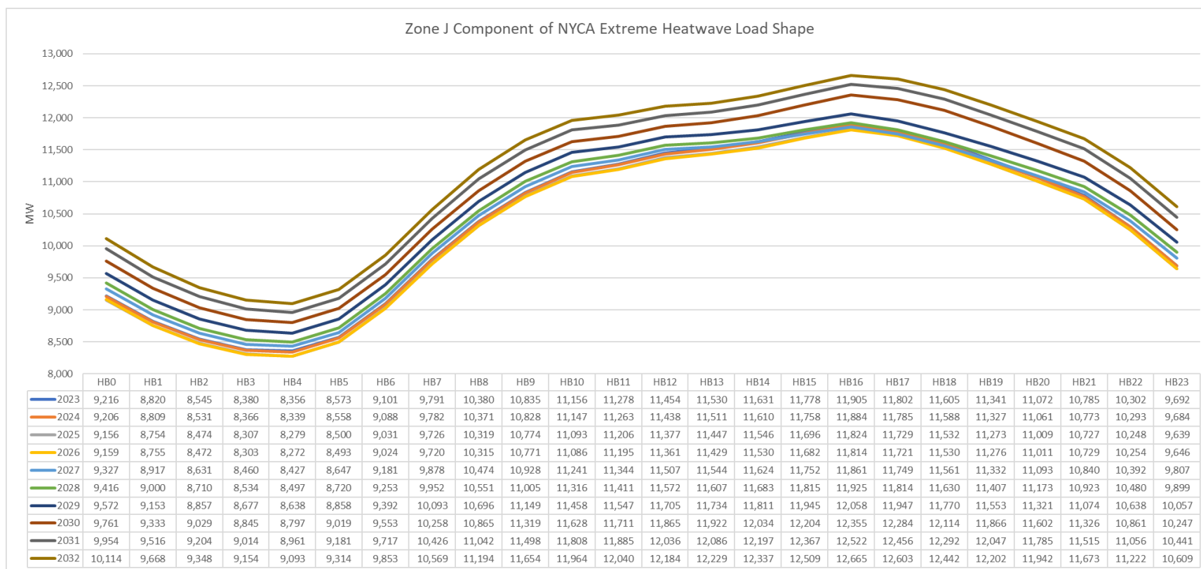
Figure 94: Zone J Component of NYCA Extreme Heatwave Load shape
