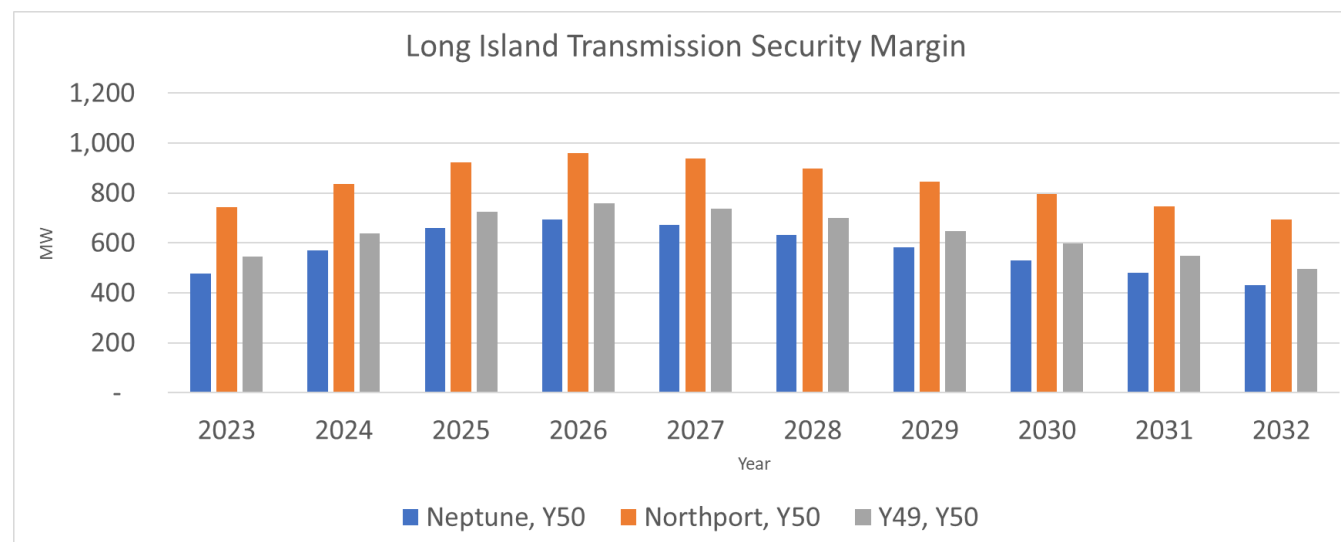
Figure 64: Impact of Contingency Combination on Zone K Transmission Security Margin
