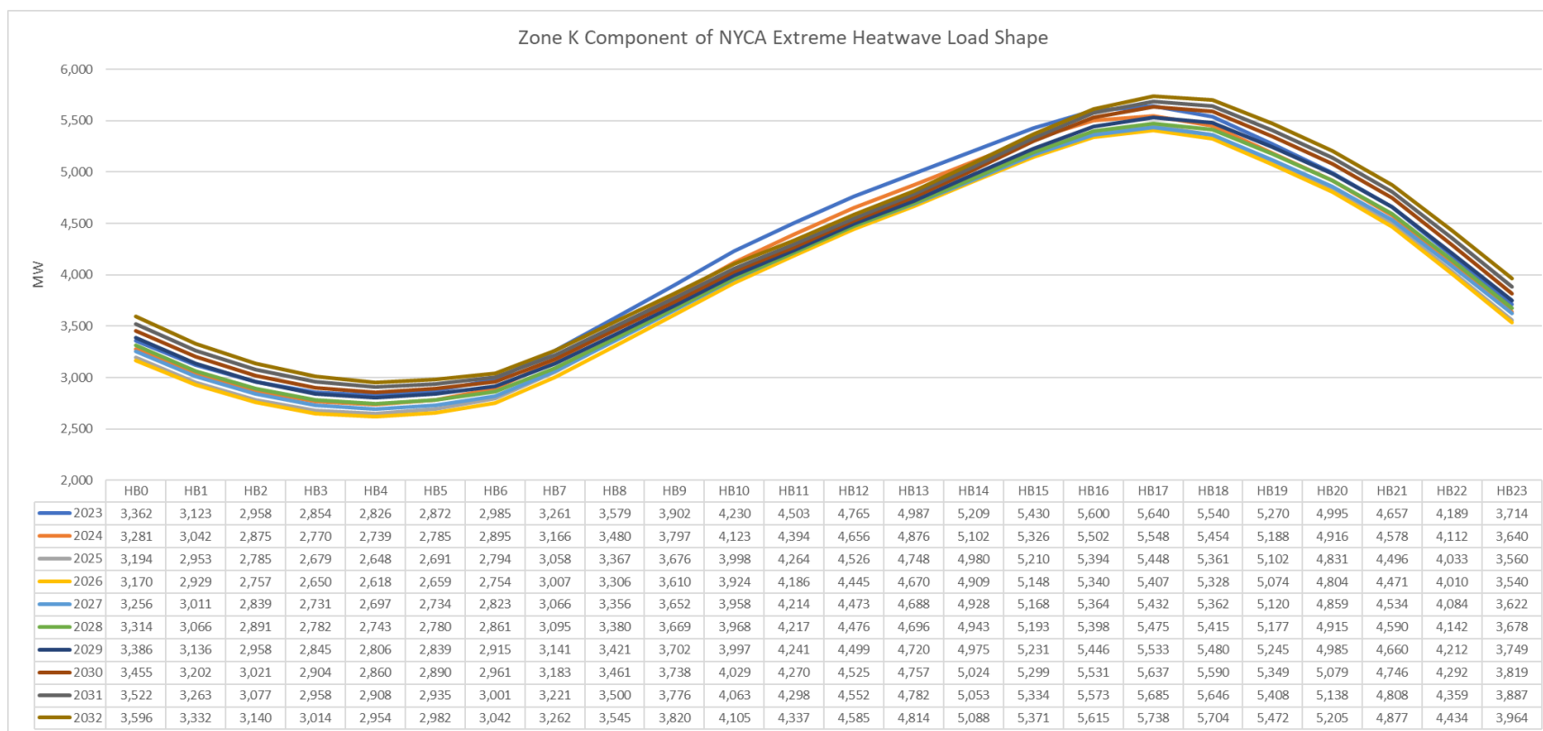
Figure 95: Zone K Component of NYCA Extreme Heatwave Load shape
