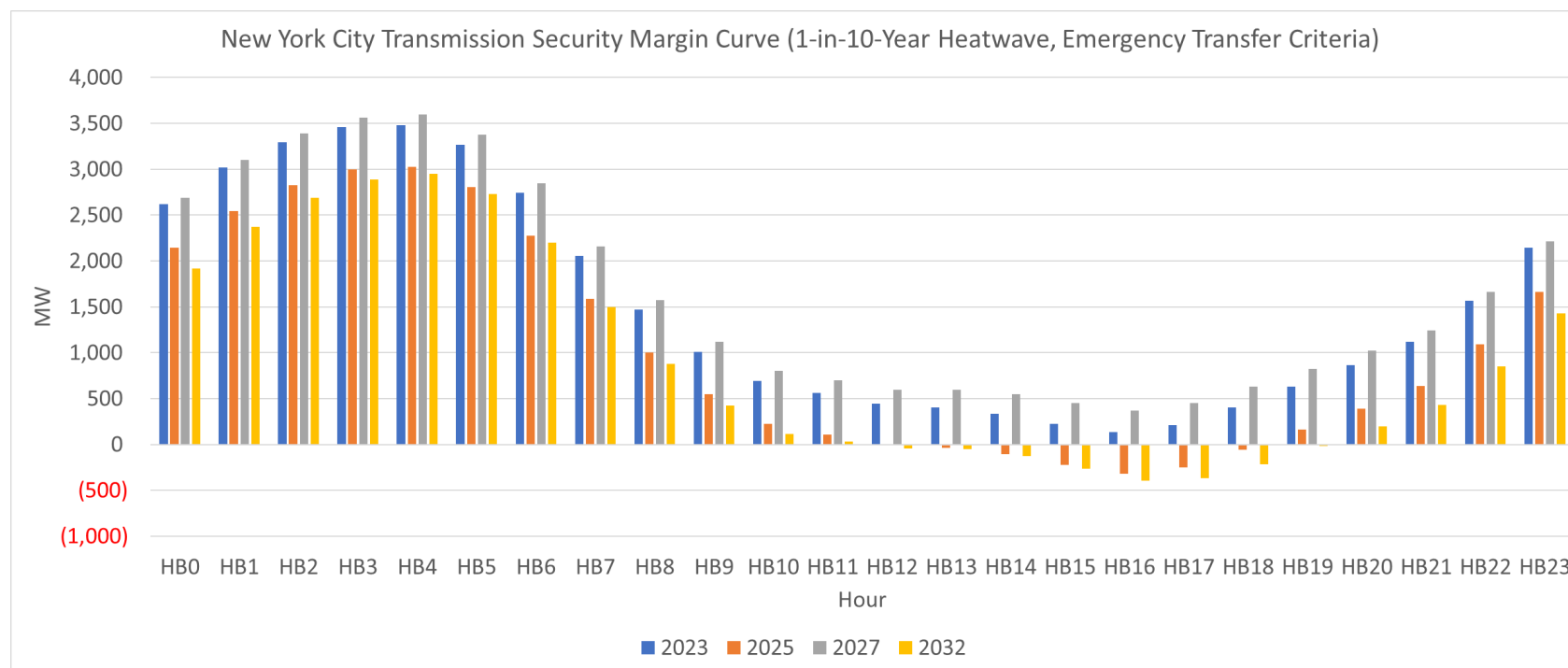
Figure 54: New York City Transmission Security Margin Hourly Curve (1-in-10-Year Heatwave, Emergency Transfer Criteria)
