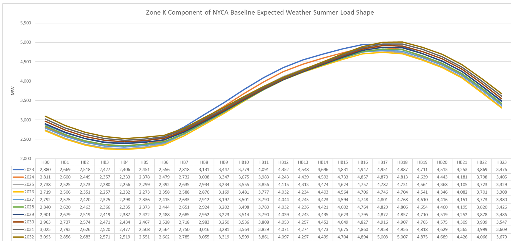
Figure 85: Zone K Component of NYCA Baseline Expected Weather Summer Peak Load shape
