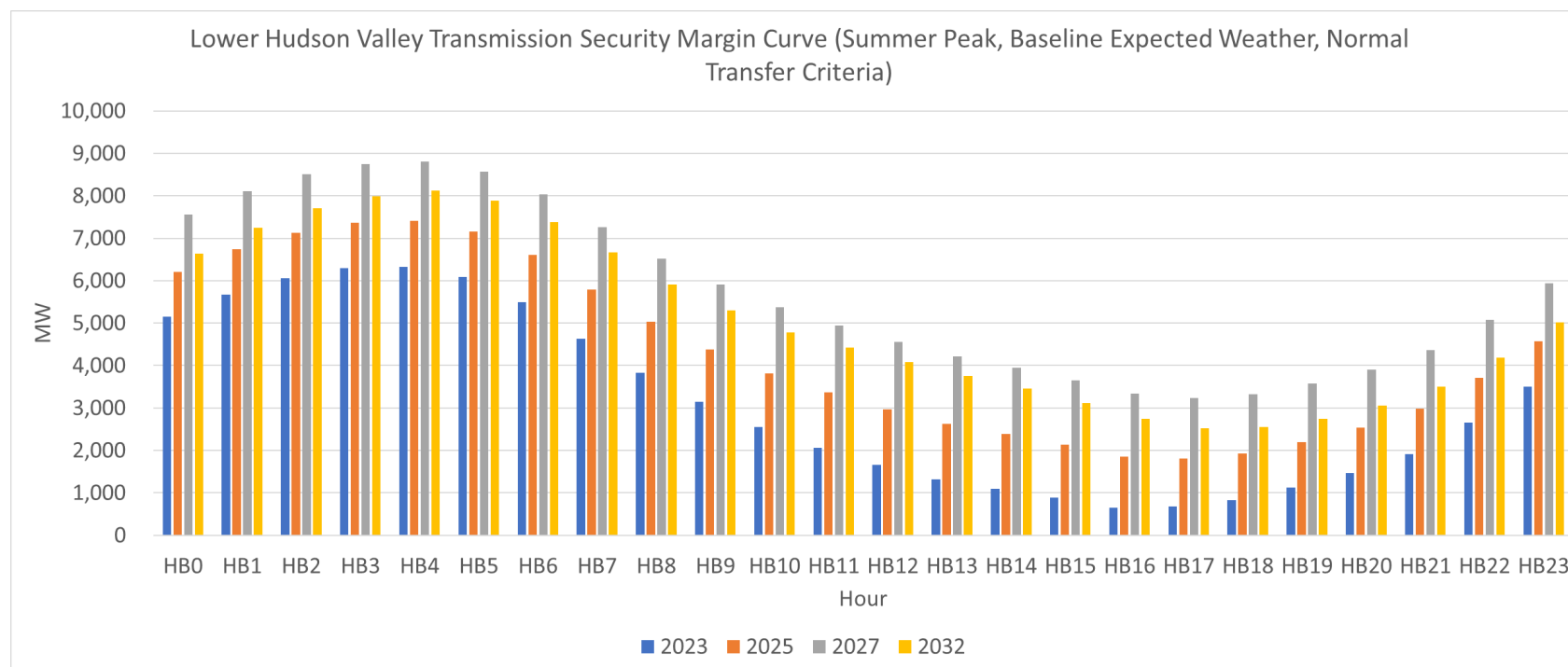
Figure 36: Lower Hudson Valley Transmission Security Margin Hourly Curve (Summer Peak – Baseline Expected Weather, Normal Transfer Criteria)
