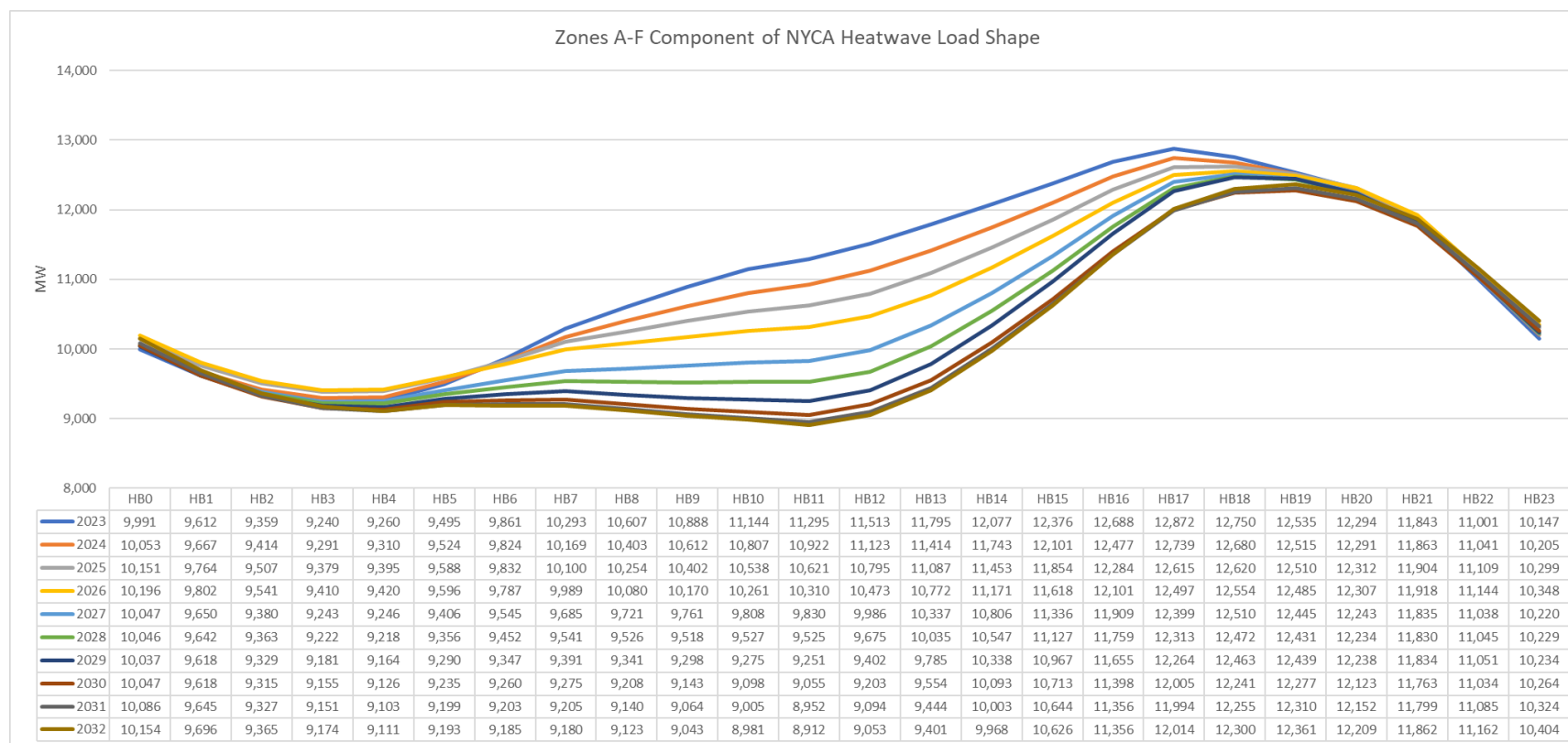
Figure 87: Zones A-F Component of NYCA Heatwave Load shape
