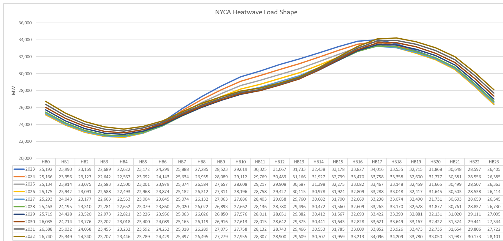
Figure 86: NYCA Heatwave Load shape
