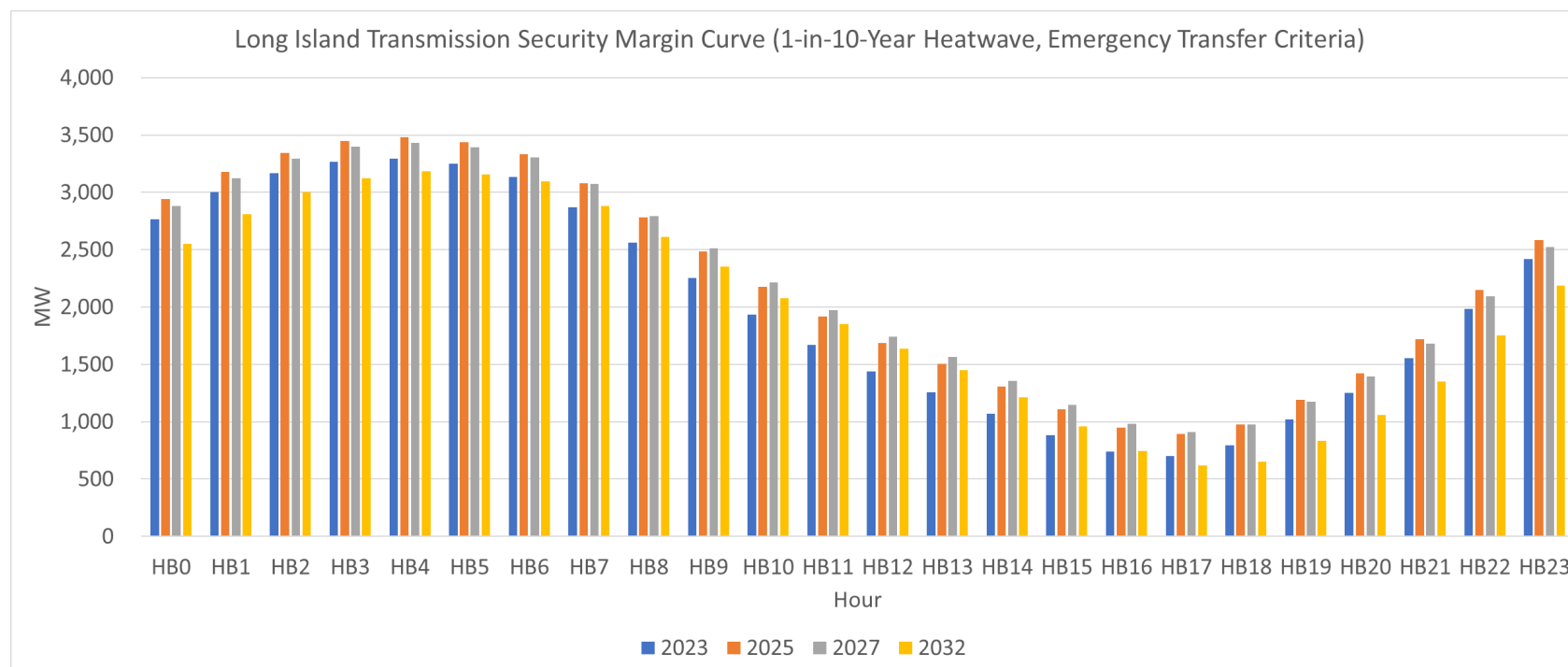
Figure 70: Long Island Transmission Security Margin Hourly Curve (1-in-10-Year Heatwave, Emergency Transfer Criteria)
