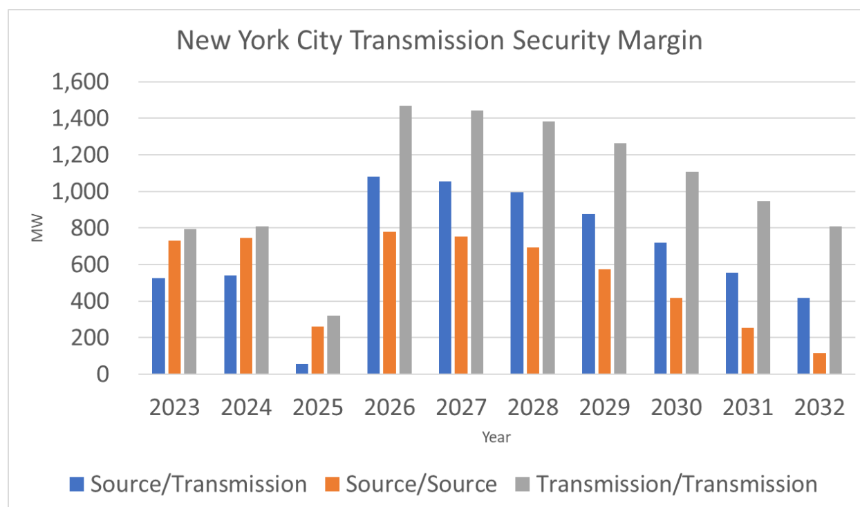
Figure 48: Impact of Contingency Combination on Zone J Transmission Security Margin
