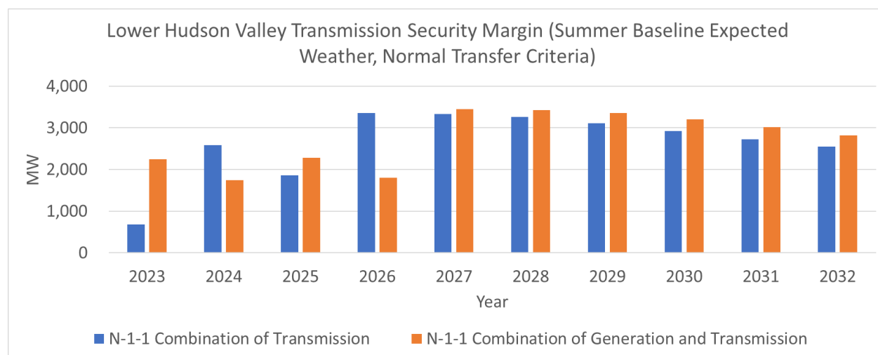
Figure 33: Lower Hudson Valley Transmission Security Margin (Summer Baseline Peak Forecast – Expected Weather)
