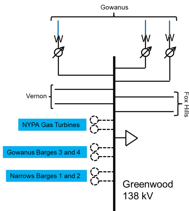
Figure 20: Greenwood 138 kV TLA
