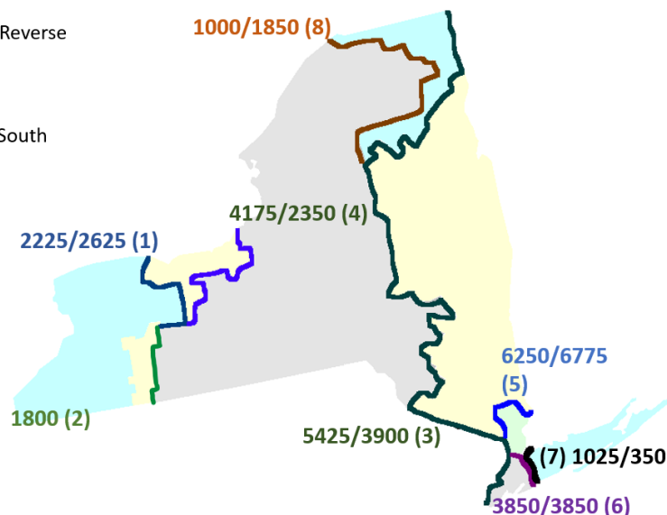
Figure 1 – Cross-State Thermal Transfer Limits
