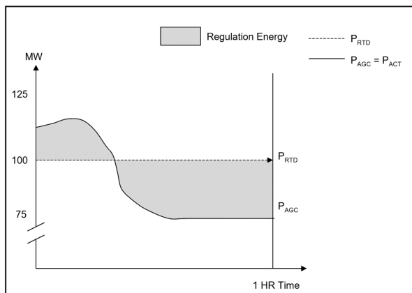
Figure 10: Perfect Performance
