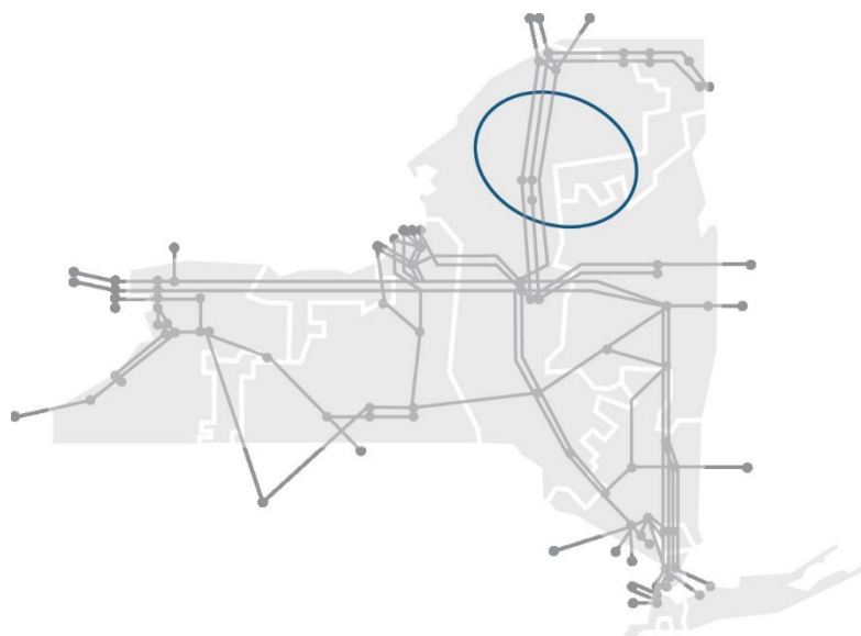
Figure 38: Northern New York Bulk Transmission
