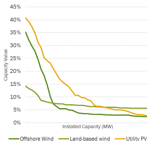
Figure 23: Renewable Resource Dynamic Capacity Value Curves: Illustrative Example 22
