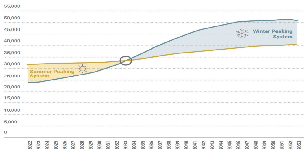
Figure 11: Peak Load Forecast for Summer & Winter (MW)
