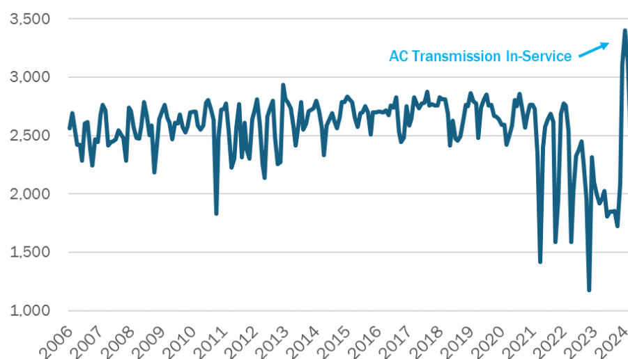
Figure 35: 2006-2024 Central East Maximum Month Flow (MW)
