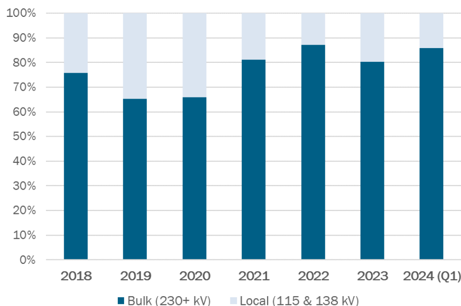
Figure 34: Historic Annual Bulk vs Local Transmission Congestion
