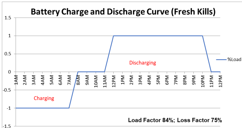
Figure 2 Battery Charge and Discharge Curve (Fresh Kills)
