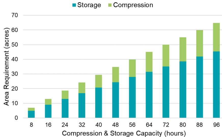
Figure 4: Hydrogen Storage & Compression Space Requirement
