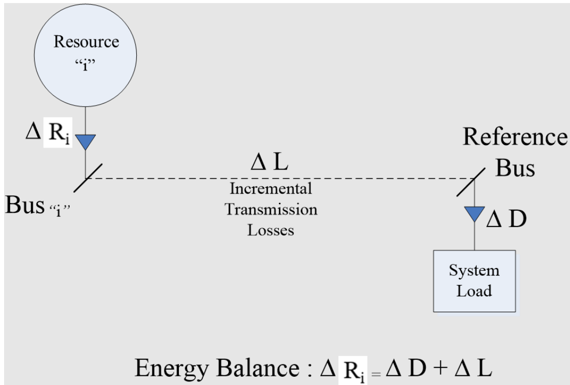
Figure 7 Figure 6 : Incremental Transmission Losses
