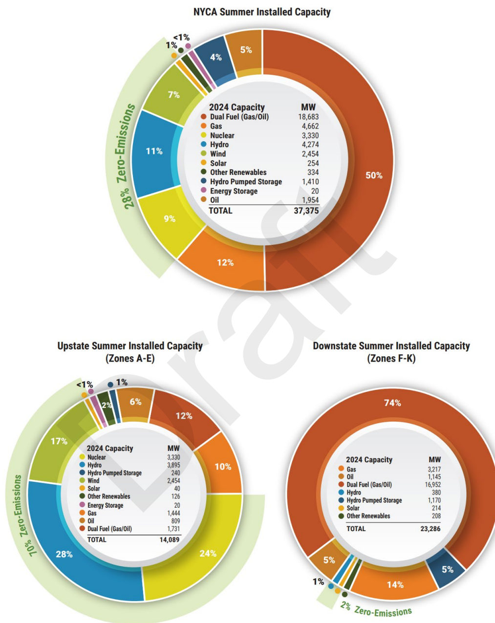
Figure 5: Summer Installed Capacity (MW) by Fuel Source – Statewide, Upstate, & Downstate New York: 2024
