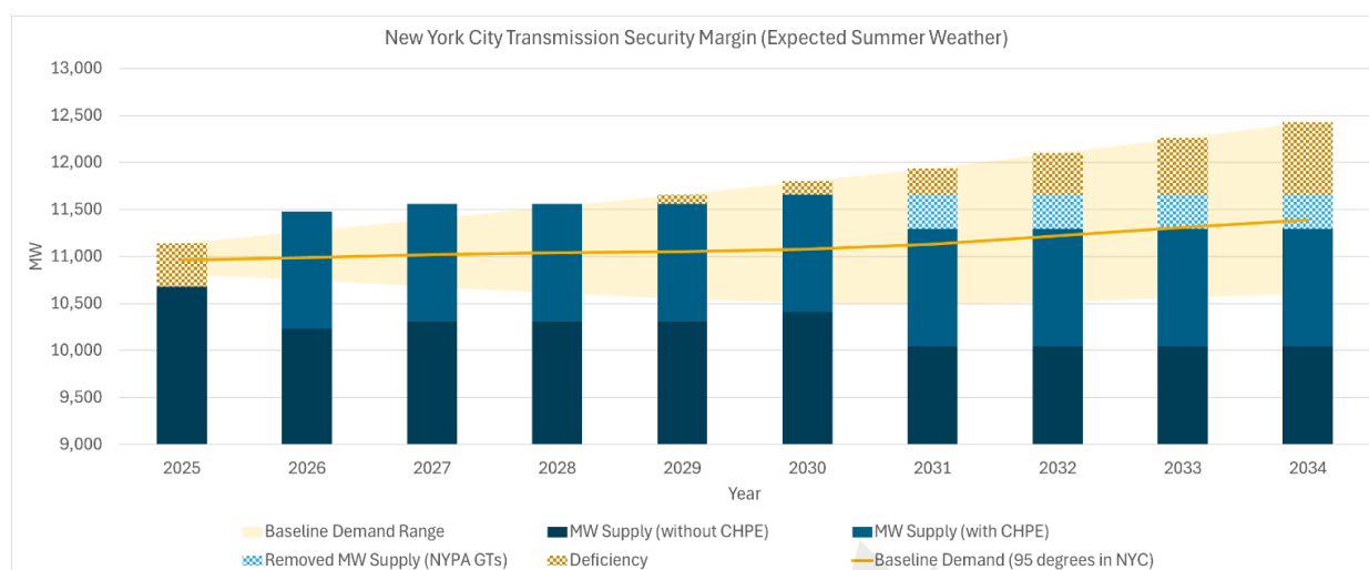
Figure 1: New York City Margin Forecast Uncertainty
