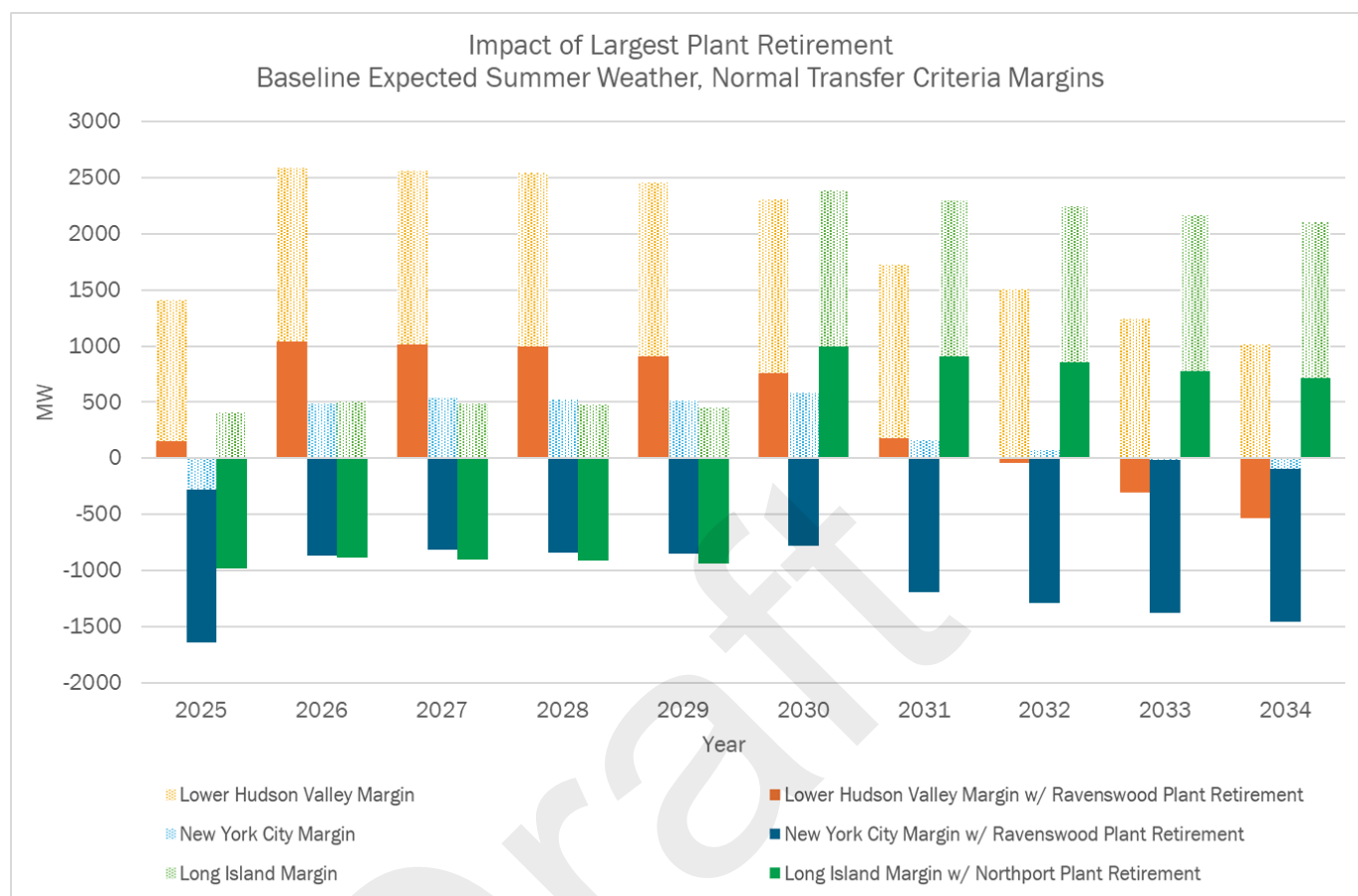
Figure 39: Impact of Potential Retirements
