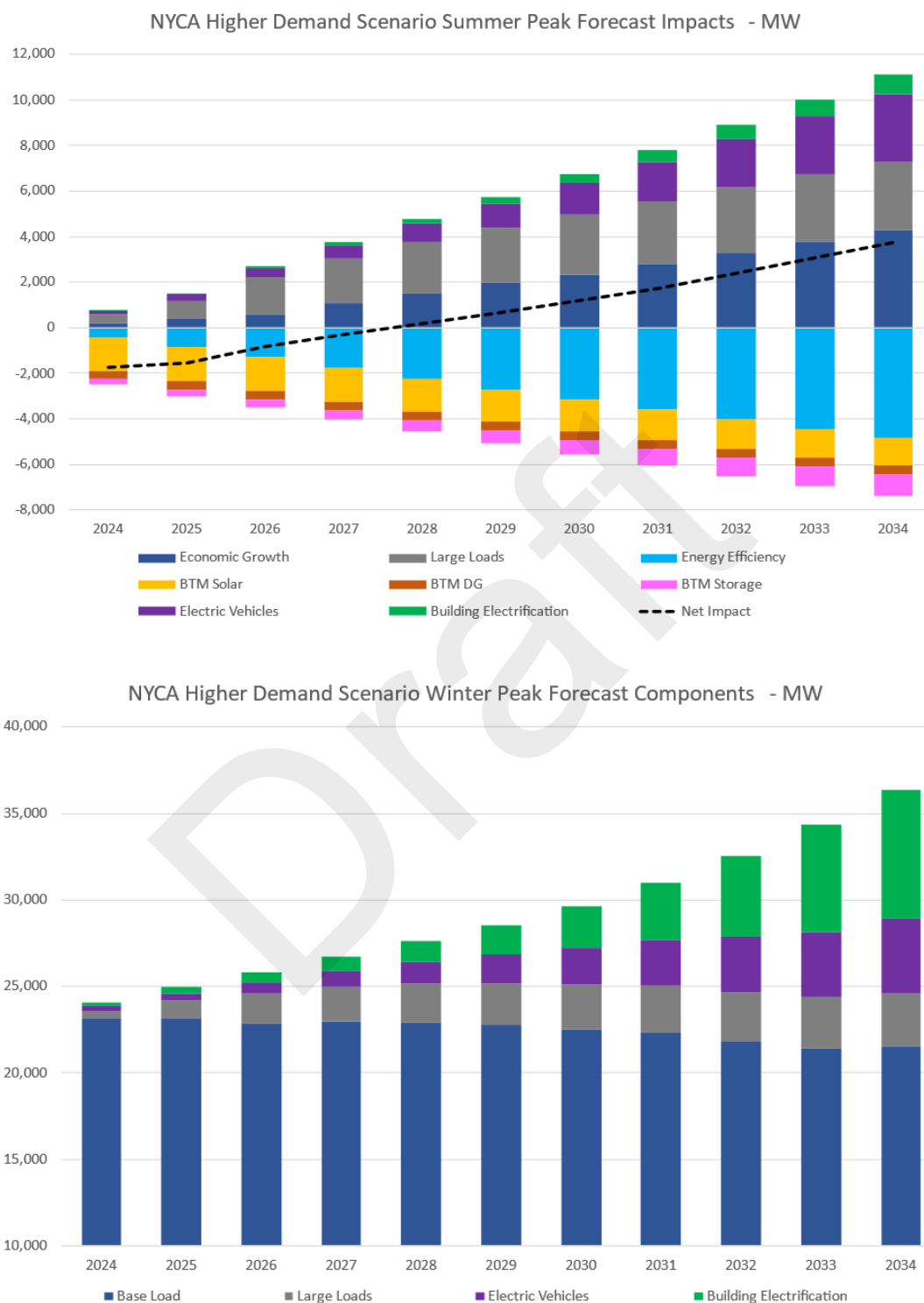
Figure 14: Higher Demand Scenario Peak Forecast Impacts
