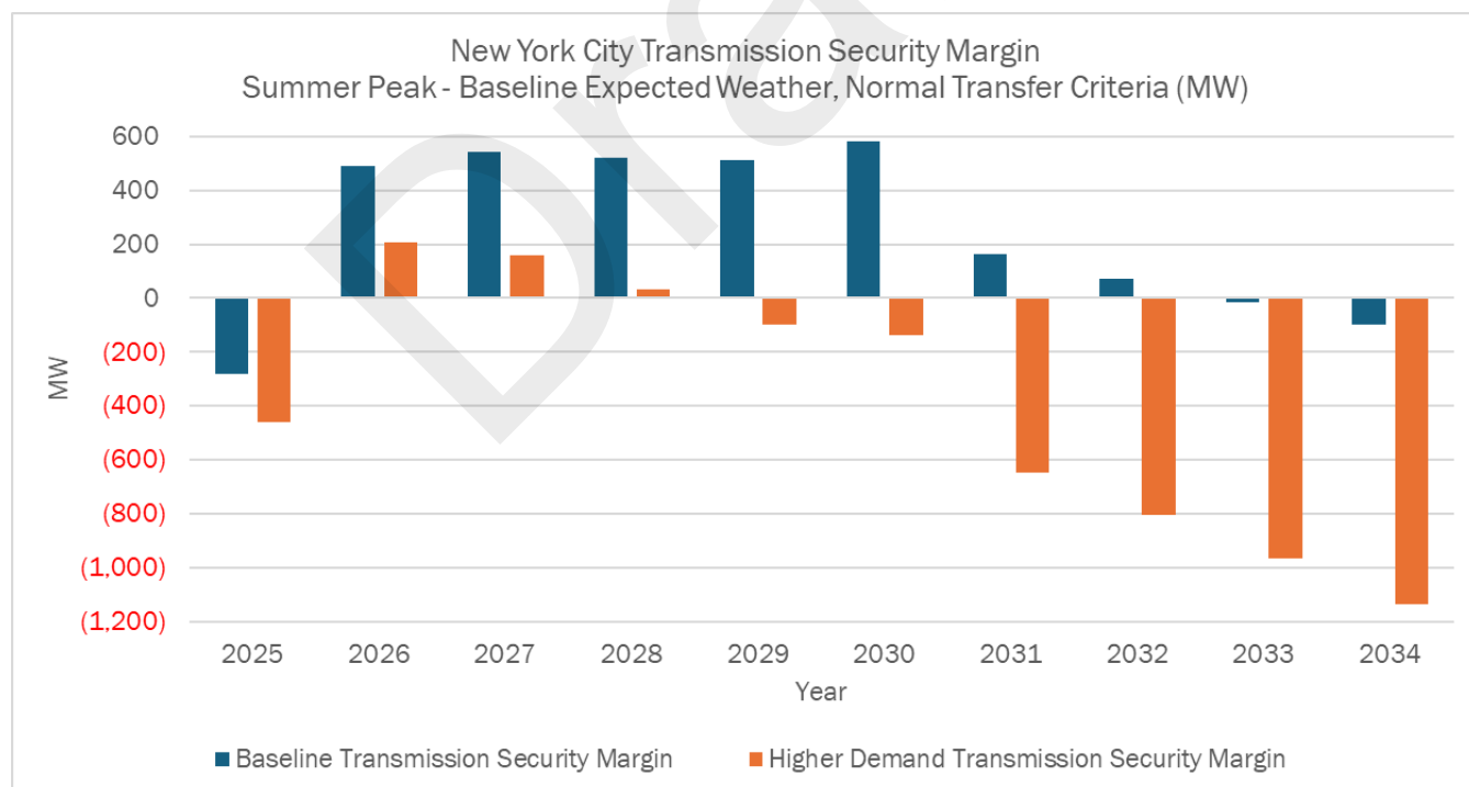
Figure 29: New York City Transmission Security Margin
