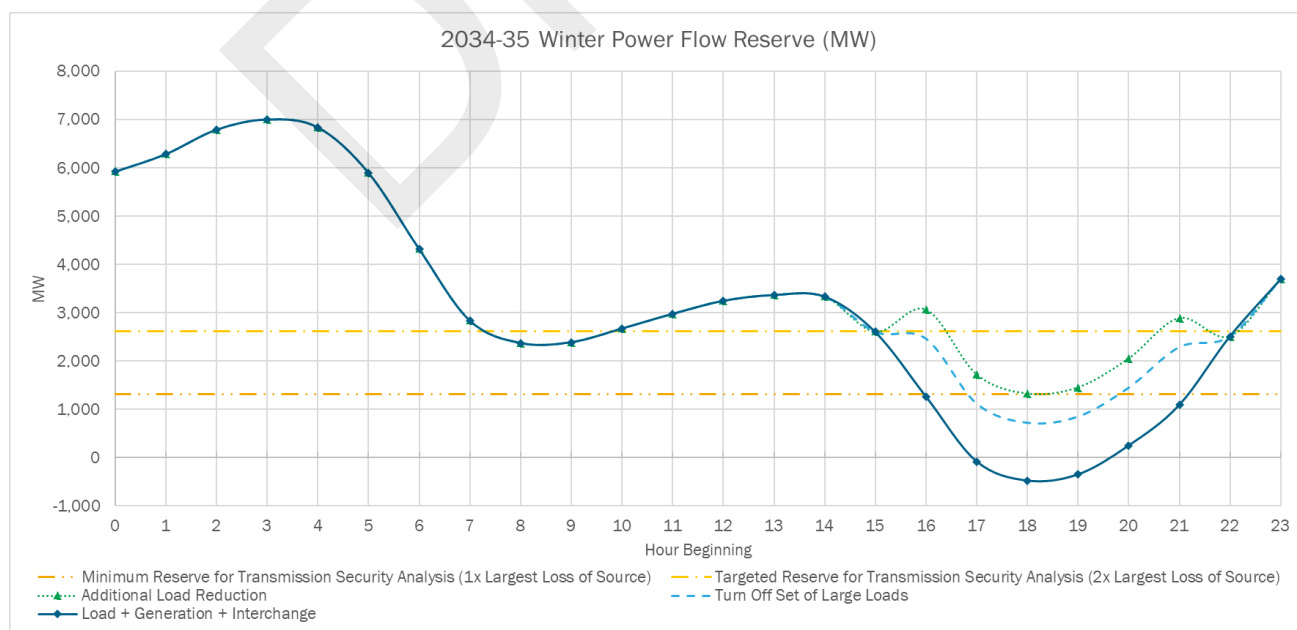
Figure 26: 2034-2035 Winter Peak Day Reserve Levels
