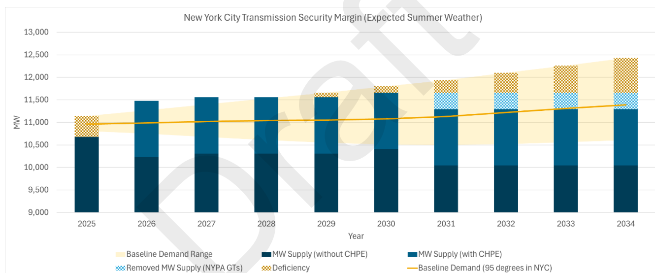
Figure 40: New York City Margin Forecast Uncertainty
