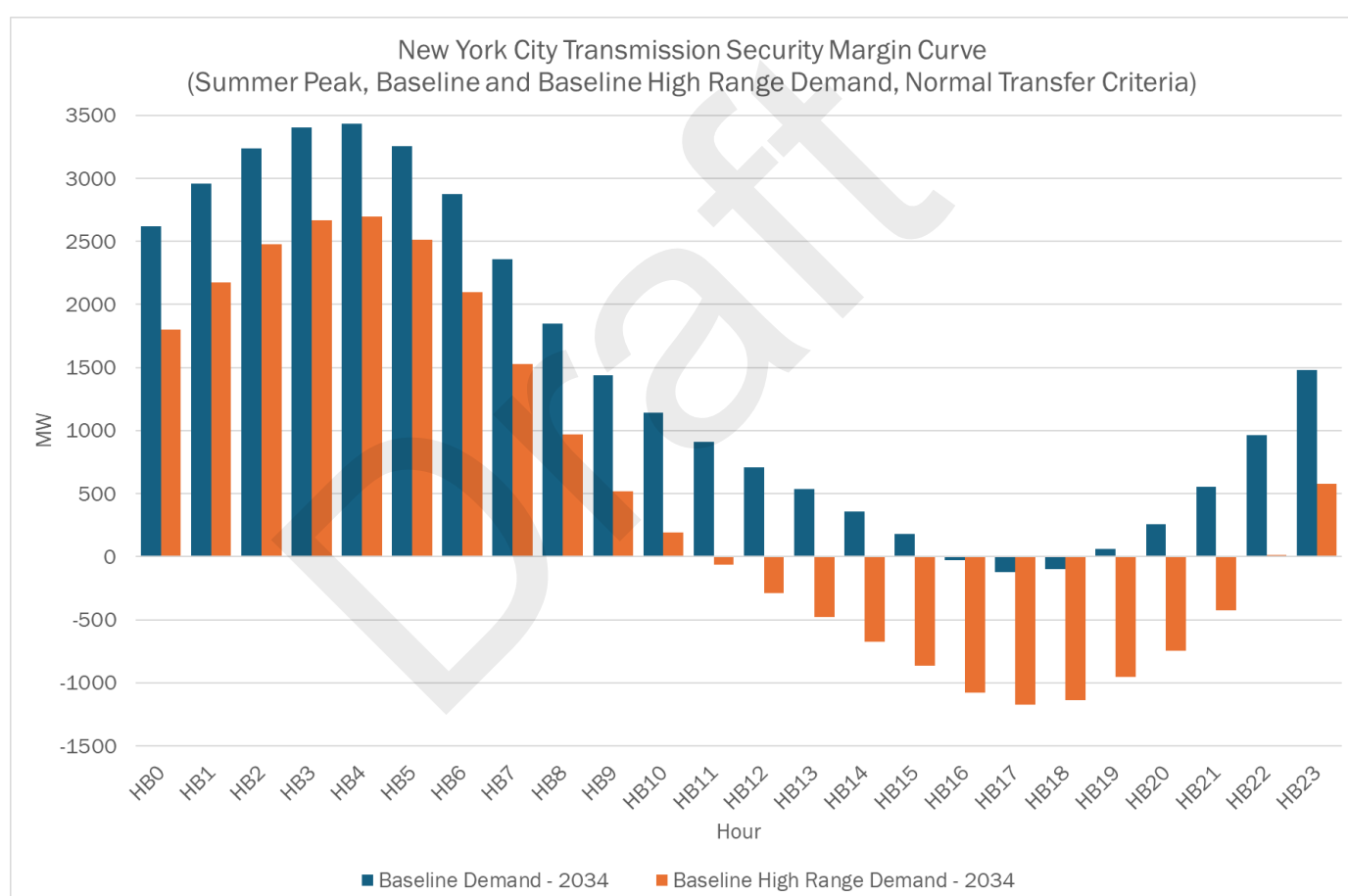
Figure 30: New York City Transmission Security Margin Hourly Curve - 2034
