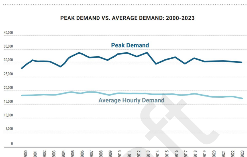
Figure 8: Historical Average Hourly Demand versus Actual Yearly Summer Peak Demand
