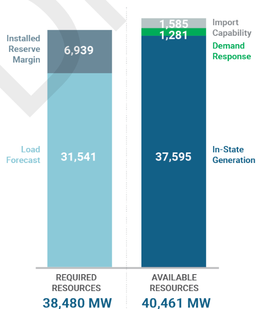
Figure 7: Statewide Resource Availability: Summer 2024
