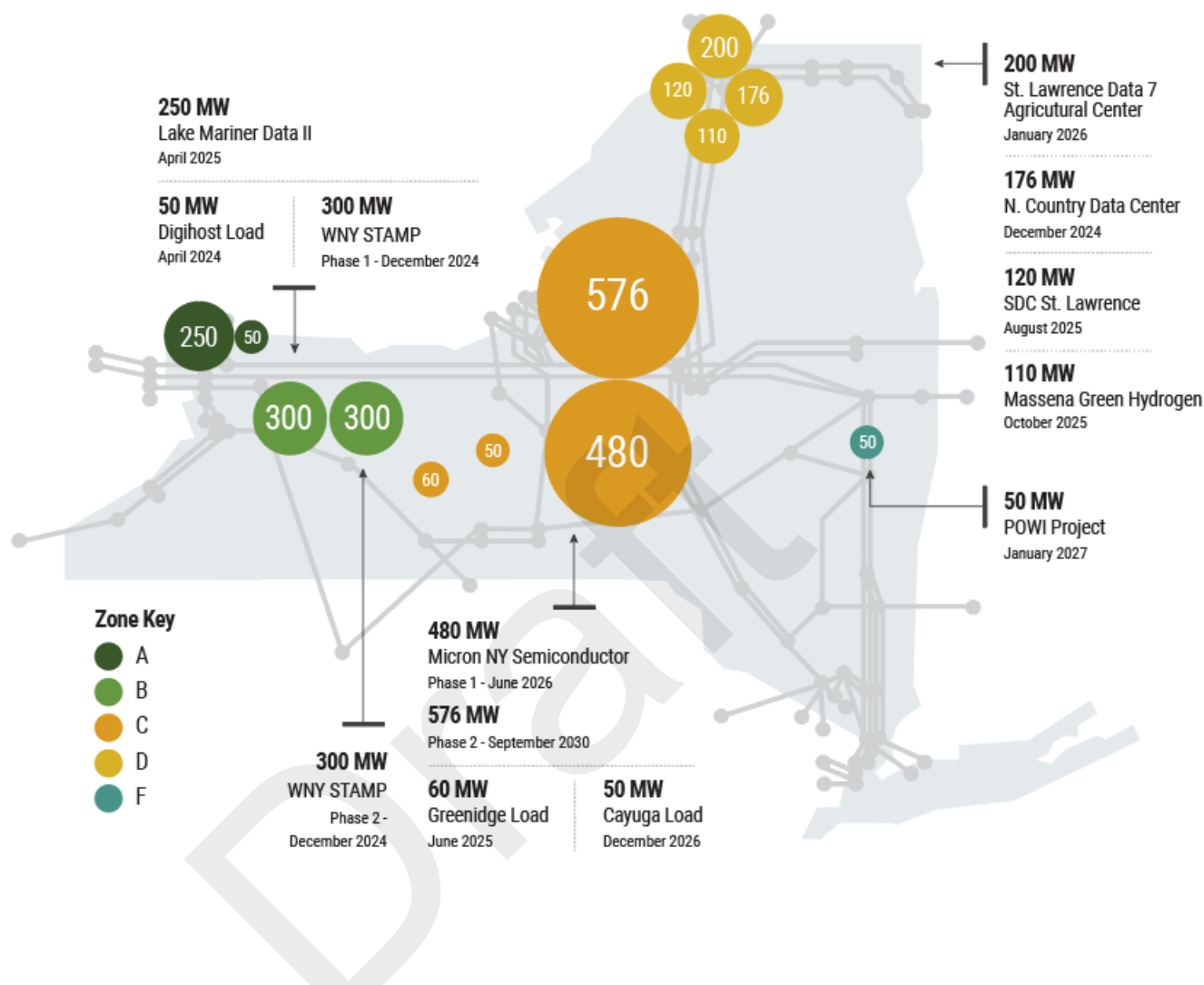
Figure 16: RNA Large Load Forecast Assumptions
