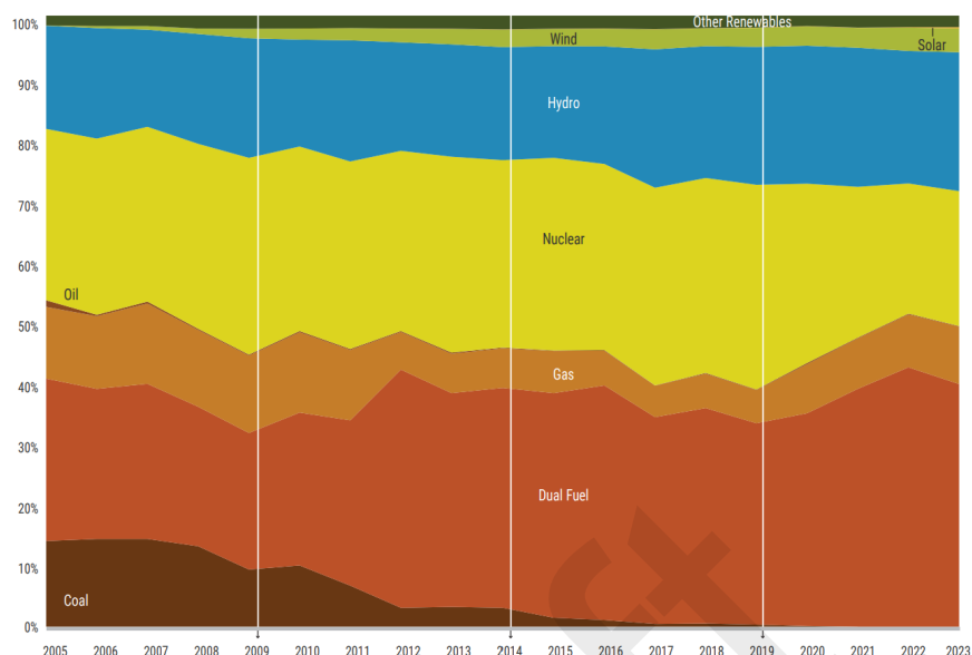
Figure 9: Historical Generating Capacity Fuel Mix in New York State: 2005-2023
