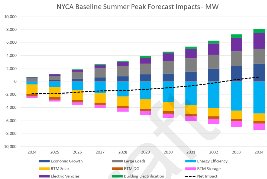
Figure 13: Baseline Peak Forecast Impacts
