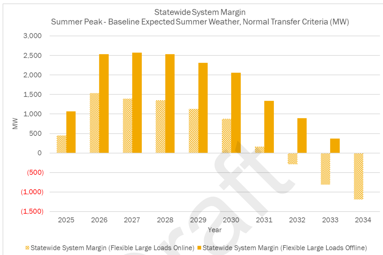
Figure 24: Summer Peak Statewide System Margin
