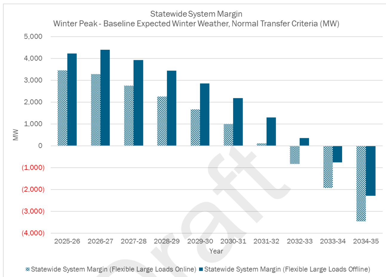
Figure 25: Winter Peak Statewide System Margin
