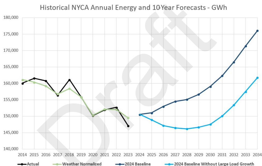
Figure 17: Large Load Impact on NYCA Baseline Load Forecast
