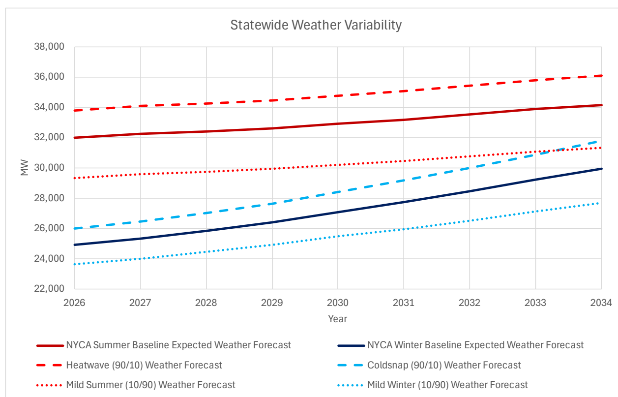
Figure 21: Weather Variability
