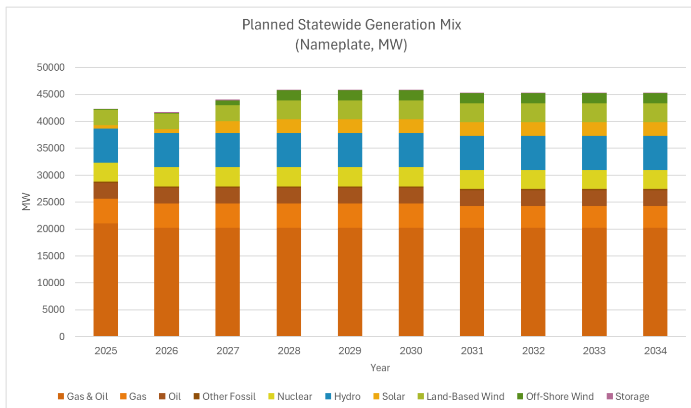
Figure 11: Planned Statewide Generation Mix
