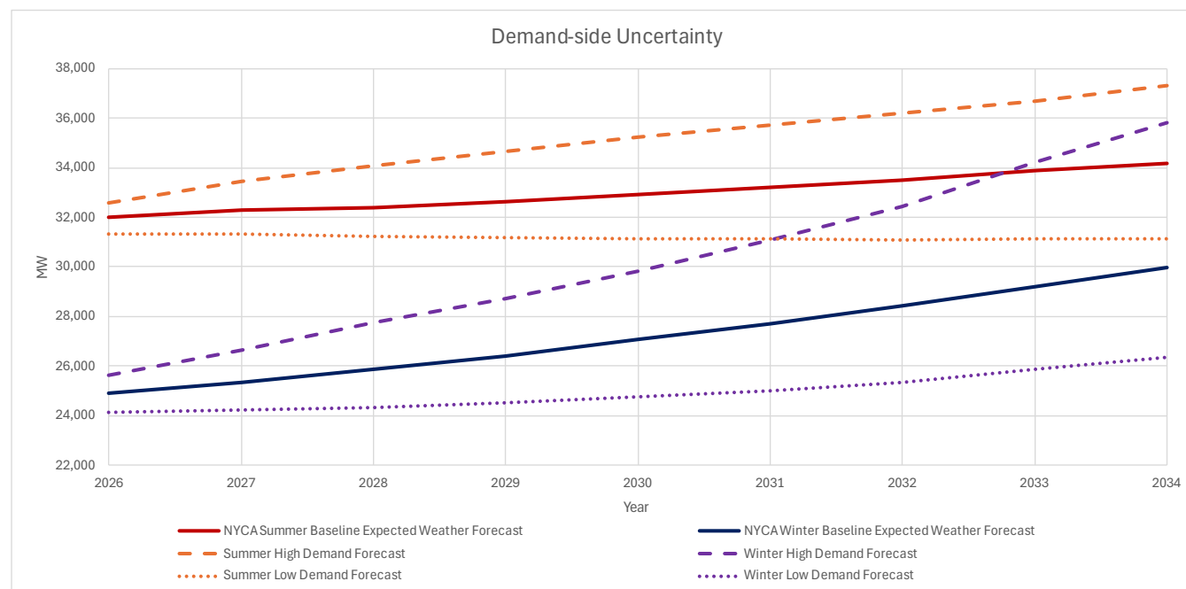
Figure 10 2026-2034 Demand Forecasts
