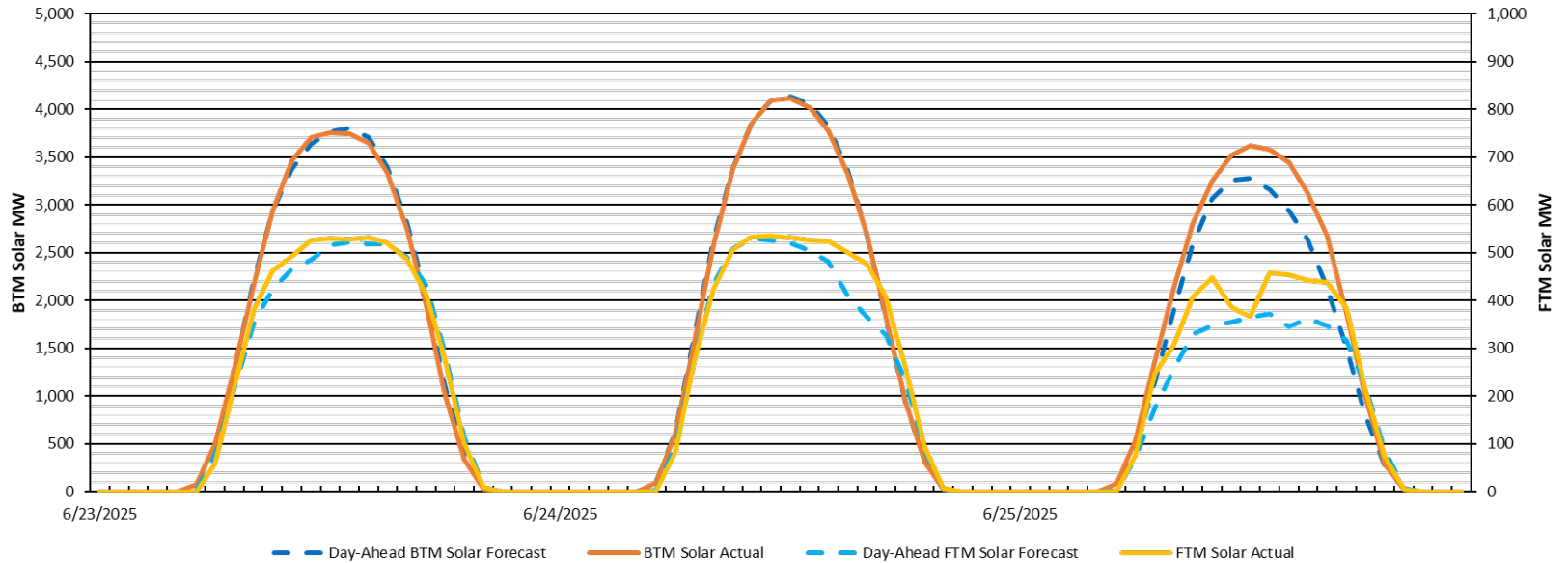
NYCA Solar Profile 6/23 - 6/25 Installed Capacities - Est BTM: ~6,411 MW FTM: 571 MW
