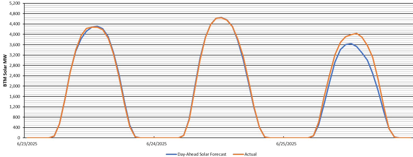
NYCA Solar Profile (~6,411 MW BTM & 571 MW FTM) 6/23 - 6/25
