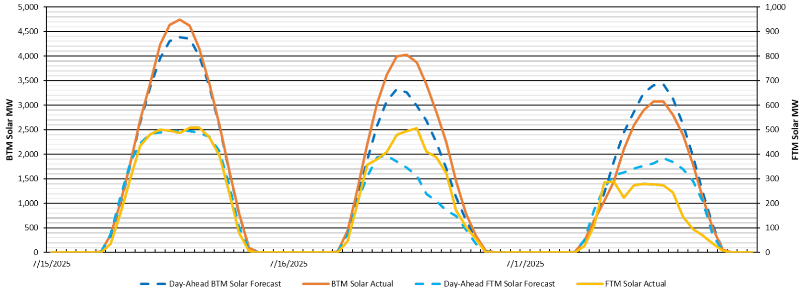
NYCA Solar Profile 7/15 - 7/17 Installed Capacities - Est BTM: ~6,470 MW FTM: 571 MW
