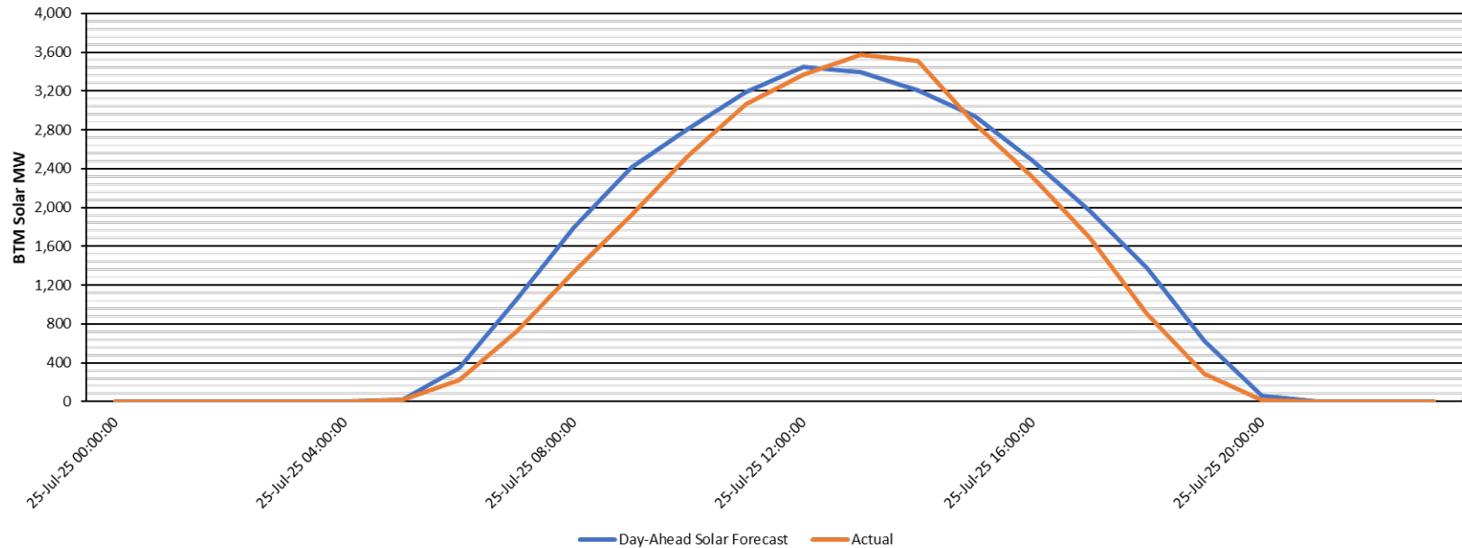
NYCA Solar Profile (~6,470 MW BTM & 571 MW FTM) 7/25
