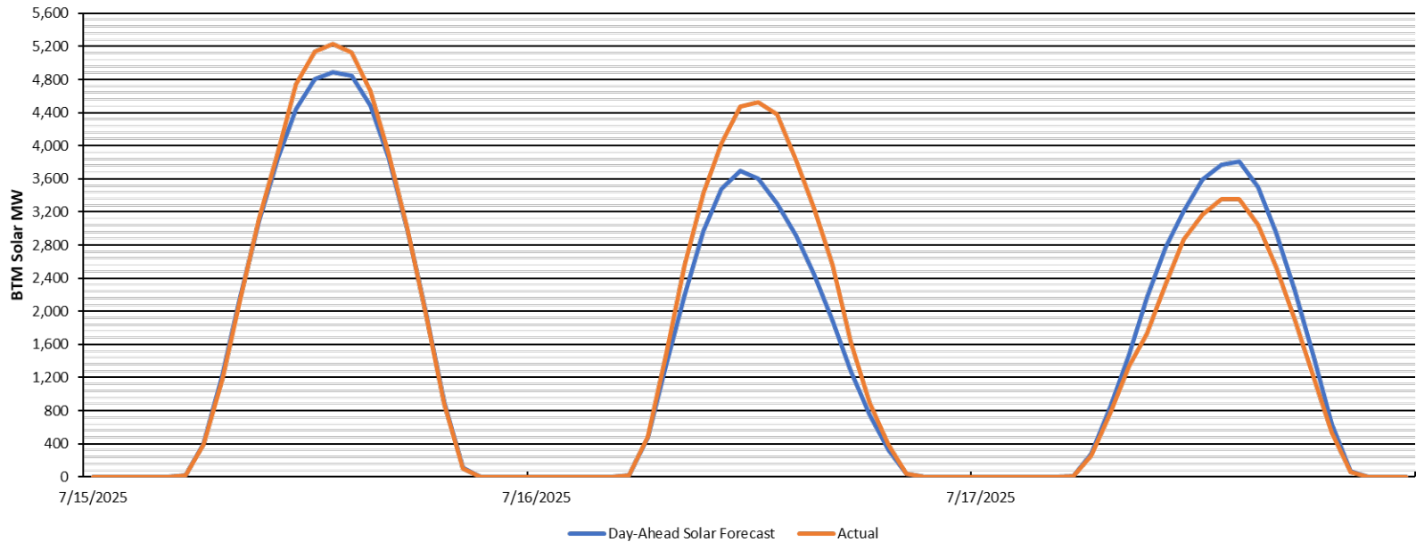
NYCA Solar Profile (~6,470 MW BTM & 571 MW FTM) 7/15 - 7/17
