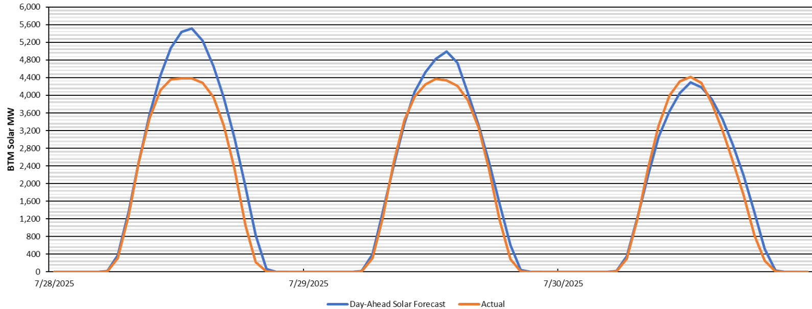
NYCA Solar Profile (~6,470 MW BTM & 571 MW FTM) 7/28 - 7/30
