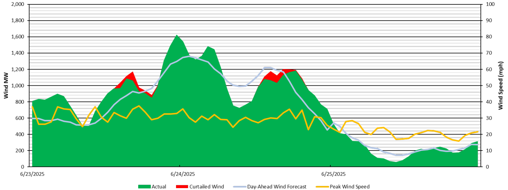
NYCA Wind Profile 6/23 - 6/25
