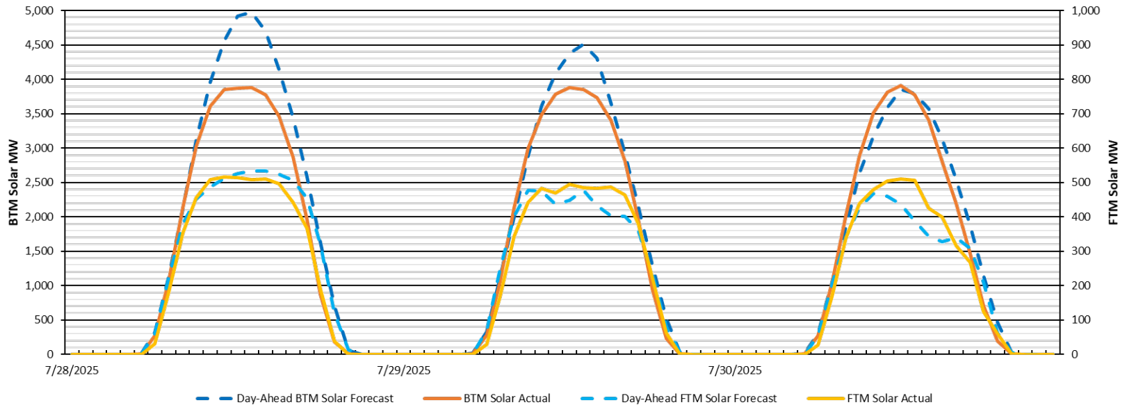
NYCA Solar Profile 7/28 - 7/30 Installed Capacities - Est BTM: ~6,470 MW FTM: 571 MW
