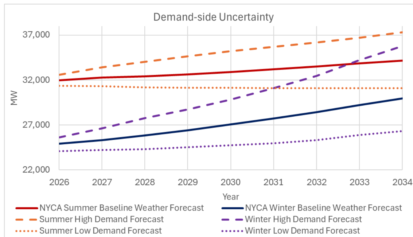
Figure 17: Demand-Side Uncertainty
