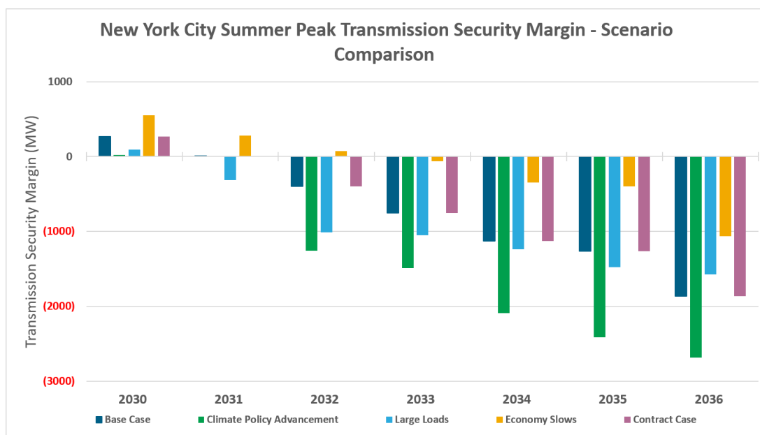
Figure 63: Scenario Summer New York City Transmission Security Margin
