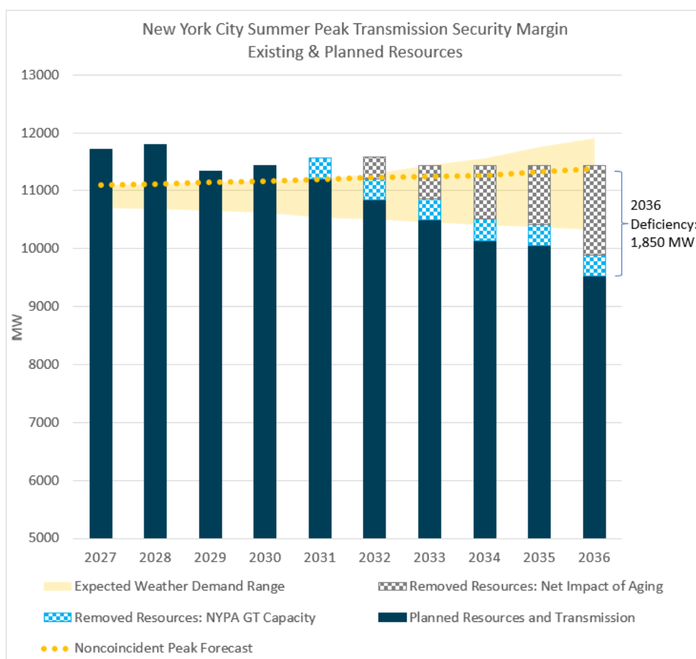
Figure 33: NYC Summer Peak Transmission Security Margin
