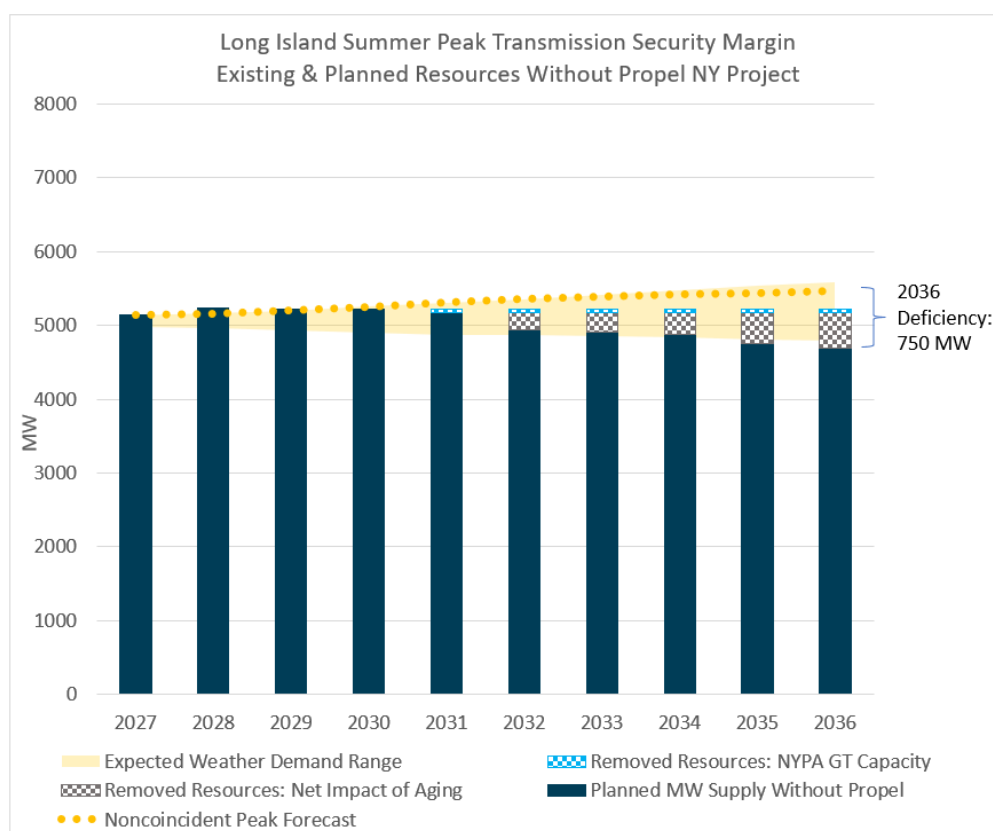
Figure 35: Long Island Transmission Security Margin without Propel NY
