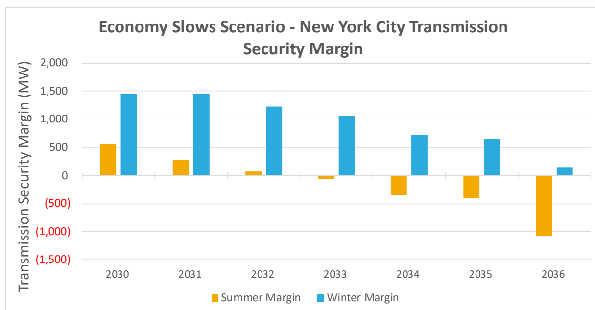
Figure 51: Economy Slows Scenario - New York City Transmission Security Margin
