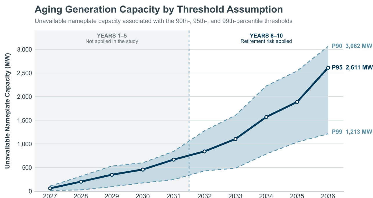
Figure 19: Aging generation trend - P90 vs P95 vs P99
