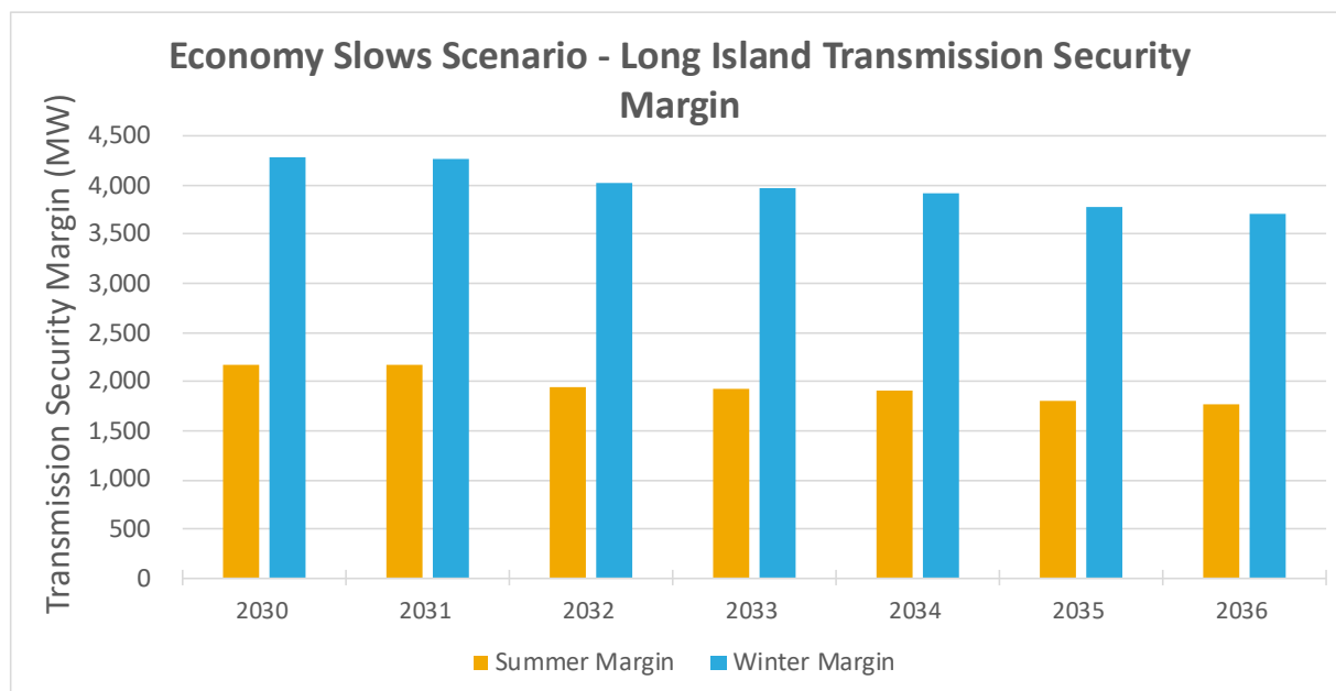
Figure 52: Economy Slows Scenario - Long Island Transmission Security Margin
