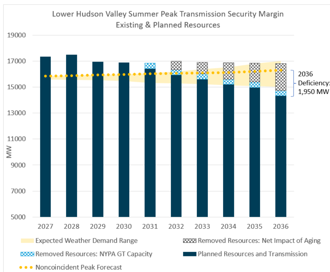
Figure 32: Lower Hudson Valley Summer Transmission Security Margin
