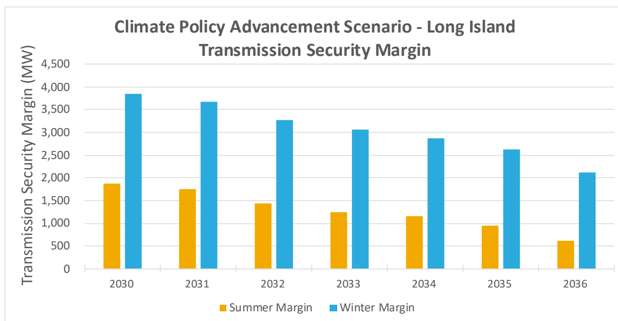
Figure 44: Climate Policy Advancement - Long Island Transmission Security Margin
