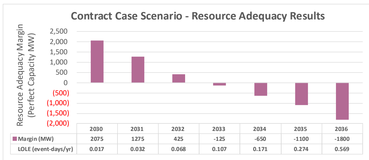
Figure 53: Contract Case Scenario - Resource Adequacy
