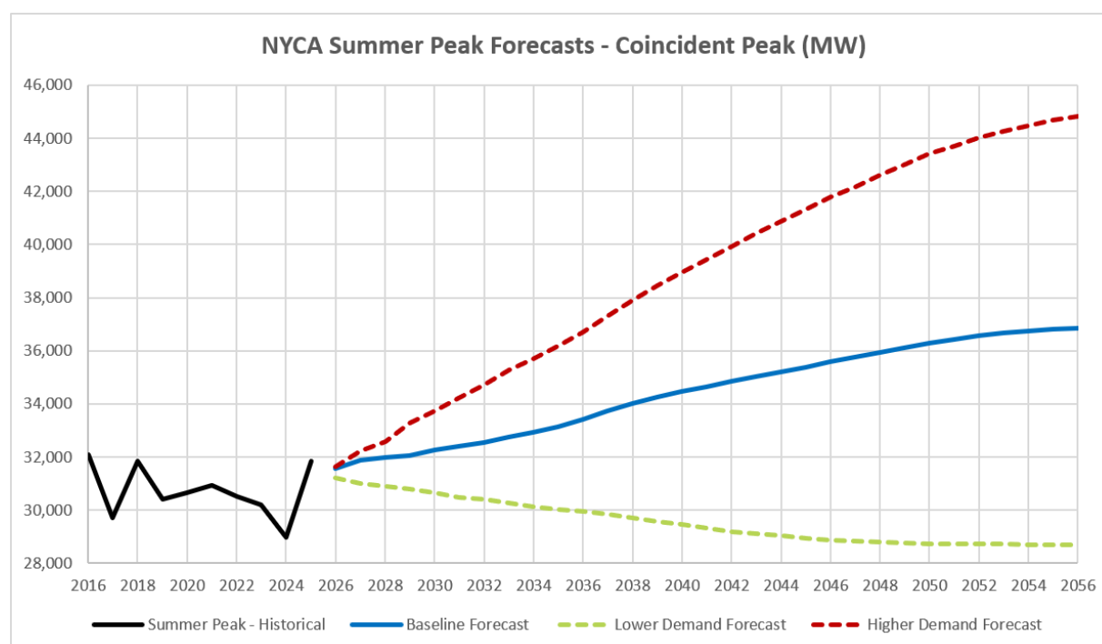
Figure 6: 30-Year NYCA Summer Peak Forecast
