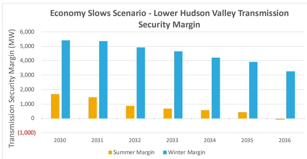
Figure 50: Economy Slows Scenario - Lower Hudson Valley Transmission Security Margin
