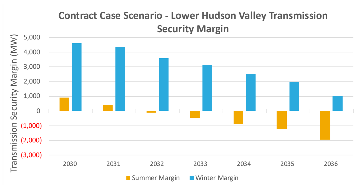
Figure 54: Contract Case Scenario - Lower Hudson Valley Transmission Security Margin
