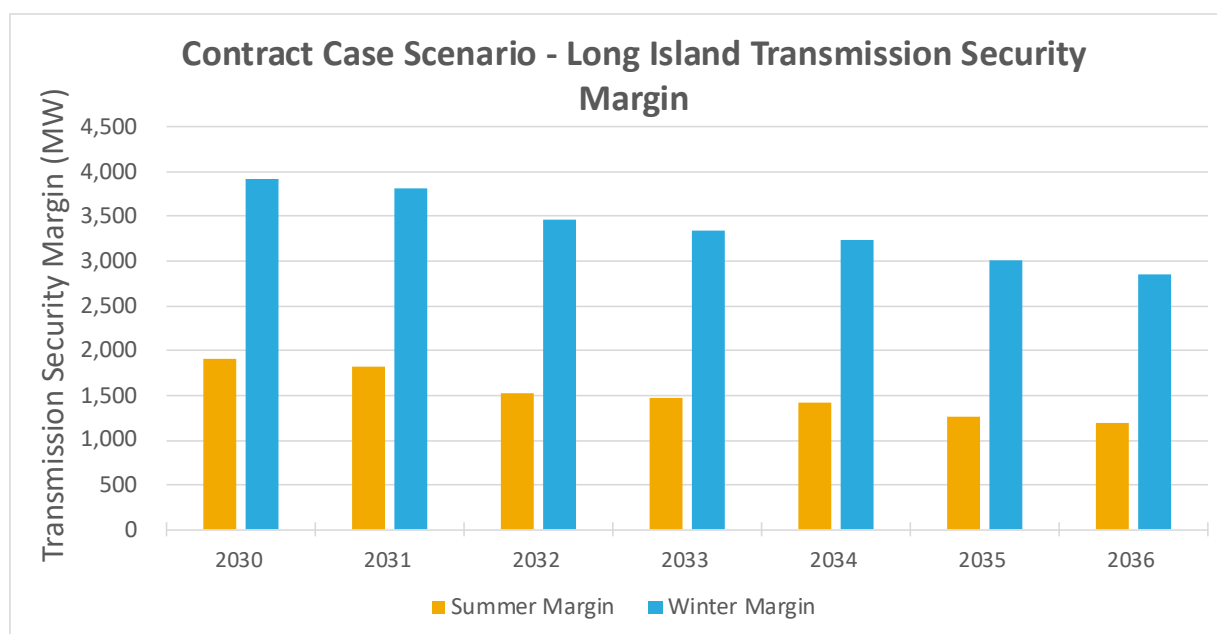
Figure 56: Contract Case - Long Island Transmission Security Margin
