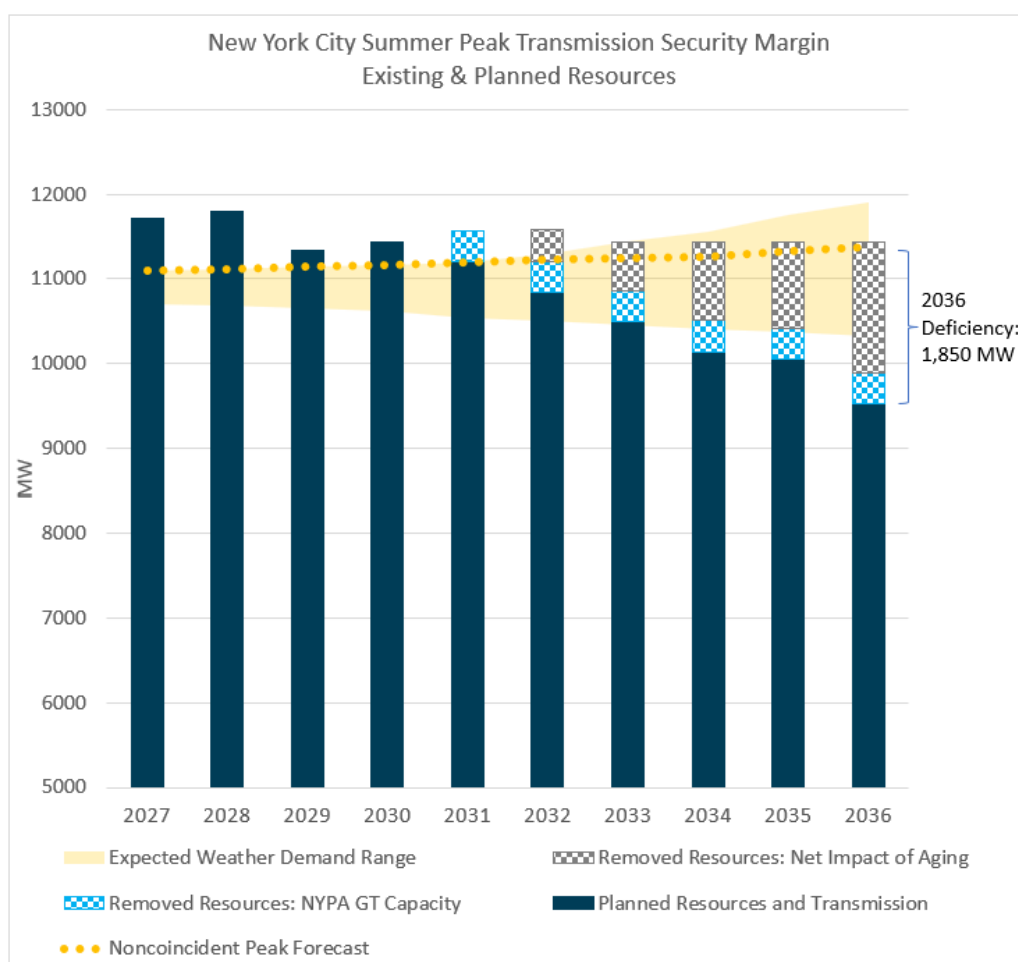
Figure 60: NYC Summer Peak Transmission Security Margin
