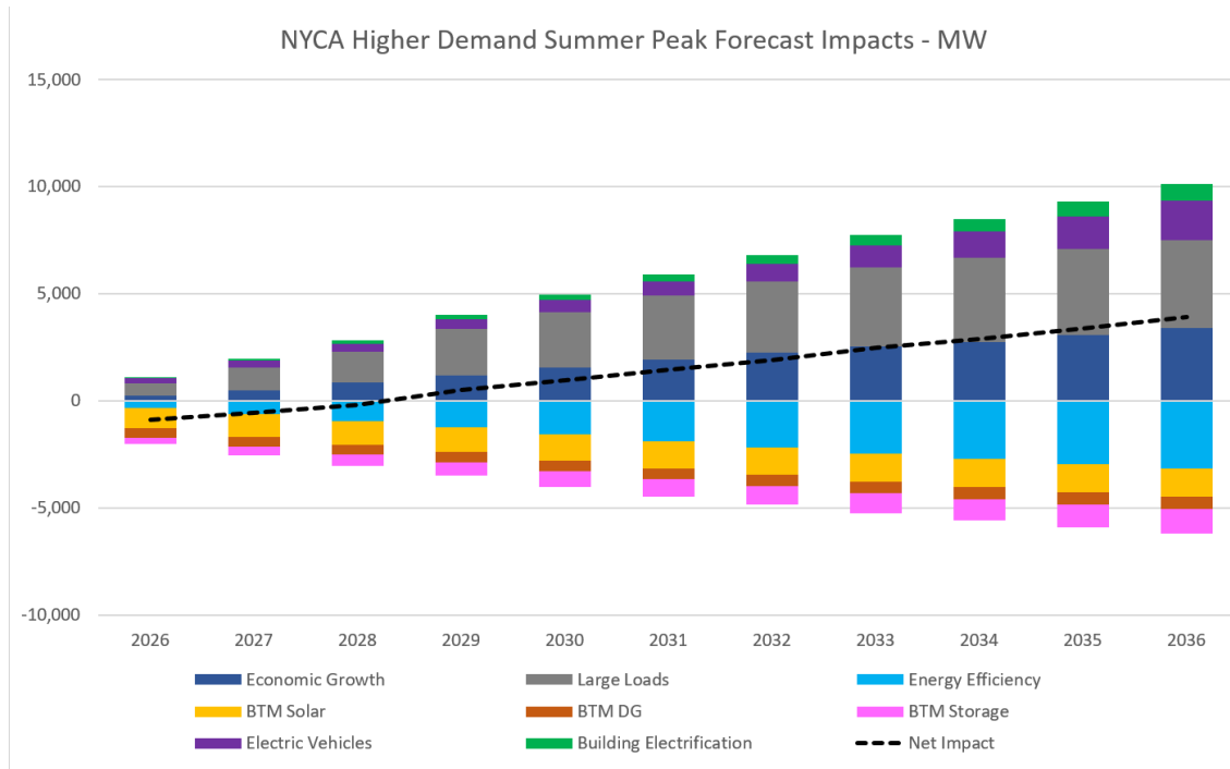
Figure 9: Higher Demand Peak Forecast Impacts
