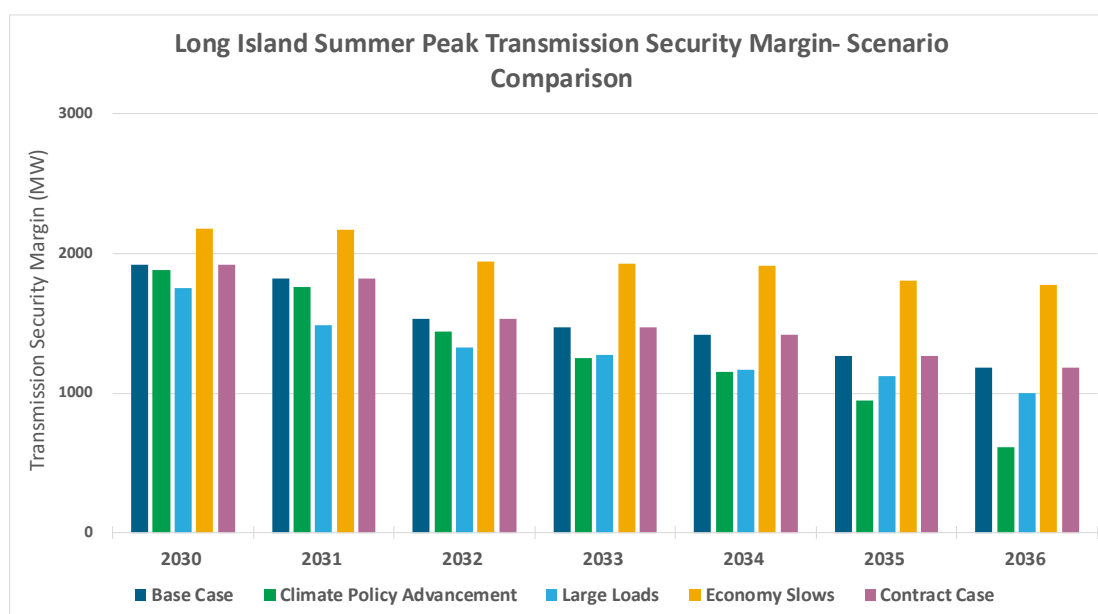
Figure 64: Scenario Summer Long Island Transmission Security Margins
