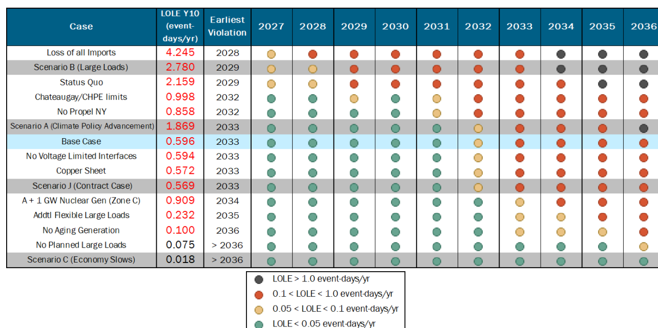
Figure 57: LOLE across the Other Informational Scenarios
