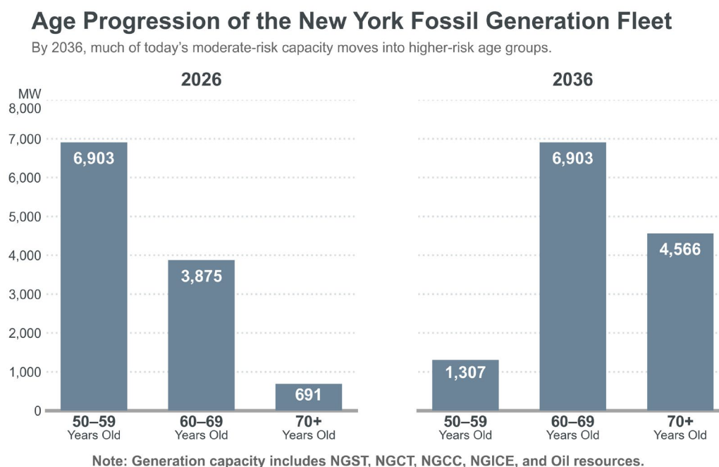
Figure 18: NY Fossil Generation Age through the RNA Horizon
