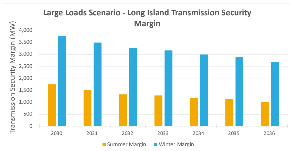
Figure 48: Large Loads Scenario - Long Island Transmission Security Margin
