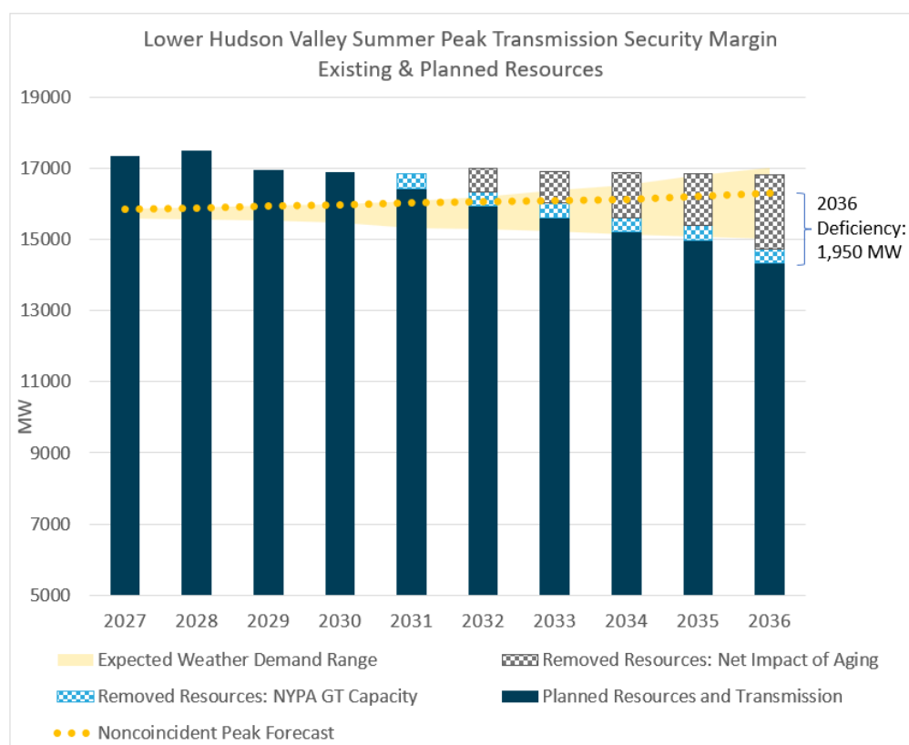
Figure 59: Lower Hudson Valley Summer Peak Transmission Security Margin
