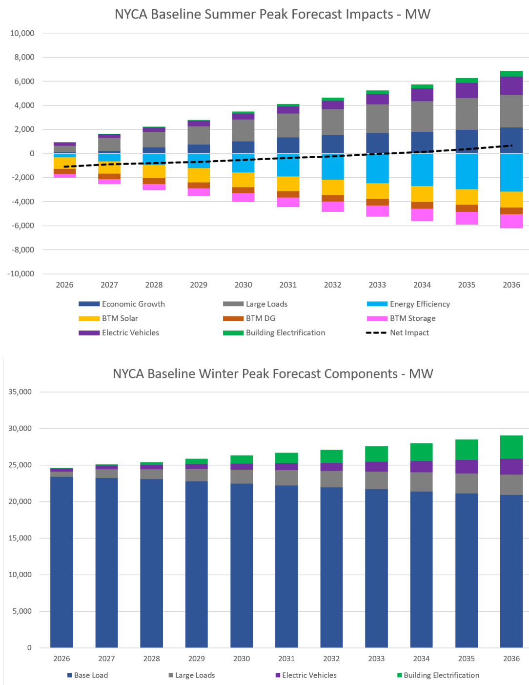
Figure 8: NYCA baseline summer and winter peak forecast impacts
