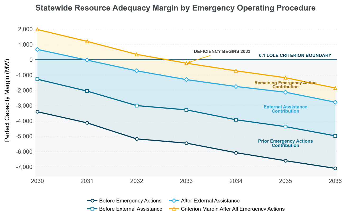
Figure 29: Statewide Resource Adequacy Margin by Emergency Operating Procedure
