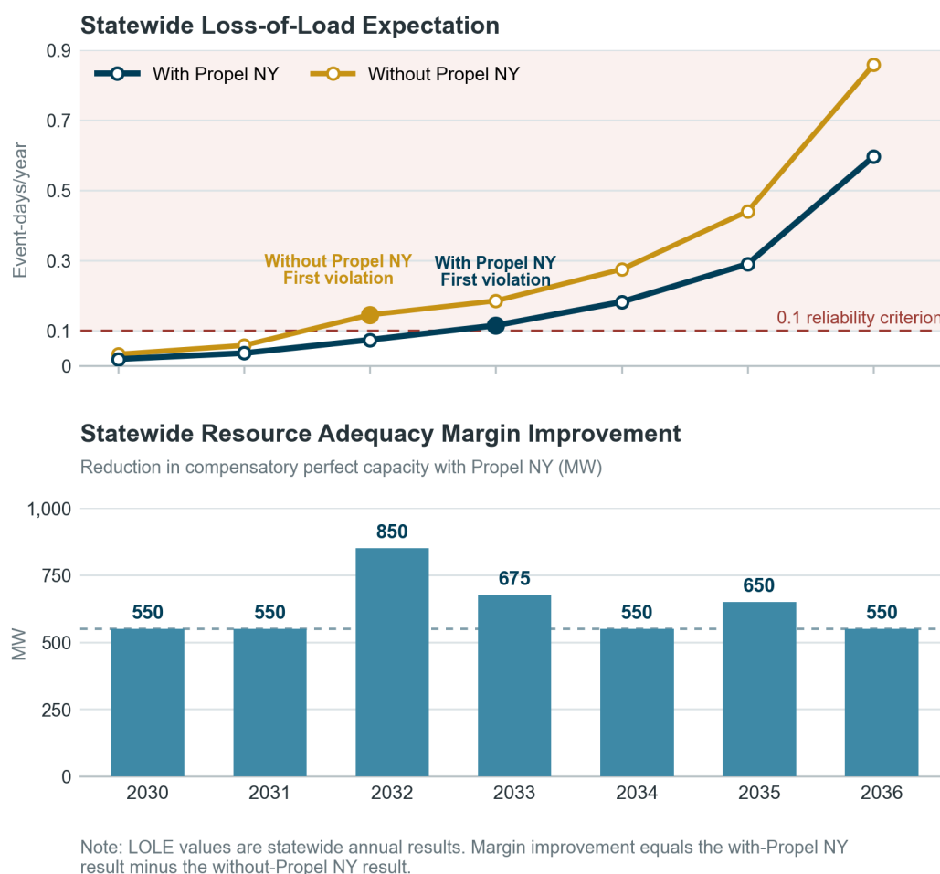
Figure 30: Resource Adequacy Impact of the Propel NY Project
