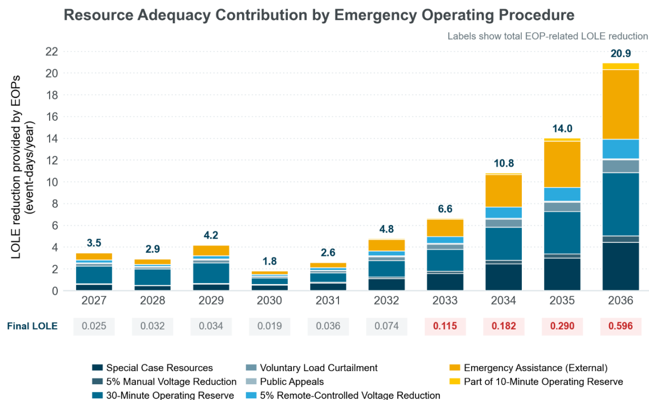
Figure 28: Resource Adequacy Contribution by Emergency Operating Procedure
