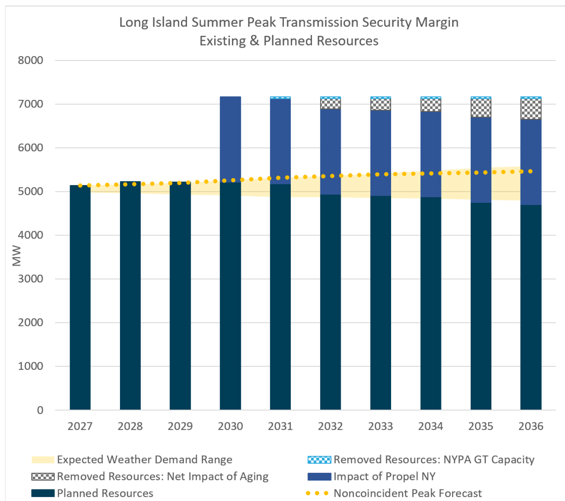
Figure 34: Long Island Summer Peak Transmission Security Margin
